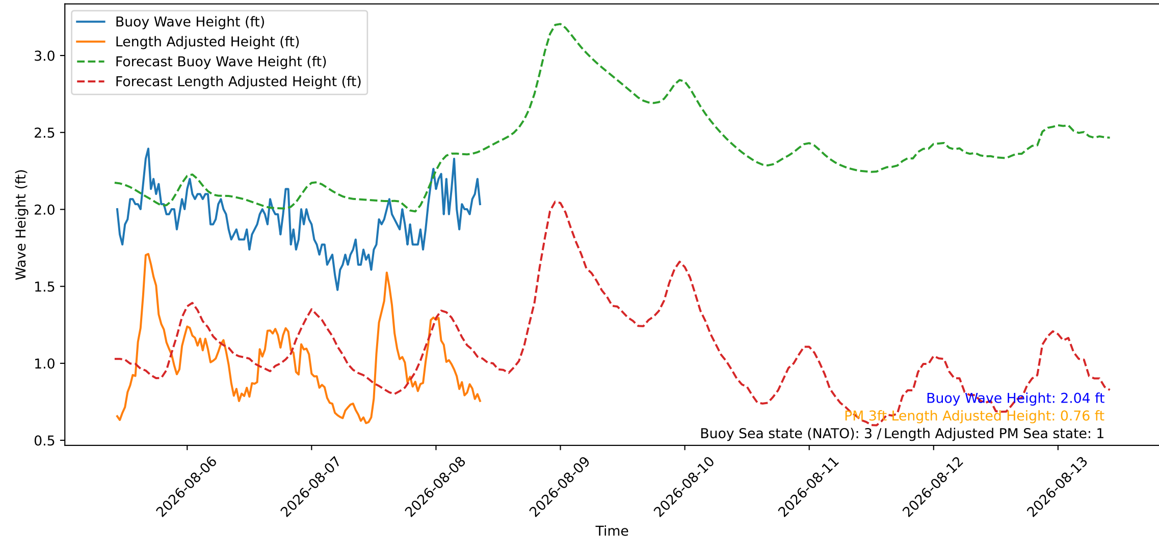
Wave Heights over Time for Red Beach at 2026-08-08 10:00:46
