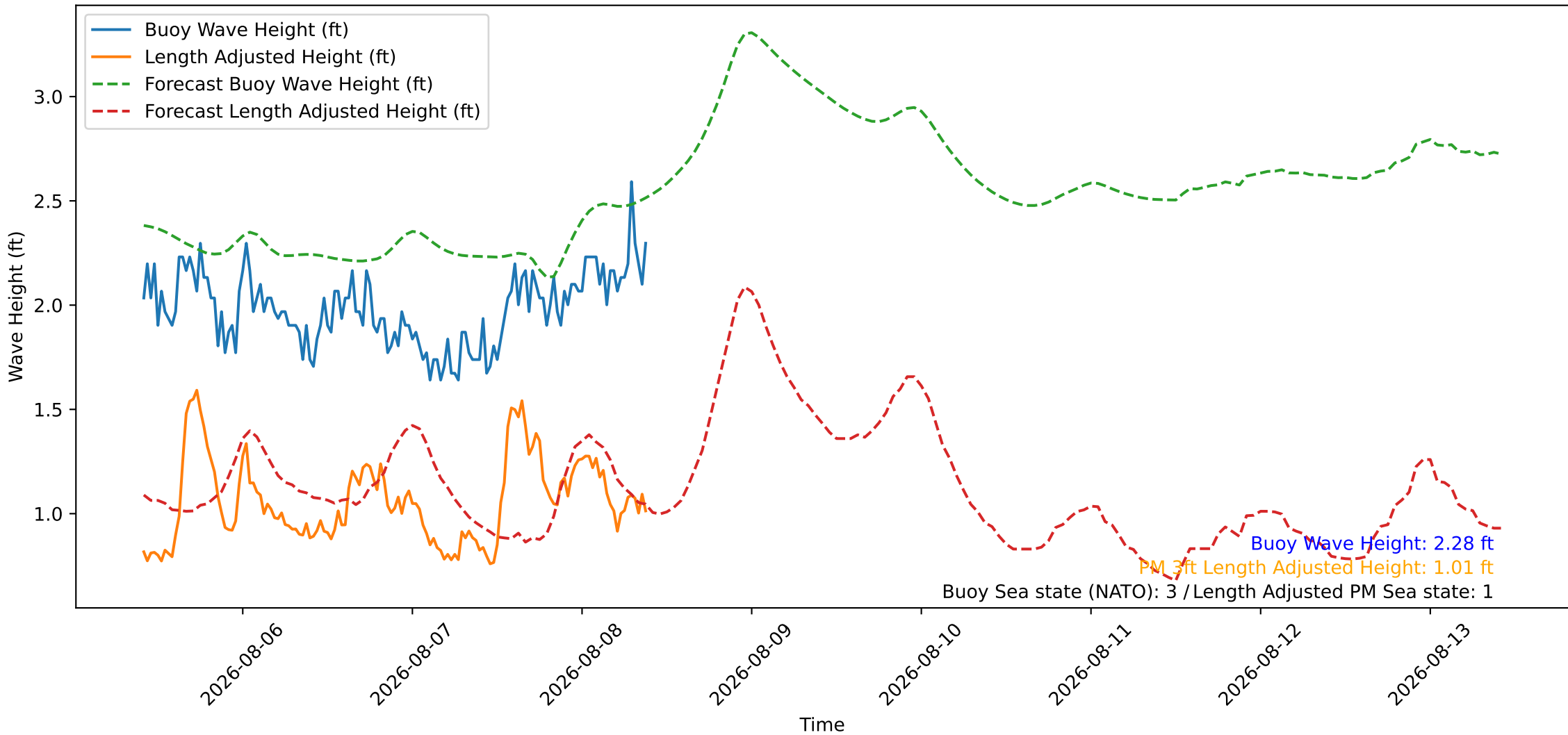
Wave Heights over Time for Oceanside Harbor at 2026-08-08 10:00:27
