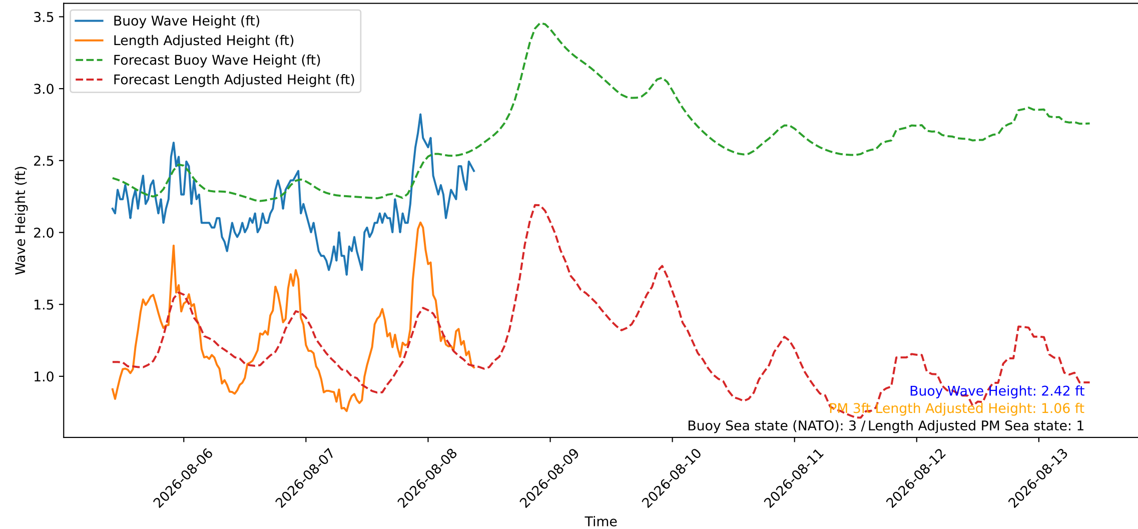
Wave Heights over Time for Green Beach at 2026-08-08 10:01:08
