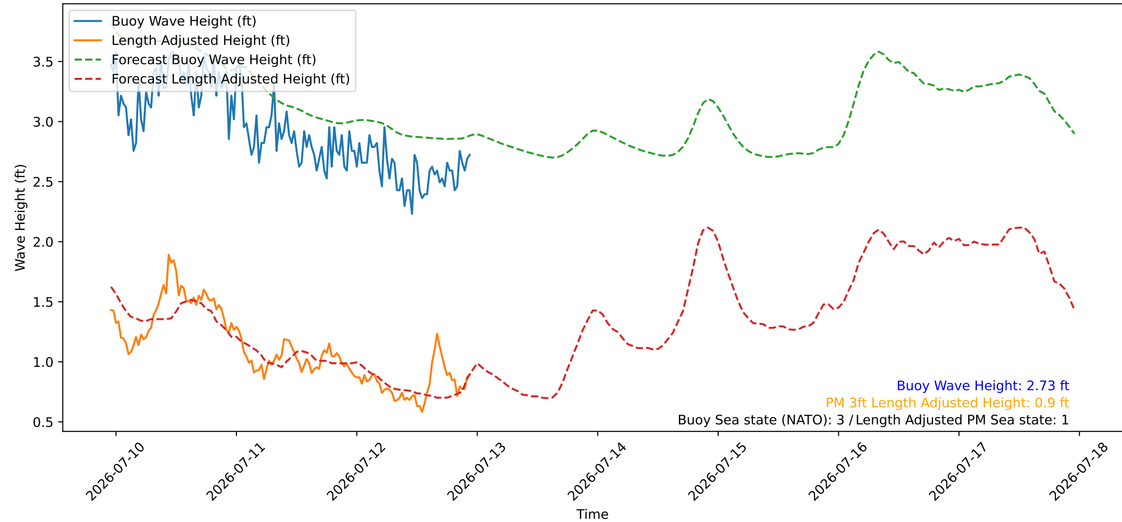
Wave Heights over Time for Green Beach at 2026-07-12 23:11:09
