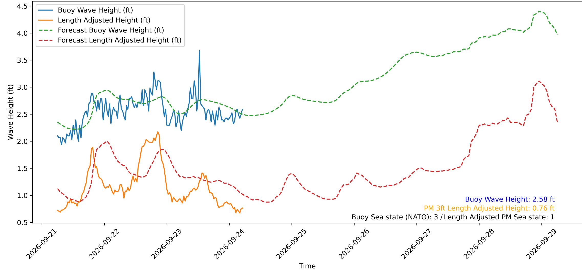
Wave Heights over Time for Red Beach at 2026-09-24 05:40:49
