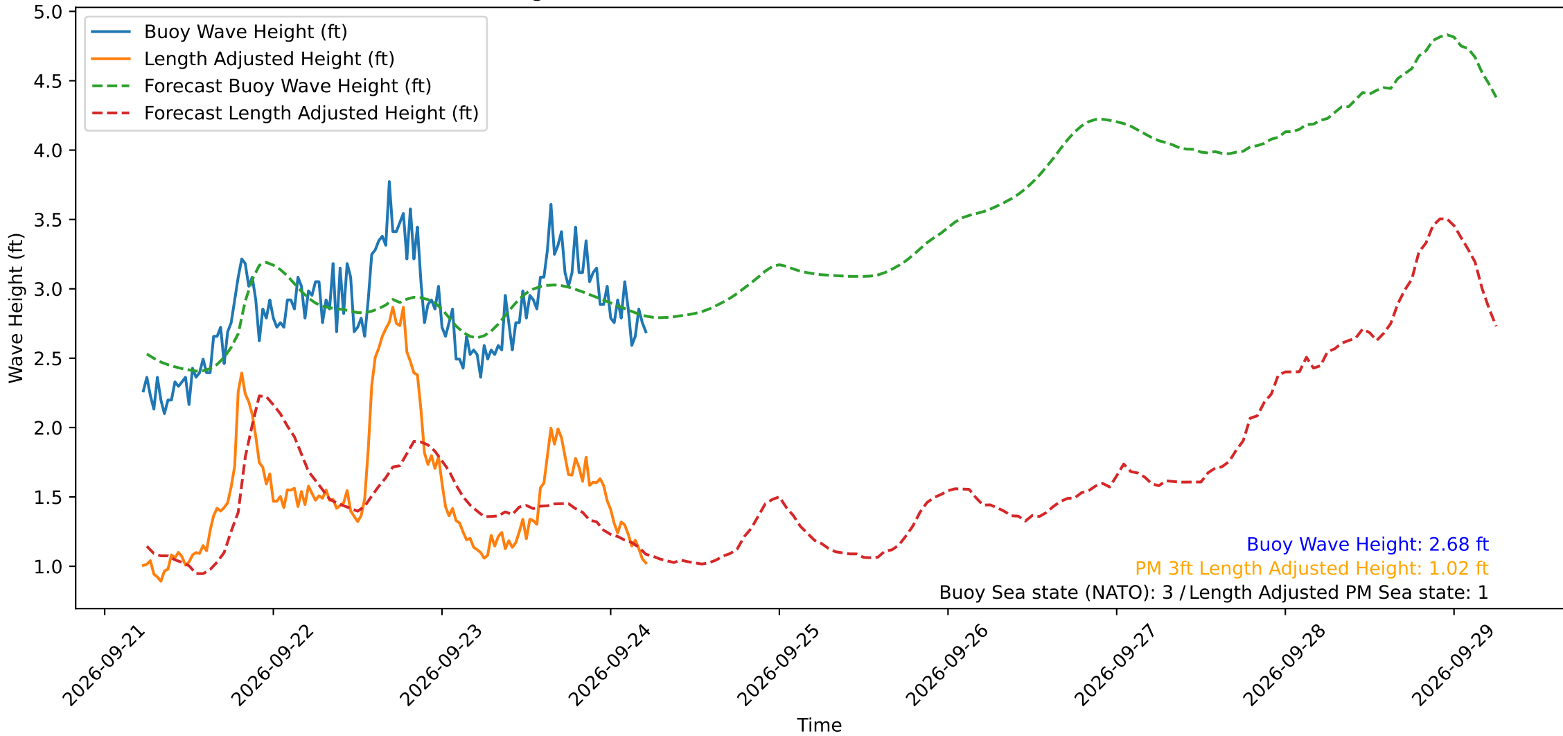
Wave Heights over Time for Oceanside Harbor at 2026-09-24 05:40:29
