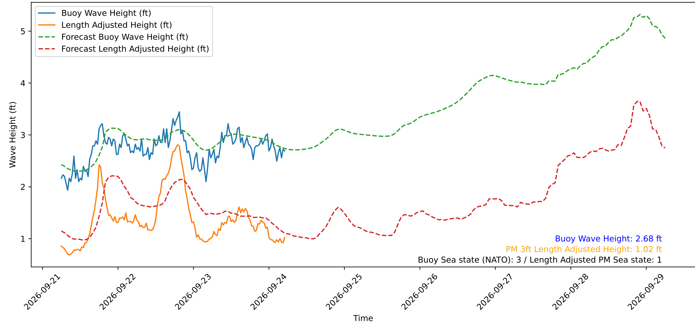
Wave Heights over Time for Green Beach at 2026-09-24 05:41:11
