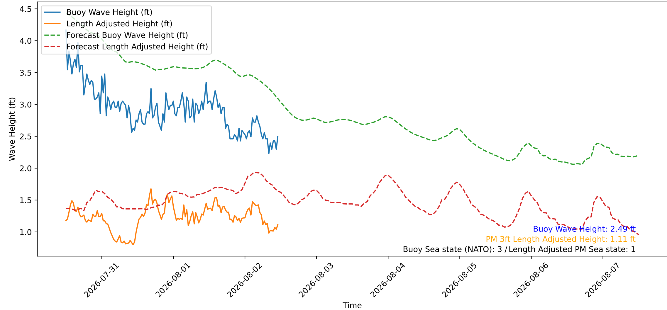
Wave Heights over Time for Red Beach at 2026-08-02 11:50:46
