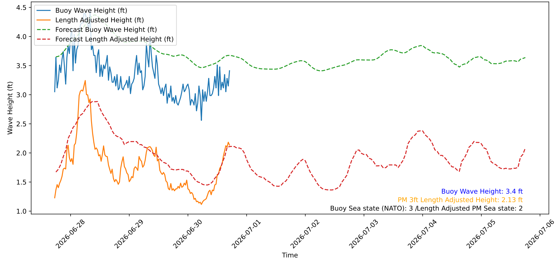
Wave Heights over Time for Oceanside Harbor at 2026-06-30 17:40:26
