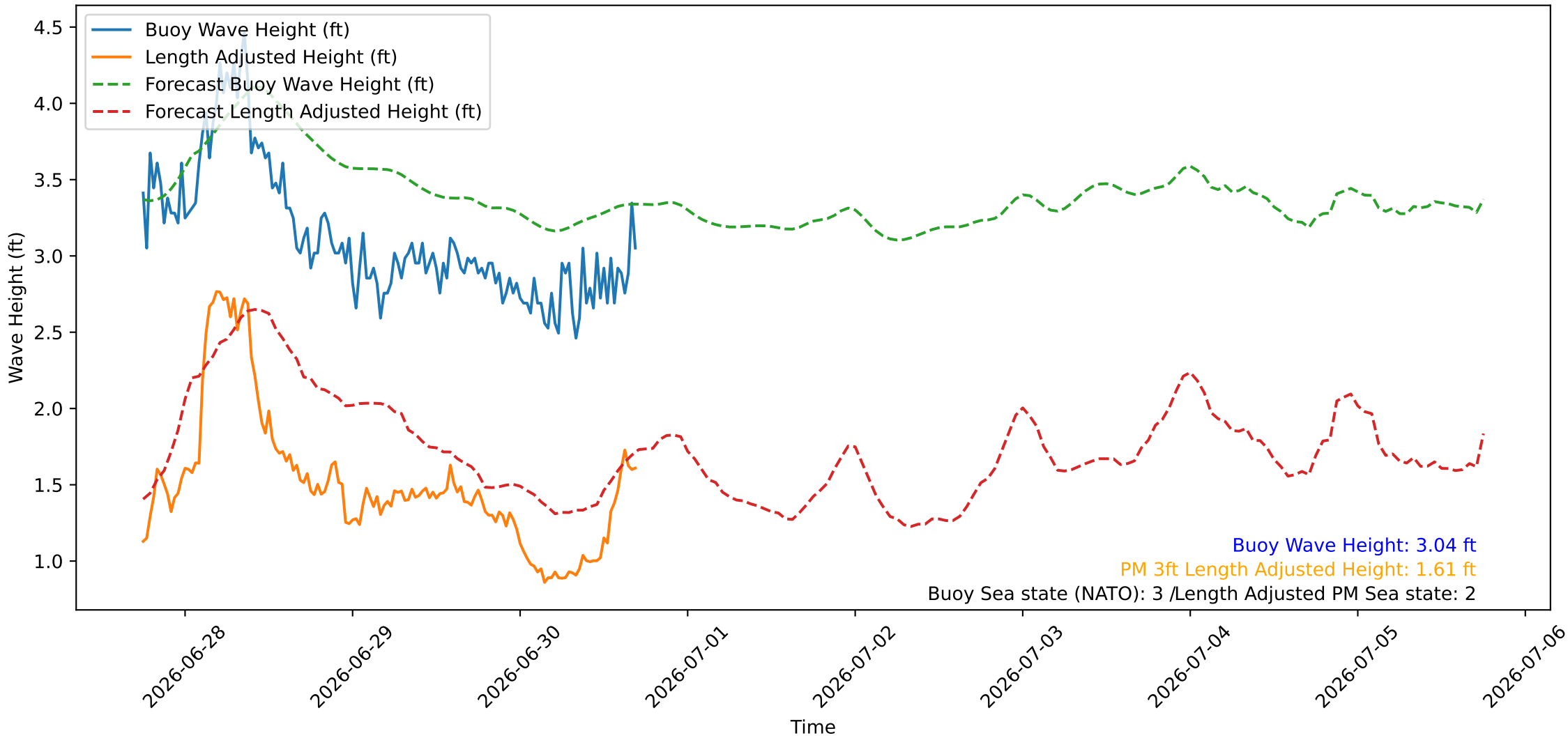
Wave Heights over Time for Red Beach at 2026-06-30 17:40:45
