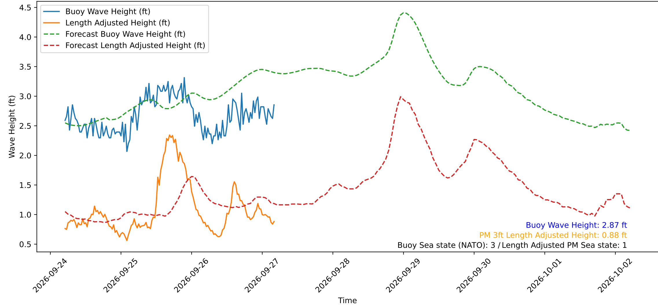
Wave Heights over Time for Red Beach at 2026-09-27 04:40:49
