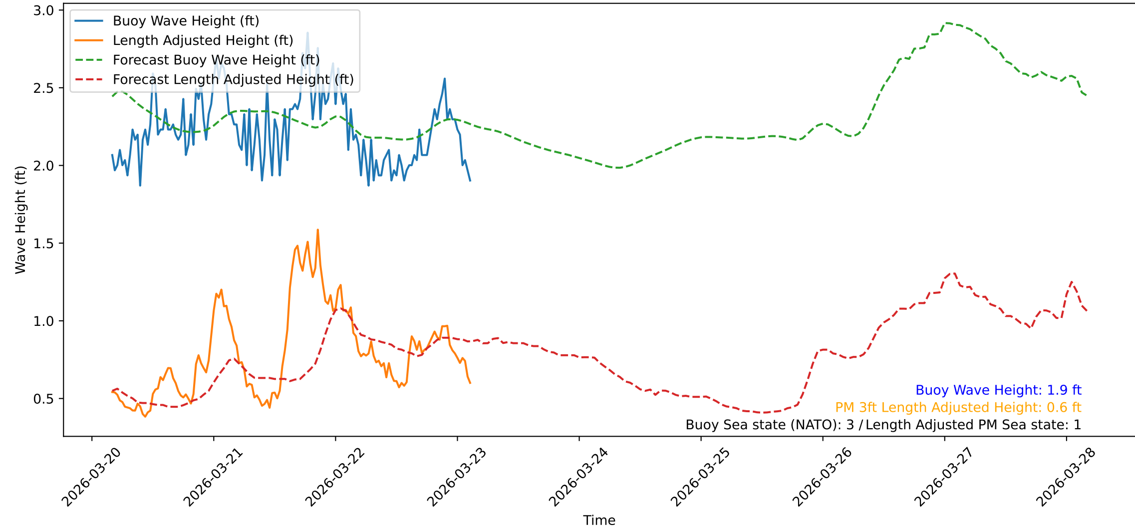
Wave Heights over Time for Red Beach at 2026-03-23 03:30:47
