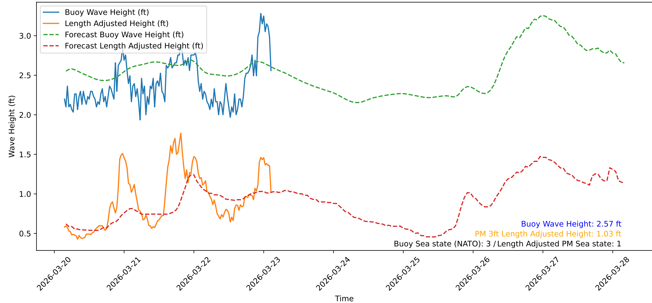
Wave Heights over Time for Green Beach at 2026-03-23 03:31:09
