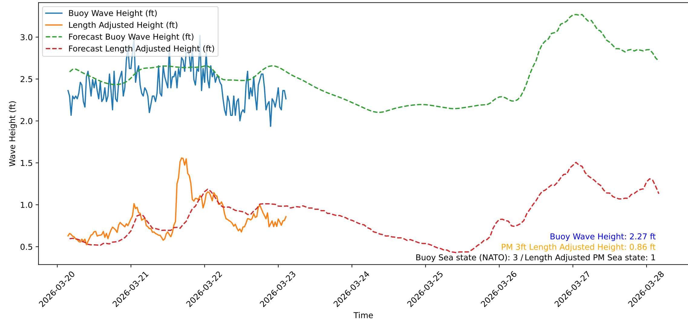
Wave Heights over Time for Oceanside Harbor at 2026-03-23 03:30:31
