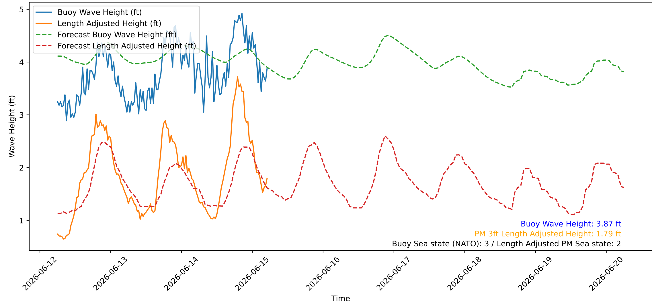
Wave Heights over Time for Green Beach at 2026-06-15 05:51:09
