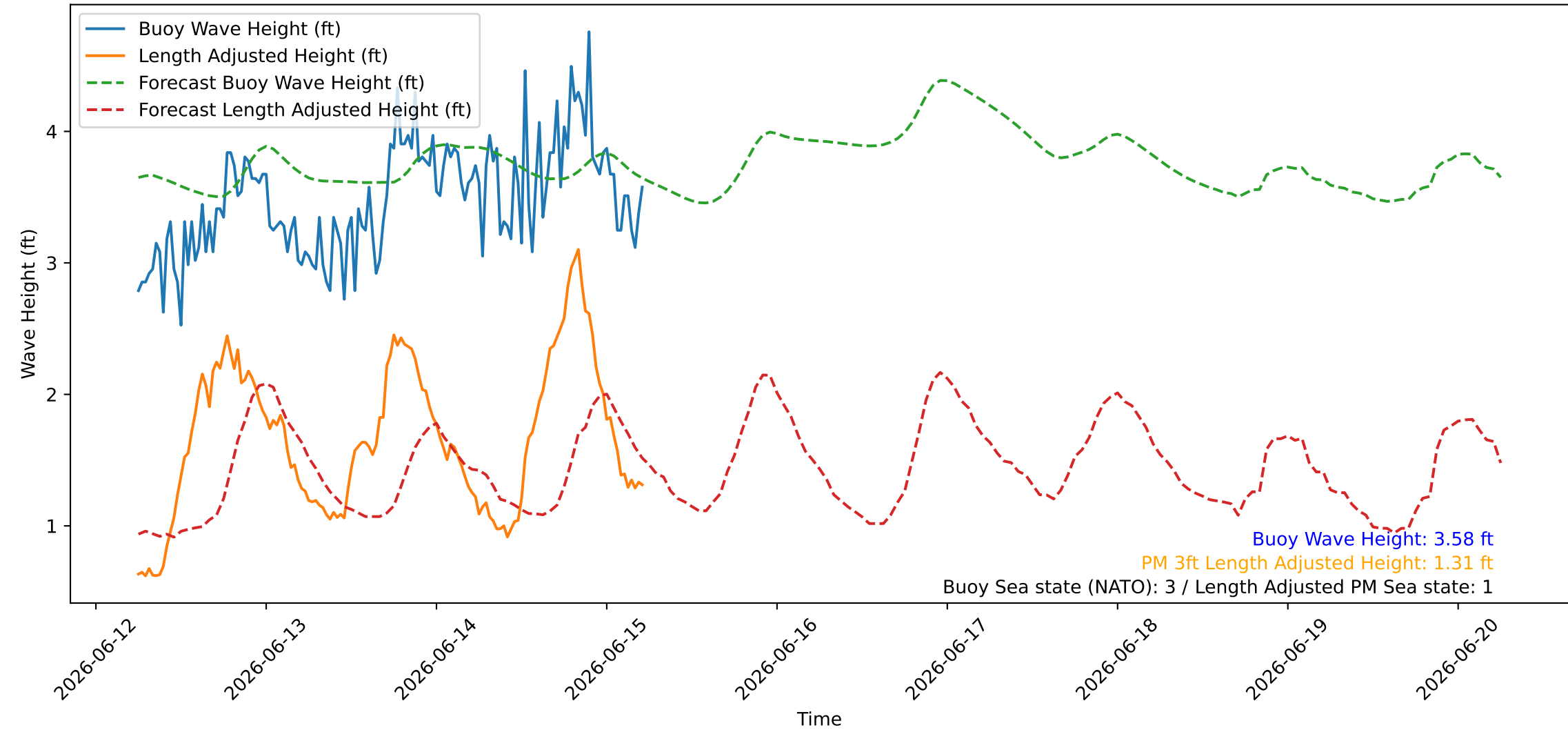
Wave Heights over Time for Red Beach at 2026-06-15 05:50:46
