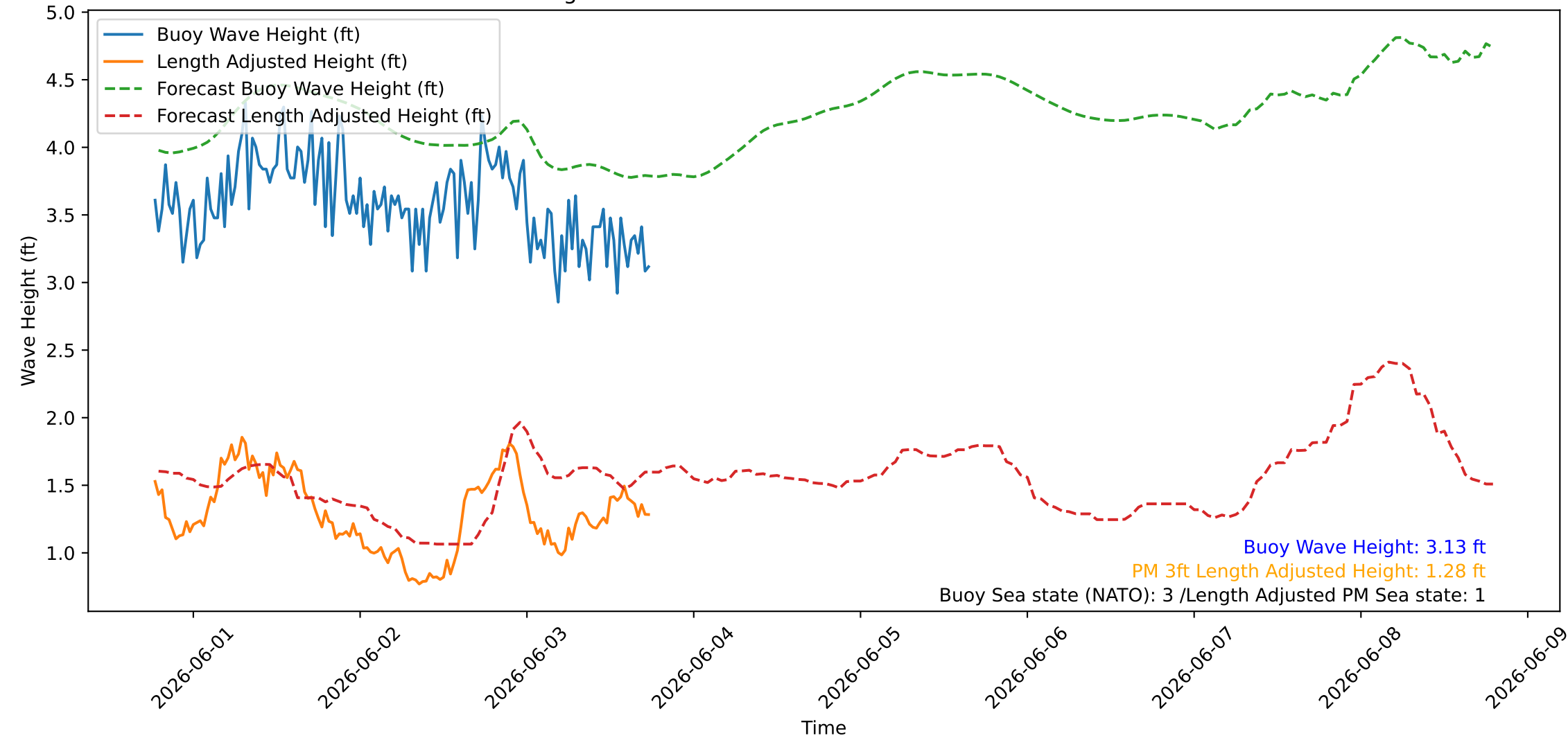
Wave Heights over Time for Green Beach at 2026-06-03 18:31:07
