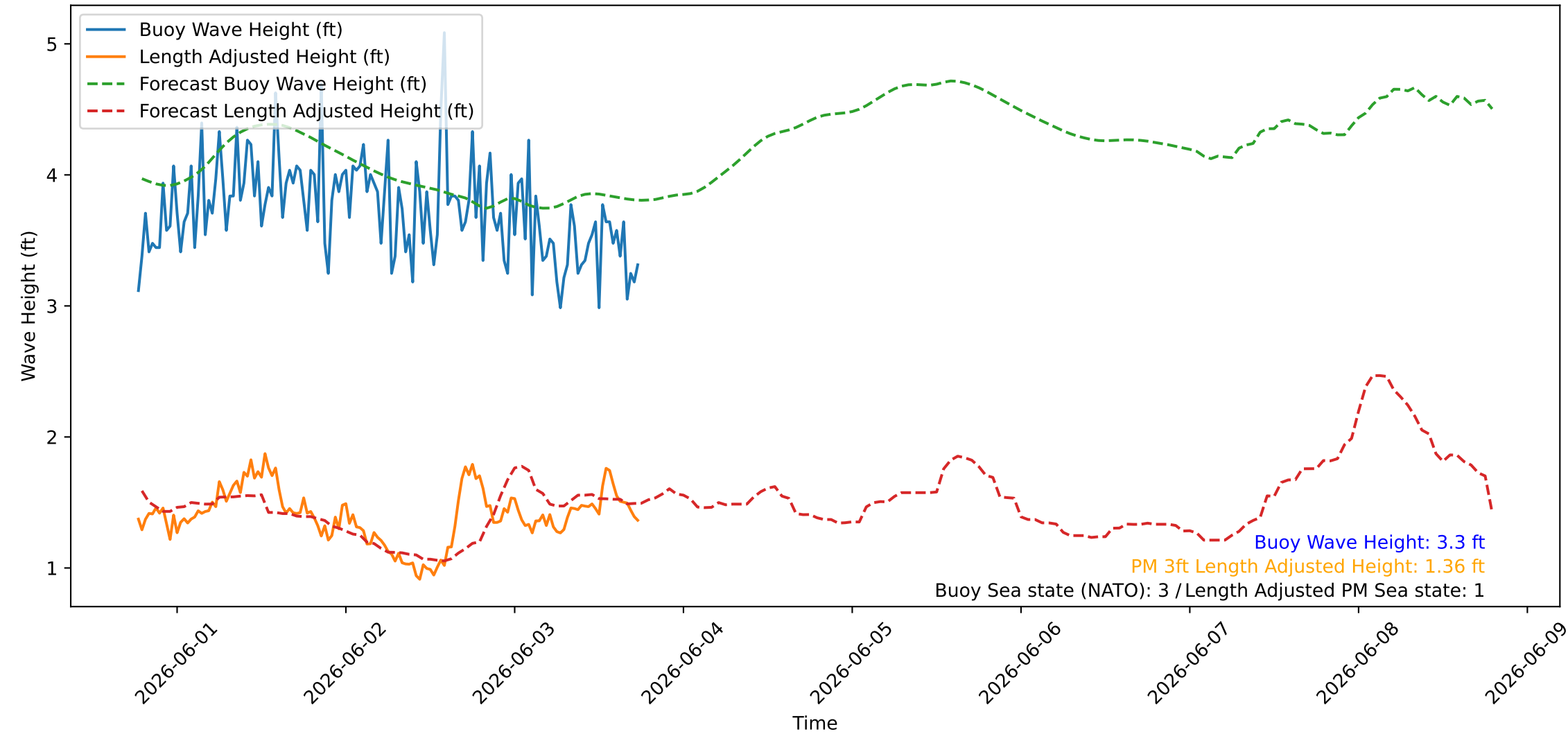
Wave Heights over Time for Oceanside Harbor at 2026-06-03 18:30:26
