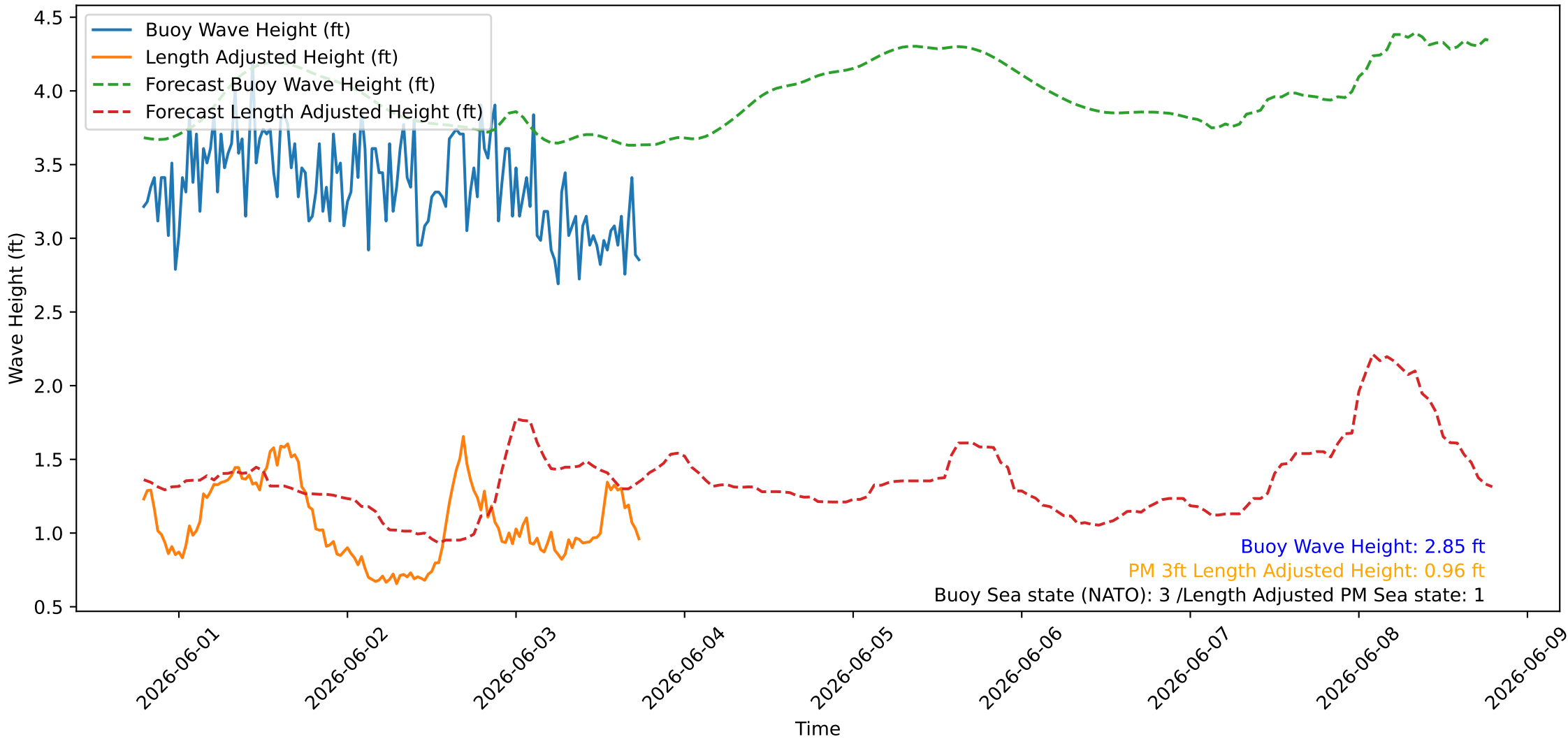
Wave Heights over Time for Red Beach at 2026-06-03 18:30:45
