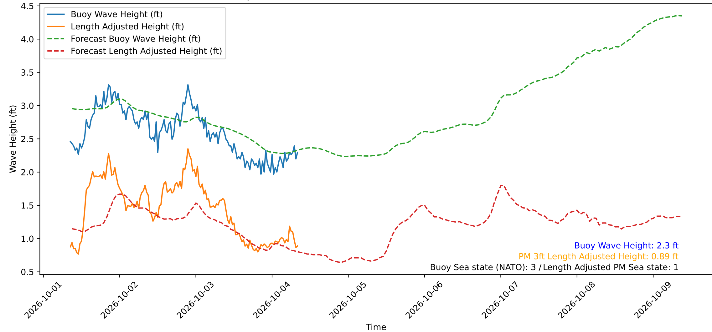
Wave Heights over Time for Oceanside Harbor at 2026-10-04 08:40:30
