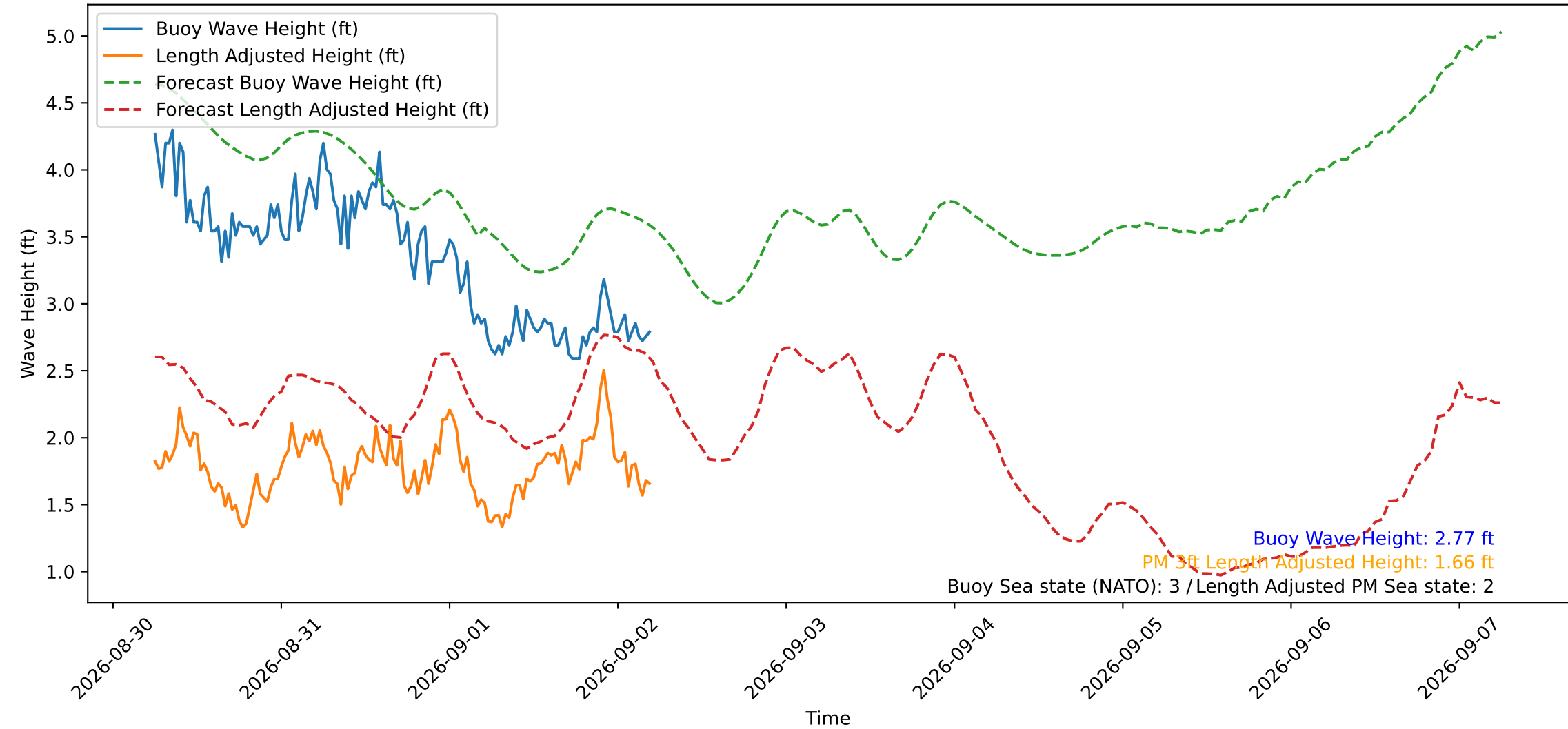
Wave Heights over Time for Red Beach at 2026-09-02 05:30:49
