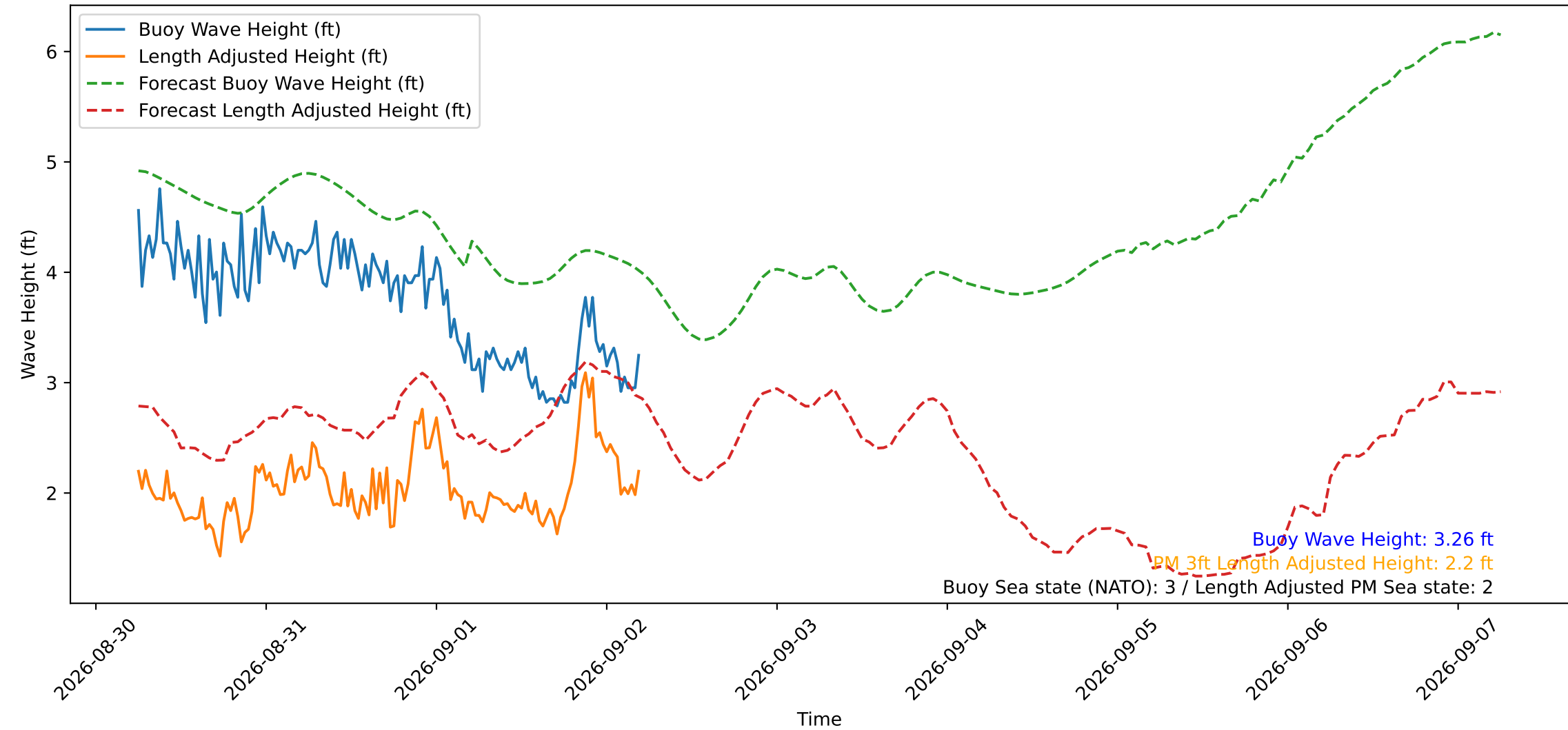
Wave Heights over Time for Green Beach at 2026-09-02 05:31:12
