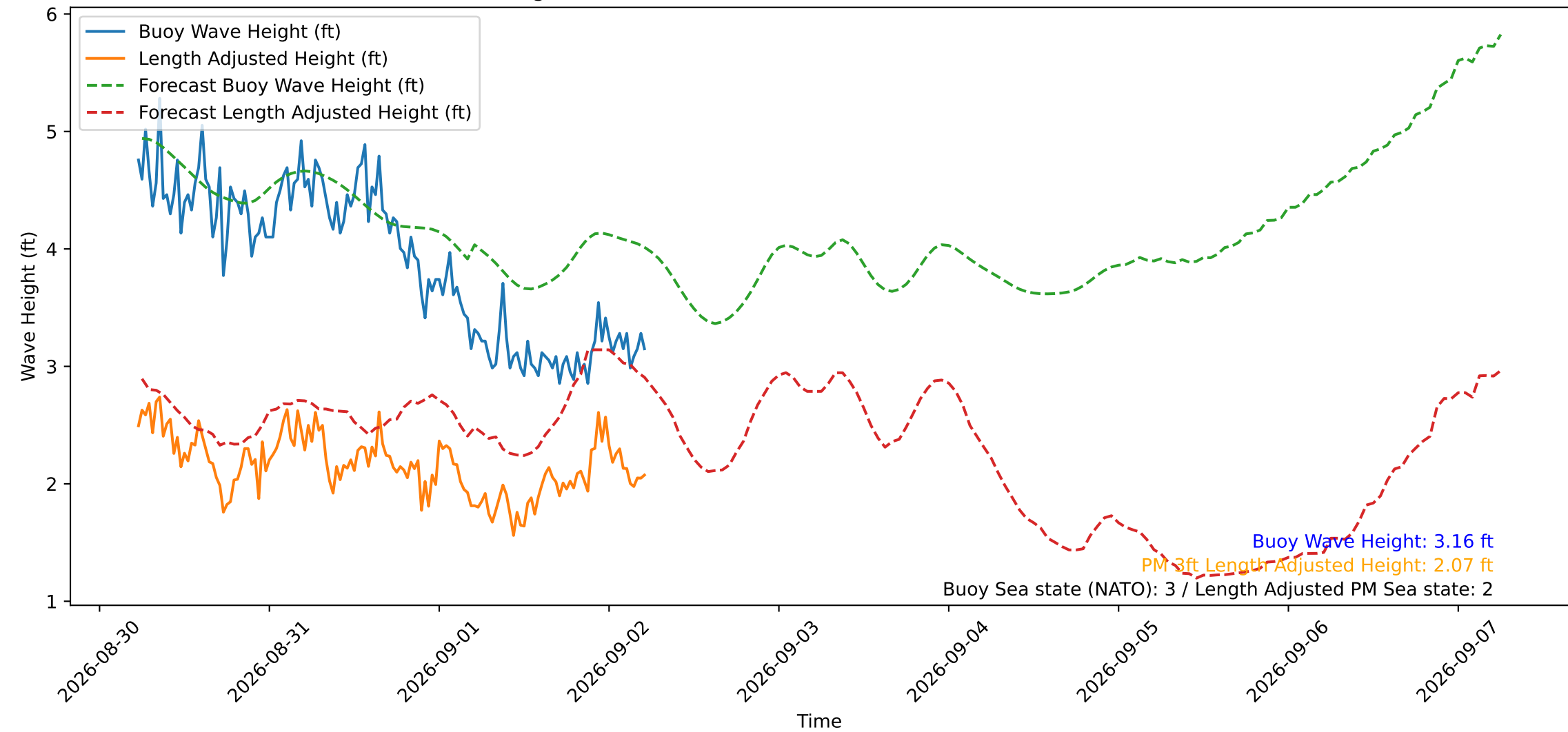
Wave Heights over Time for Oceanside Harbor at 2026-09-02 05:30:29
