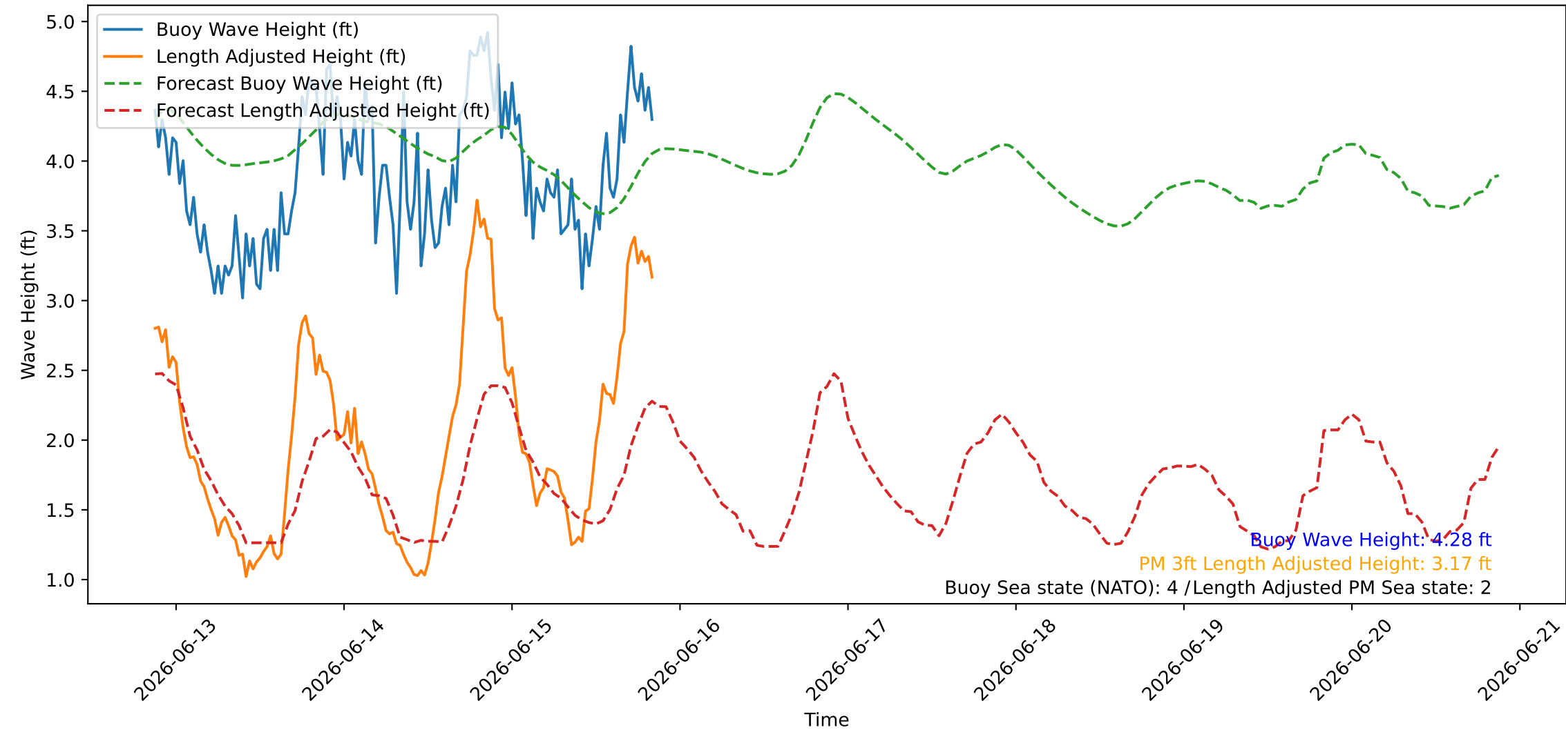
Wave Heights over Time for Green Beach at 2026-06-15 20:51:09
