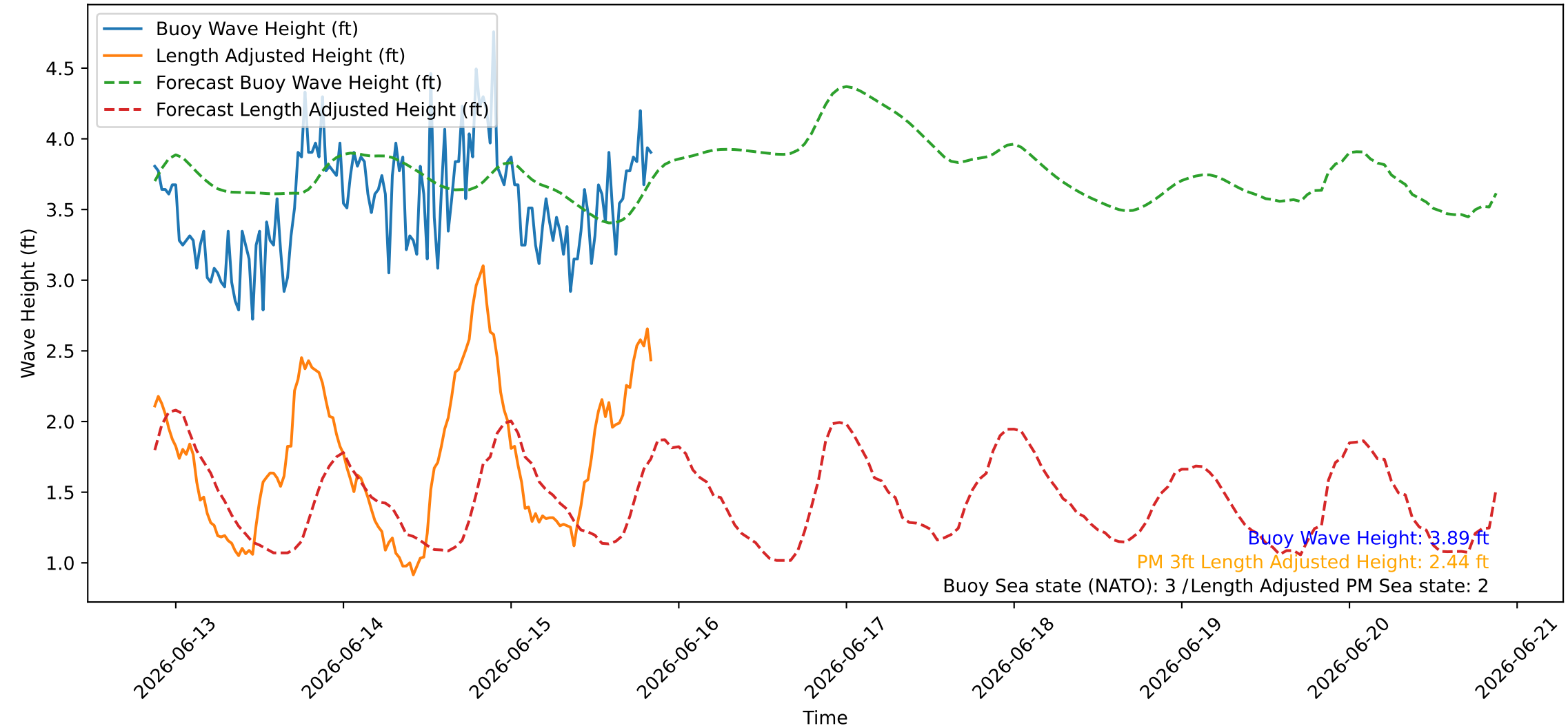
Wave Heights over Time for Red Beach at 2026-06-15 20:50:46
