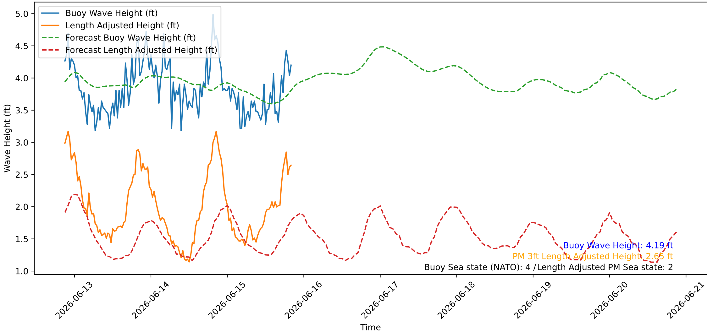
Wave Heights over Time for Oceanside Harbor at 2026-06-15 20:50:26
