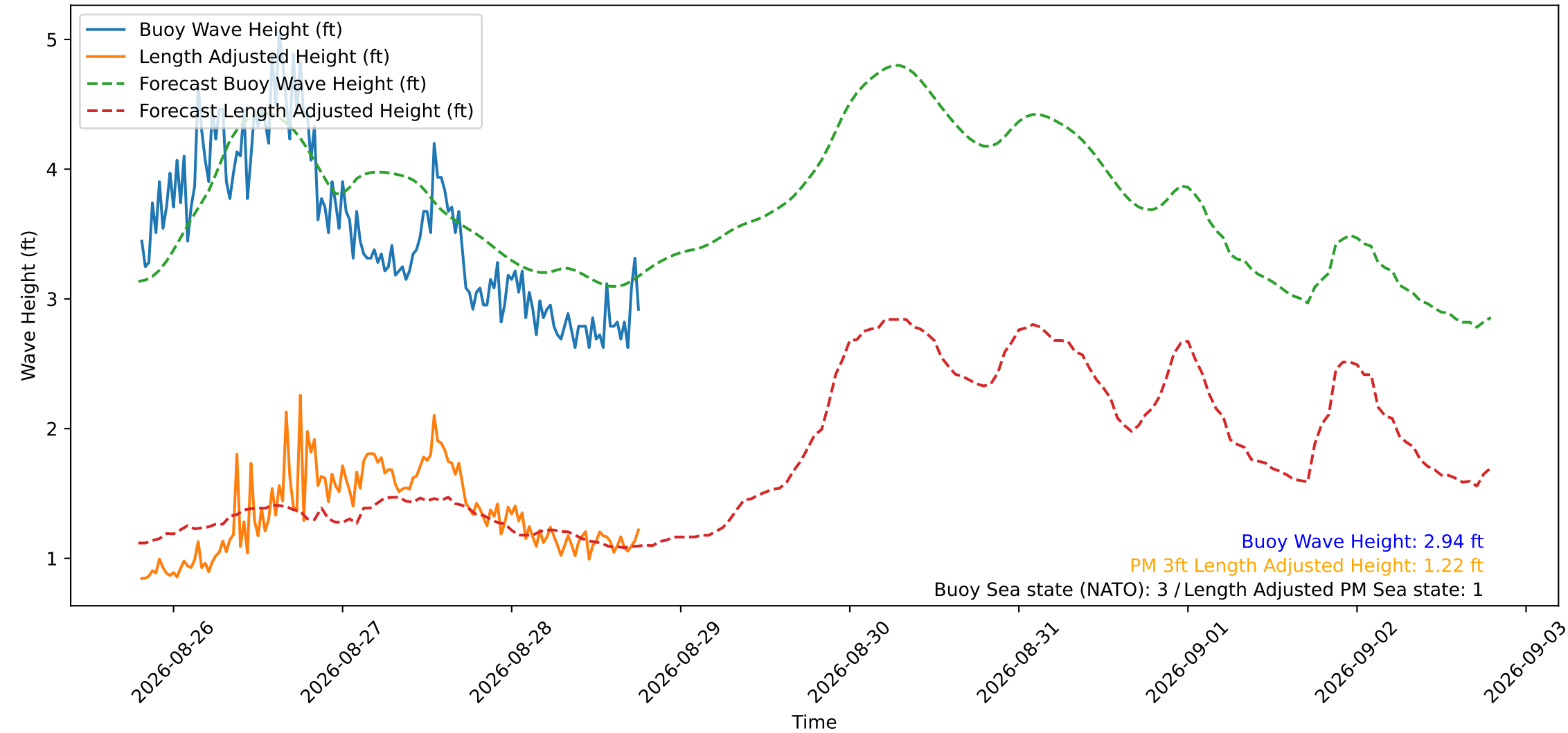
Wave Heights over Time for Red Beach at 2026-08-28 19:00:48
