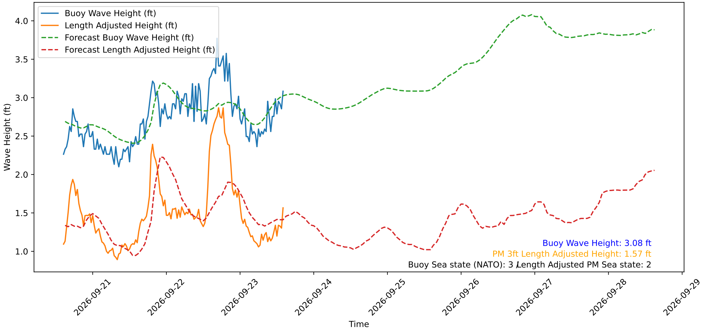
Wave Heights over Time for Oceanside Harbor at 2026-09-23 14:40:29
