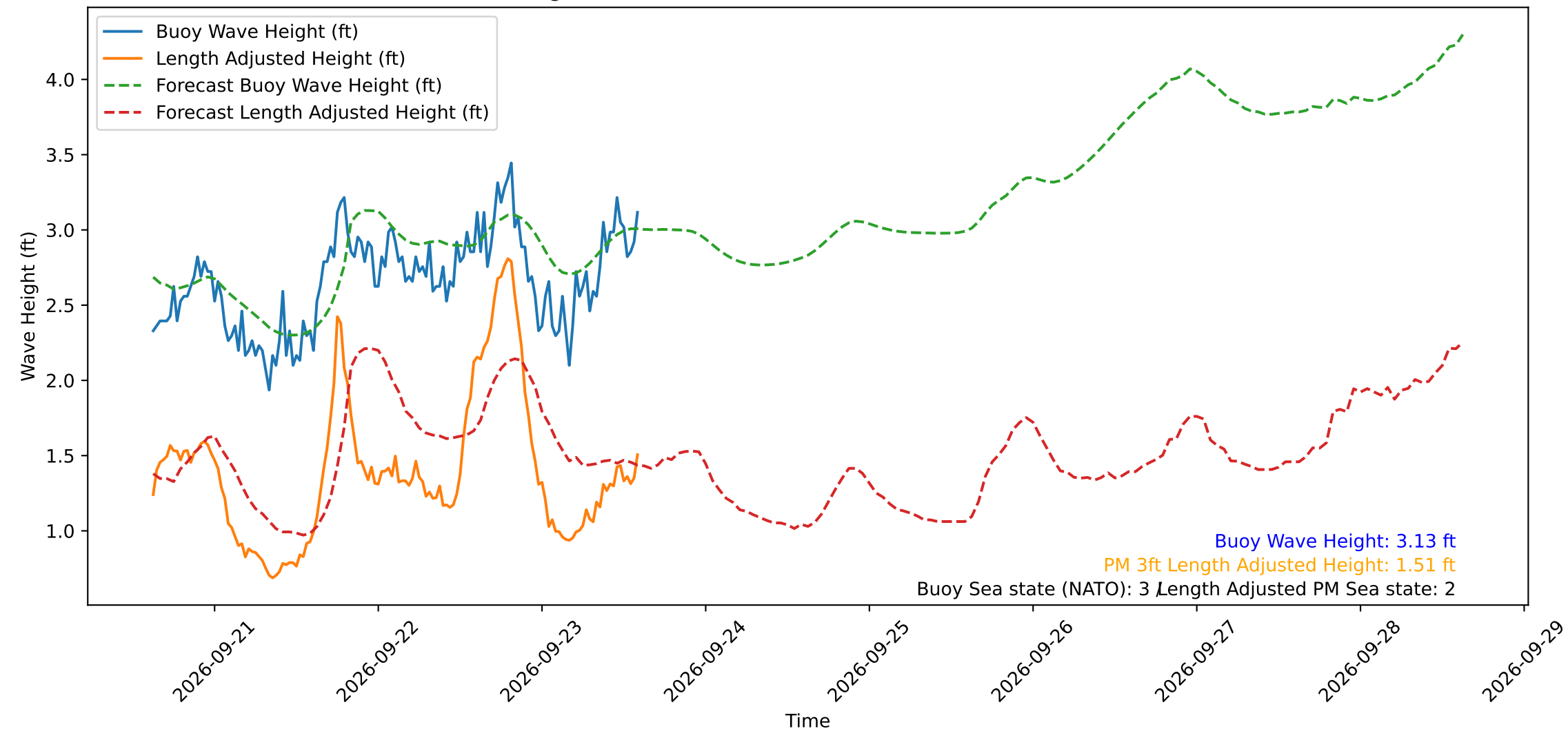
Wave Heights over Time for Green Beach at 2026-09-23 14:41:12
