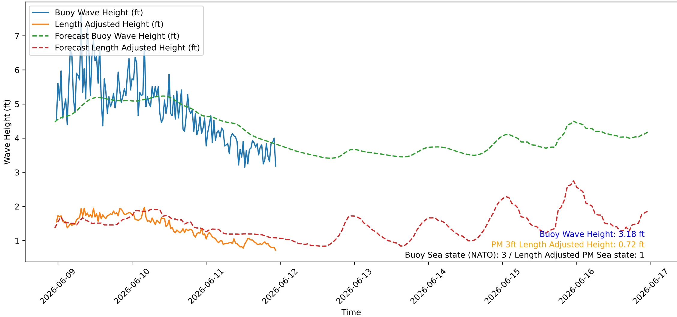
Wave Heights over Time for Red Beach at 2026-06-11 23:10:46
