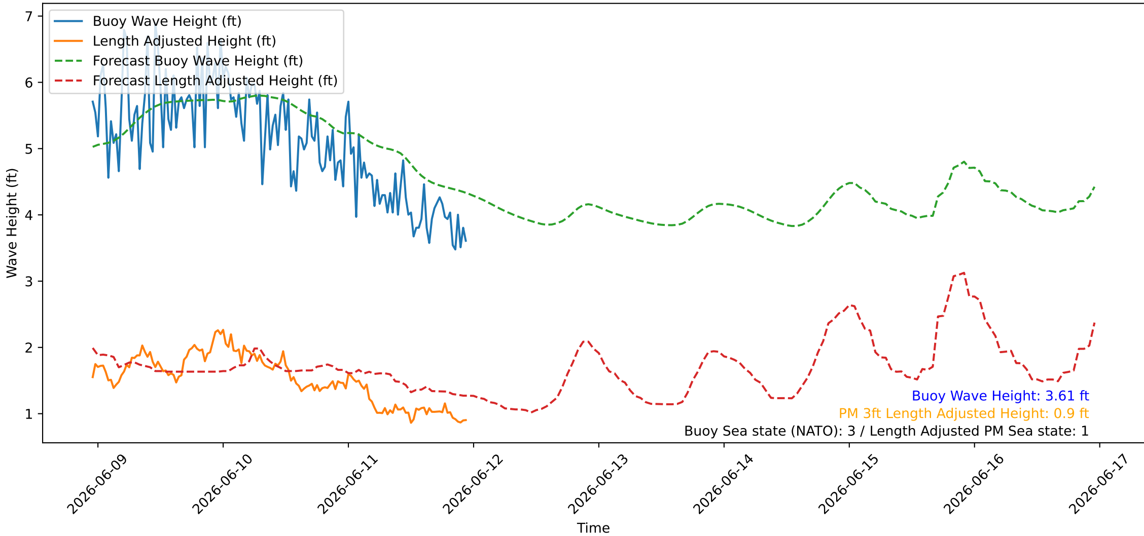
Wave Heights over Time for Green Beach at 2026-06-11 23:11:08
