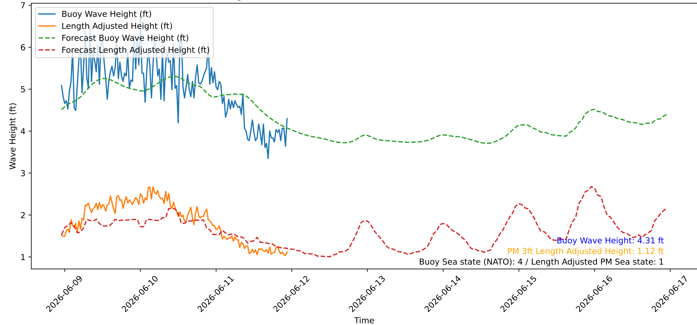
Wave Heights over Time for Oceanside Harbor at 2026-06-11 23:10:26
