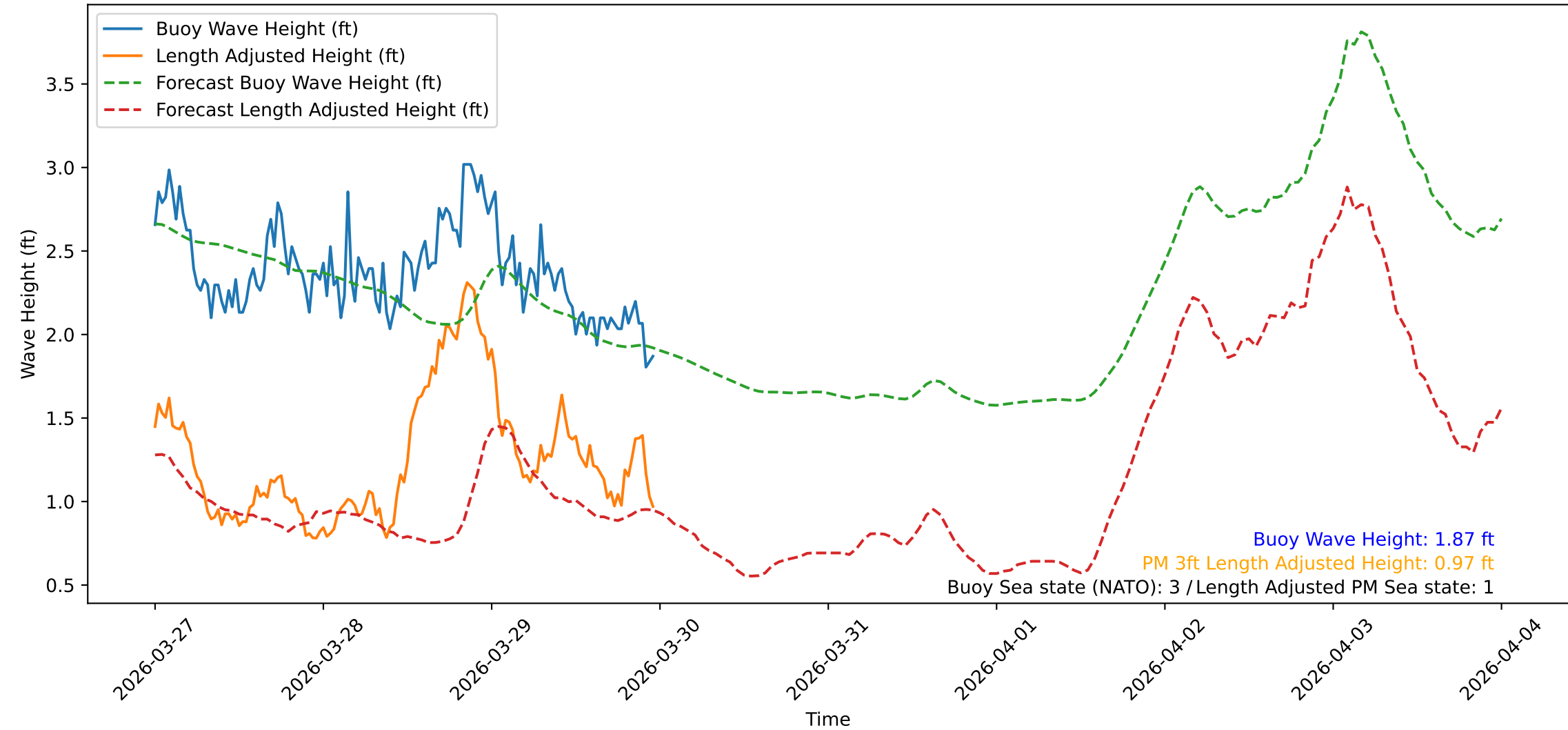
Wave Heights over Time for Red Beach at 2026-03-29 23:40:47
