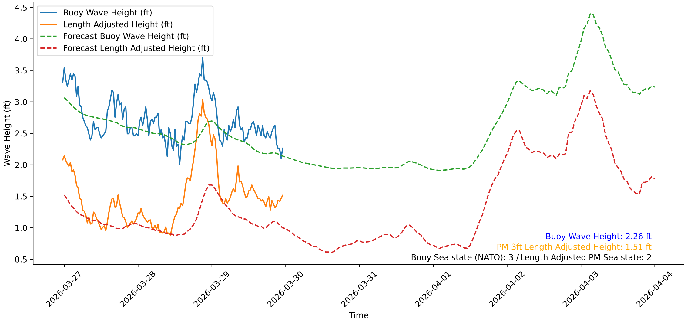
Wave Heights over Time for Green Beach at 2026-03-29 23:41:10
