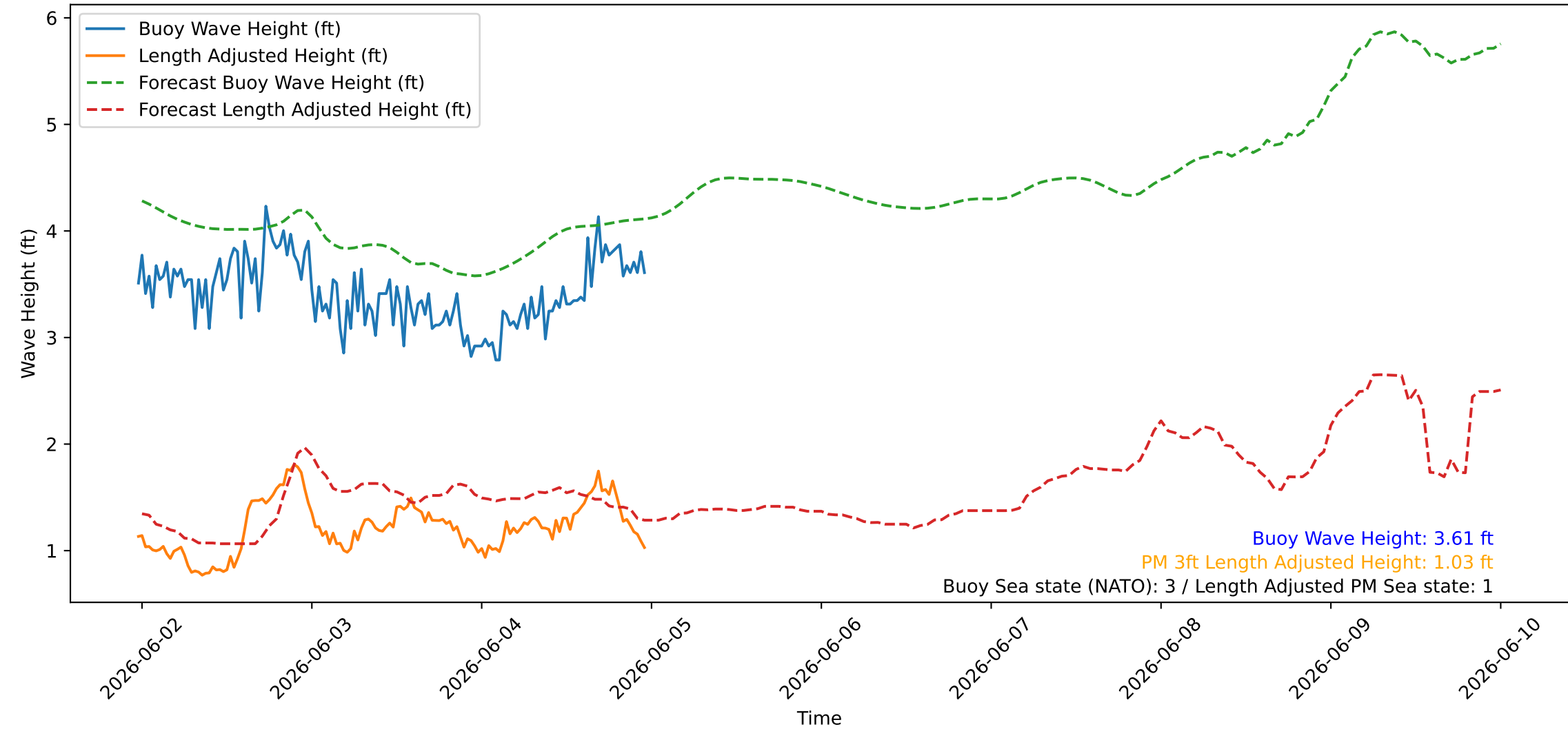
Wave Heights over Time for Green Beach at 2026-06-04 23:41:09
