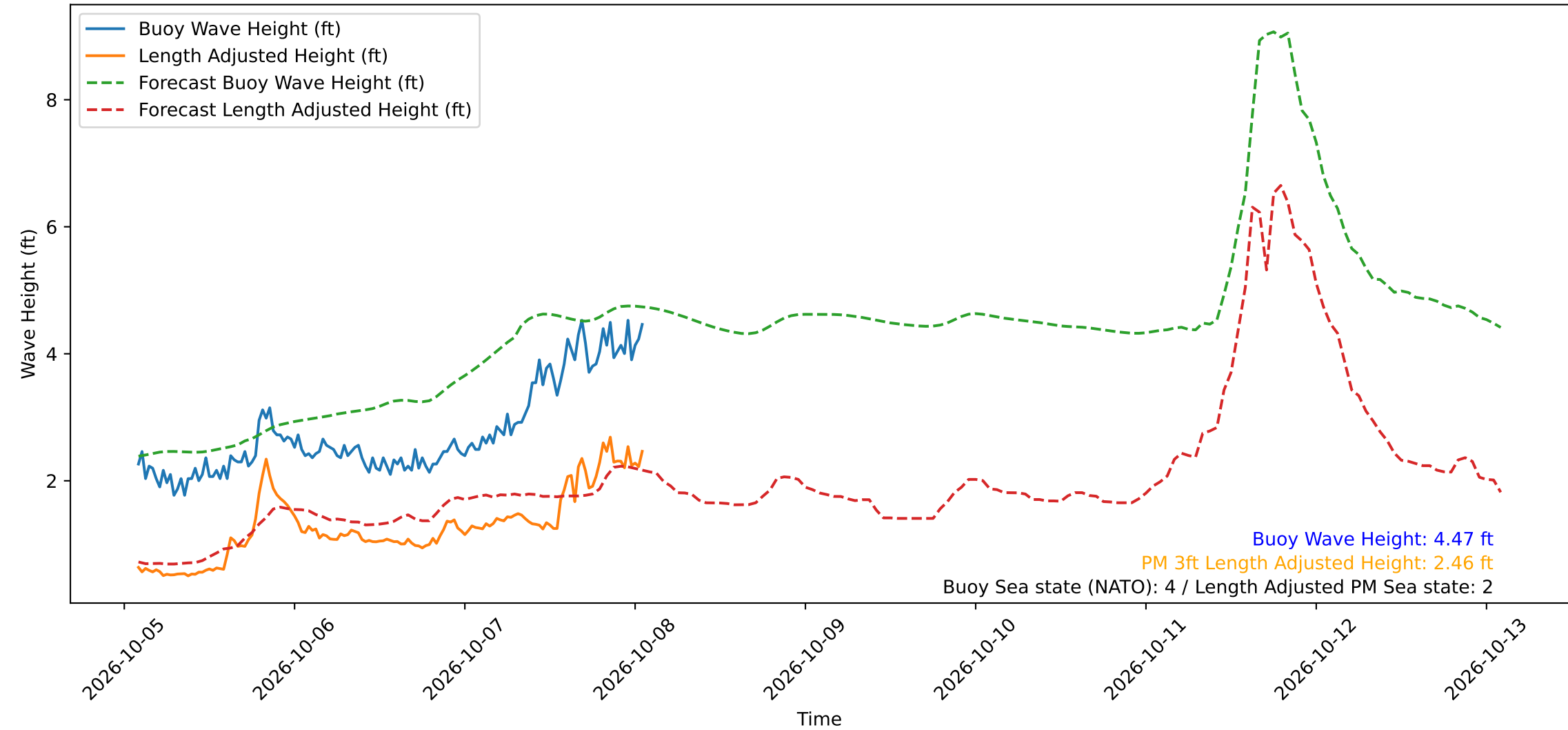
Wave Heights over Time for Green Beach at 2026-10-08 01:41:12
