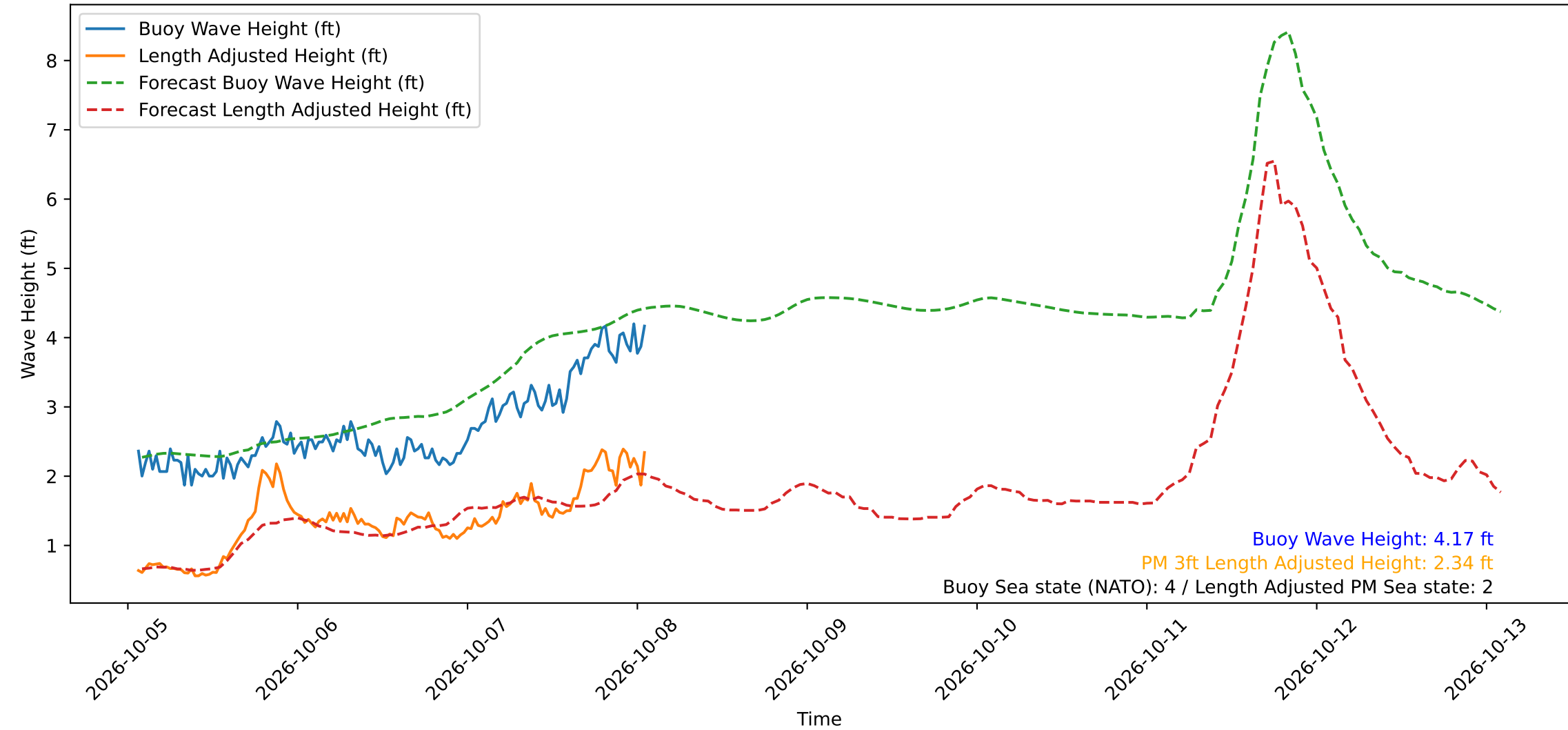
Wave Heights over Time for Oceanside Harbor at 2026-10-08 01:40:29
