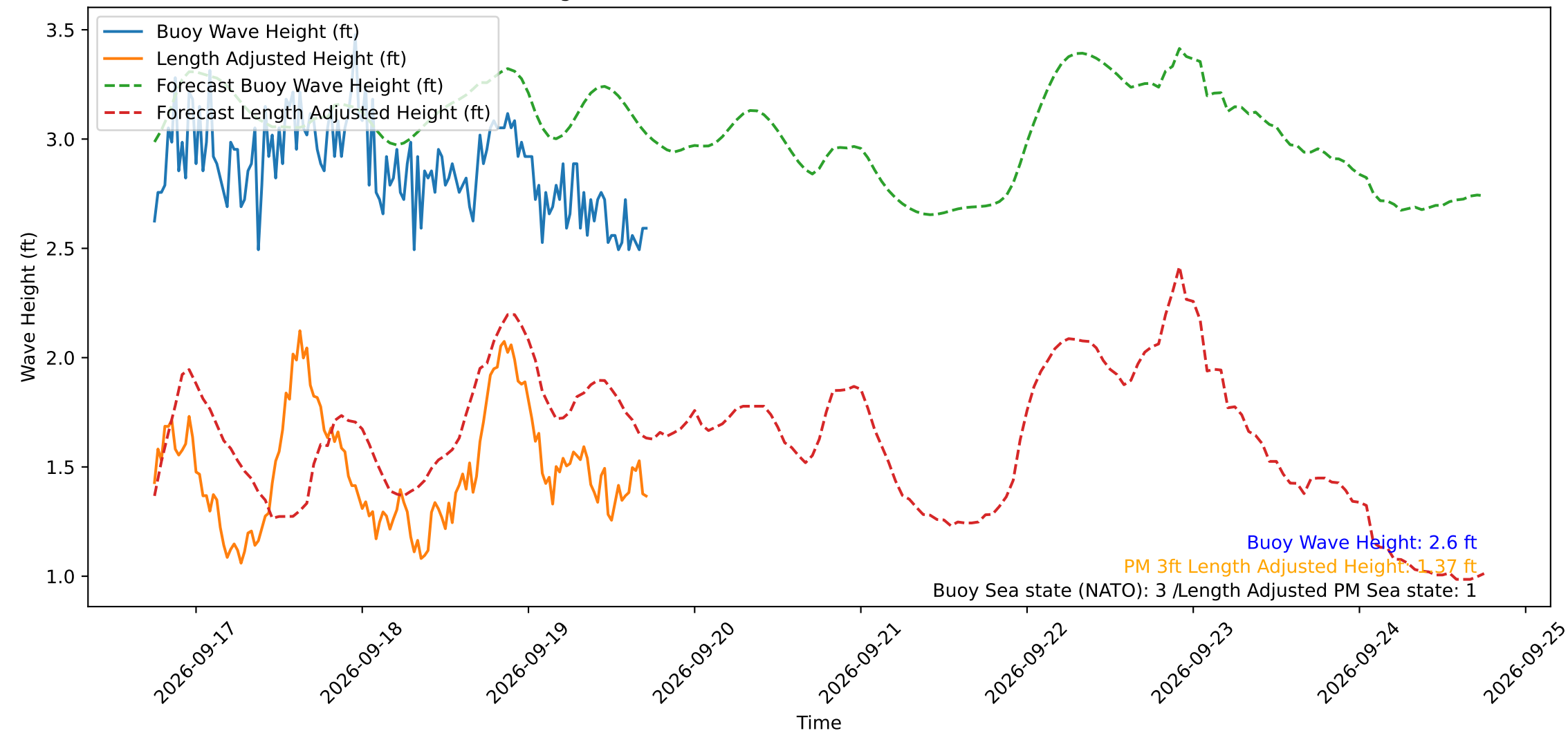
Wave Heights over Time for Green Beach at 2026-09-19 17:41:11
