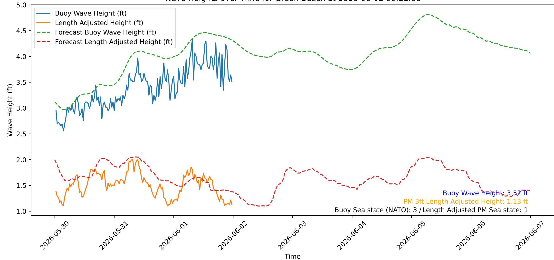
Wave Heights over Time for Green Beach at 2026-06-02 00:21:08
