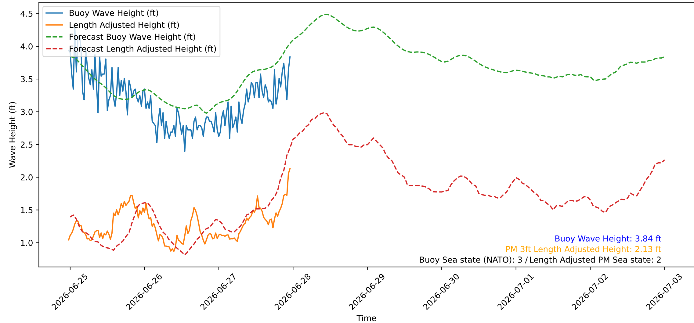
Wave Heights over Time for Oceanside Harbor at 2026-06-27 23:40:26
