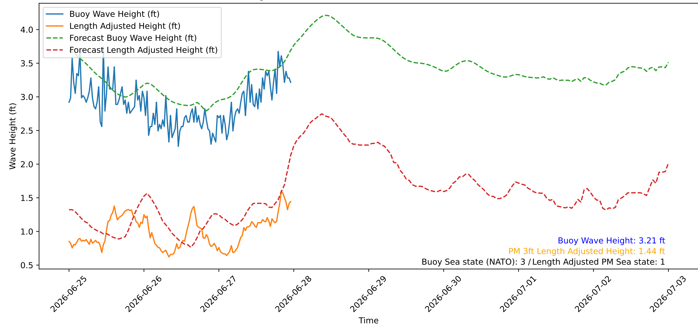
Wave Heights over Time for Red Beach at 2026-06-27 23:40:45
