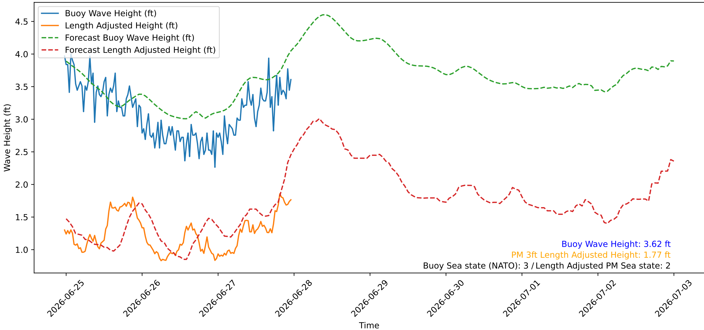
Wave Heights over Time for Green Beach at 2026-06-27 23:41:08
