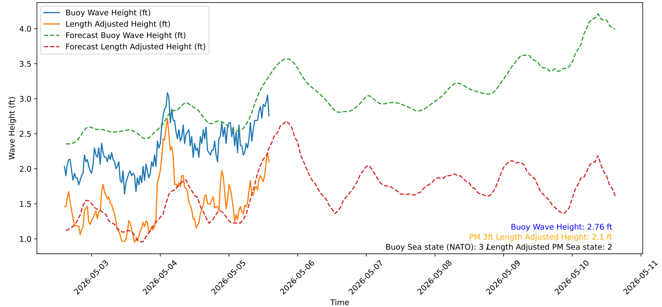
Wave Heights over Time for Oceanside Harbor at 2026-05-05 14:40:31
