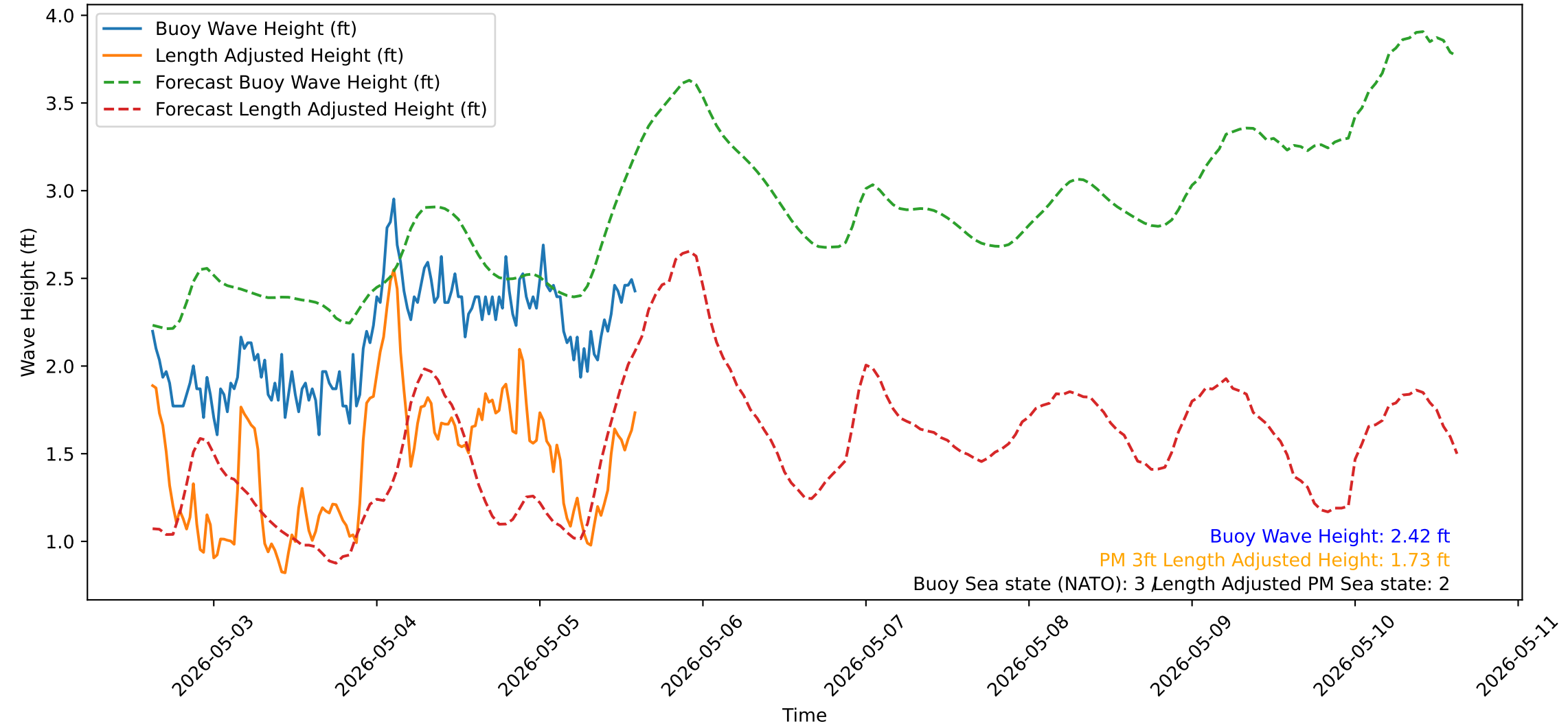
Wave Heights over Time for Red Beach at 2026-05-05 14:40:50
