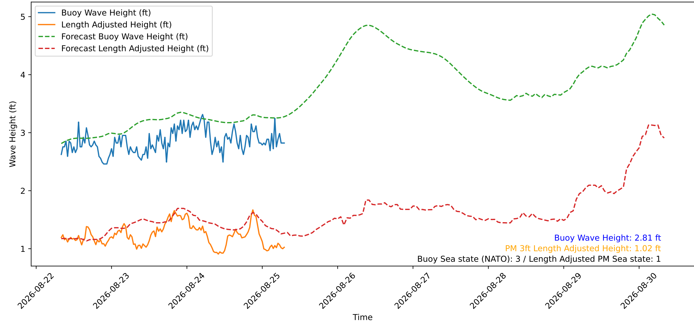
Wave Heights over Time for Green Beach at 2026-08-25 07:41:13
