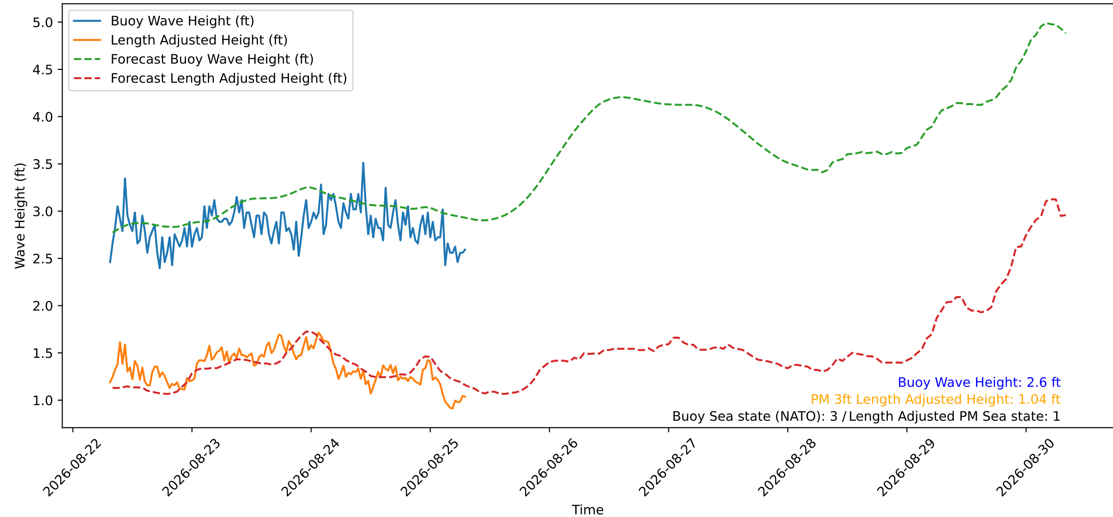
Wave Heights over Time for Oceanside Harbor at 2026-08-25 07:40:31
