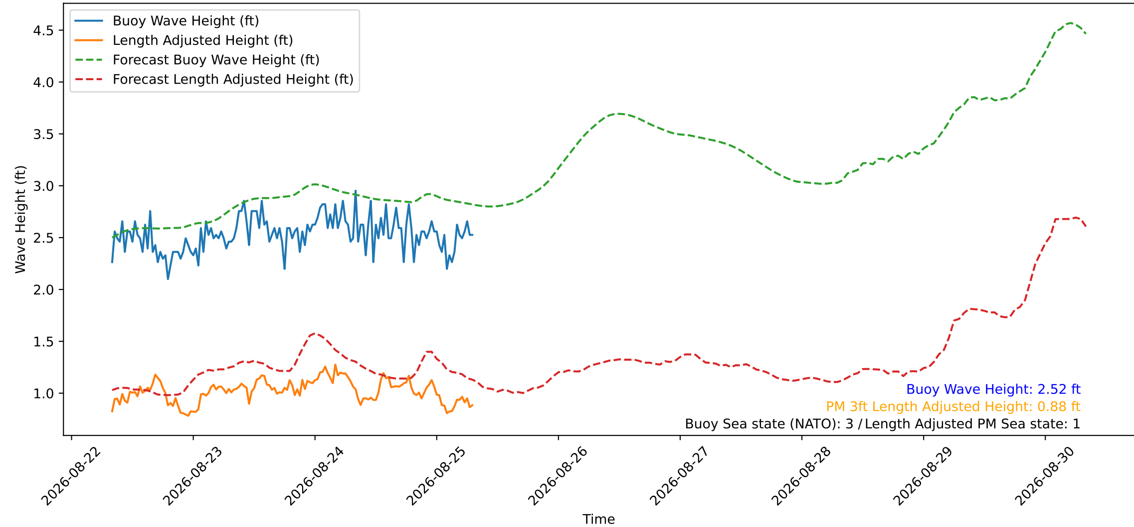
Wave Heights over Time for Red Beach at 2026-08-25 07:40:50
