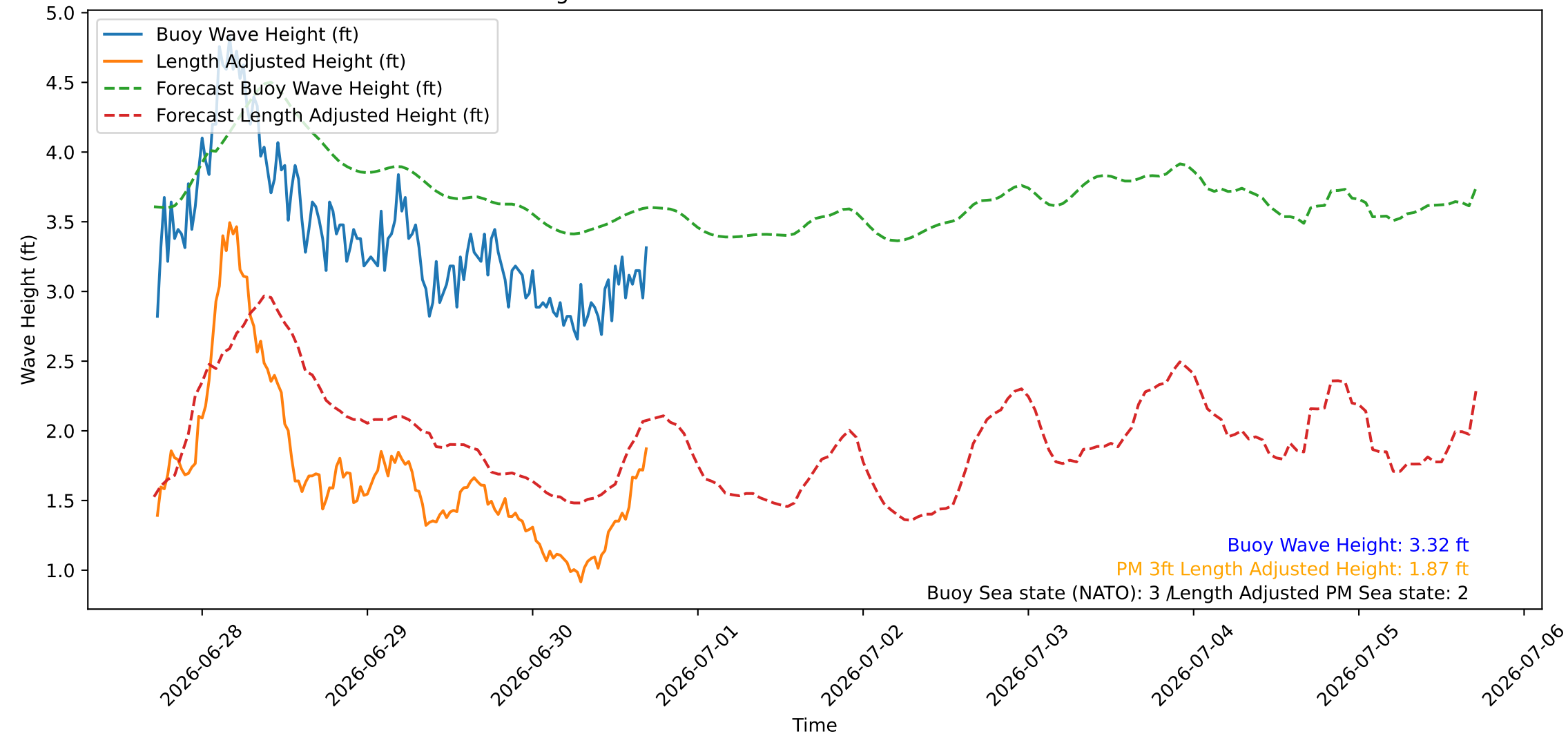
Wave Heights over Time for Green Beach at 2026-06-30 17:21:08
