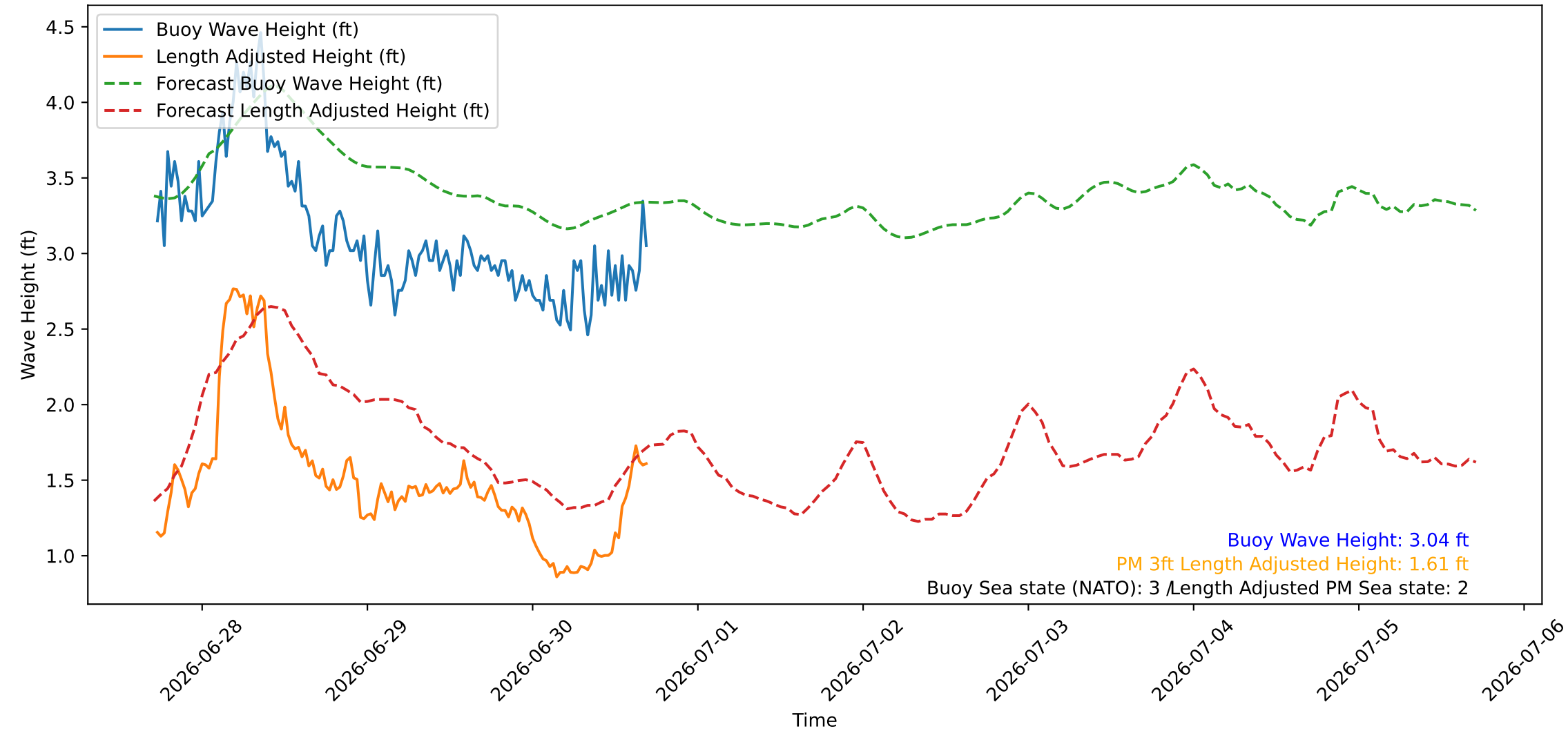
Wave Heights over Time for Red Beach at 2026-06-30 17:20:46
