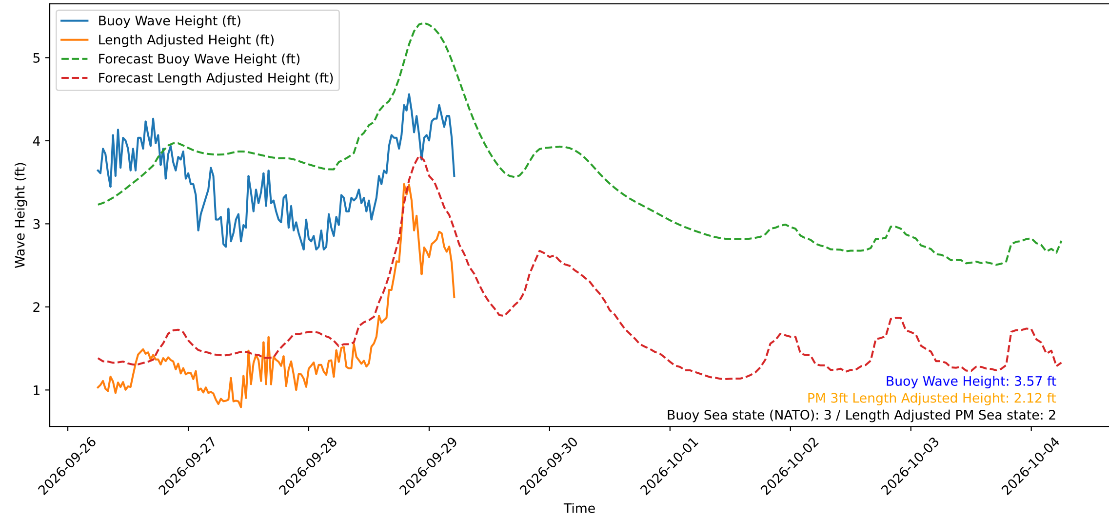
Wave Heights over Time for Green Beach at 2026-09-29 05:51:15
