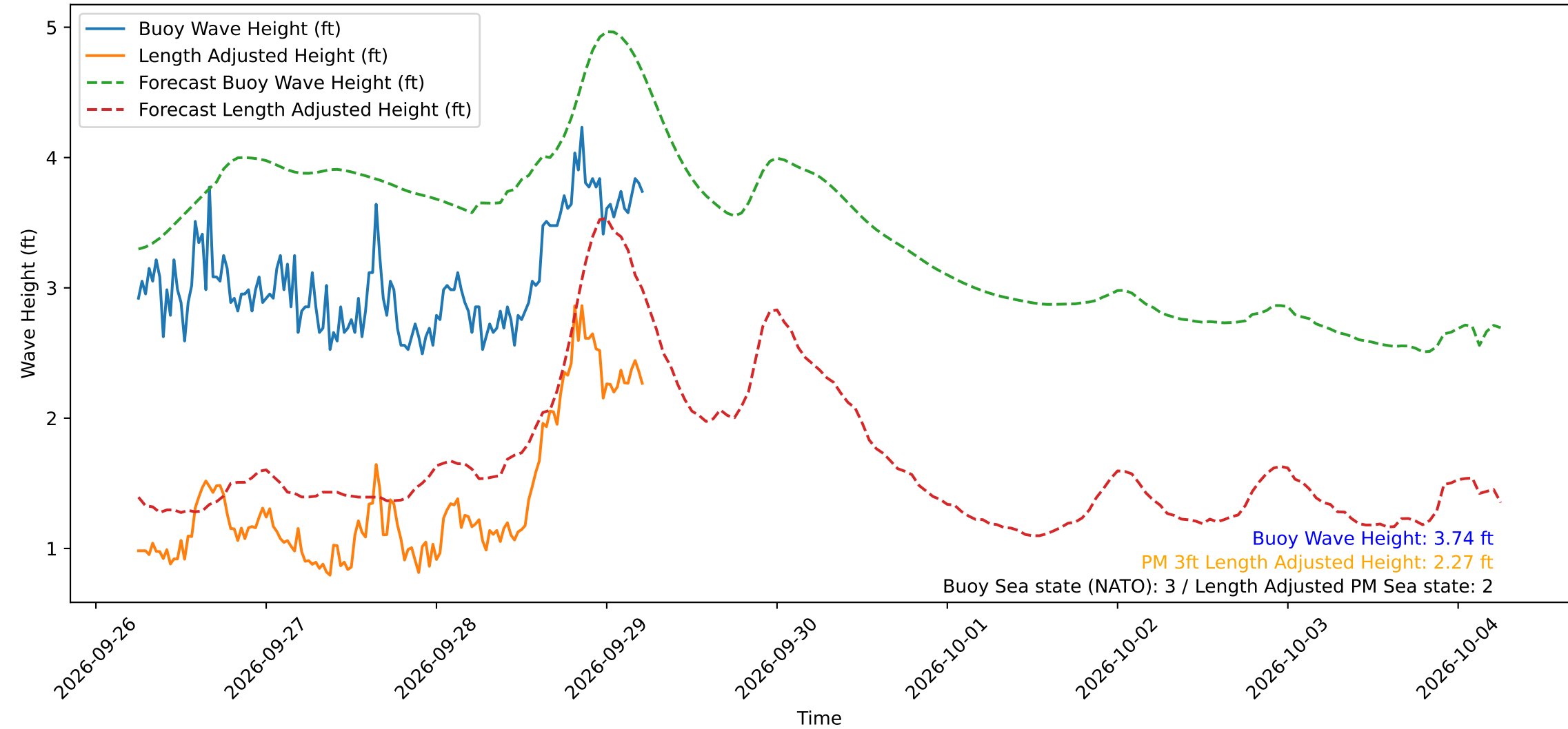
Wave Heights over Time for Oceanside Harbor at 2026-09-29 05:50:29
