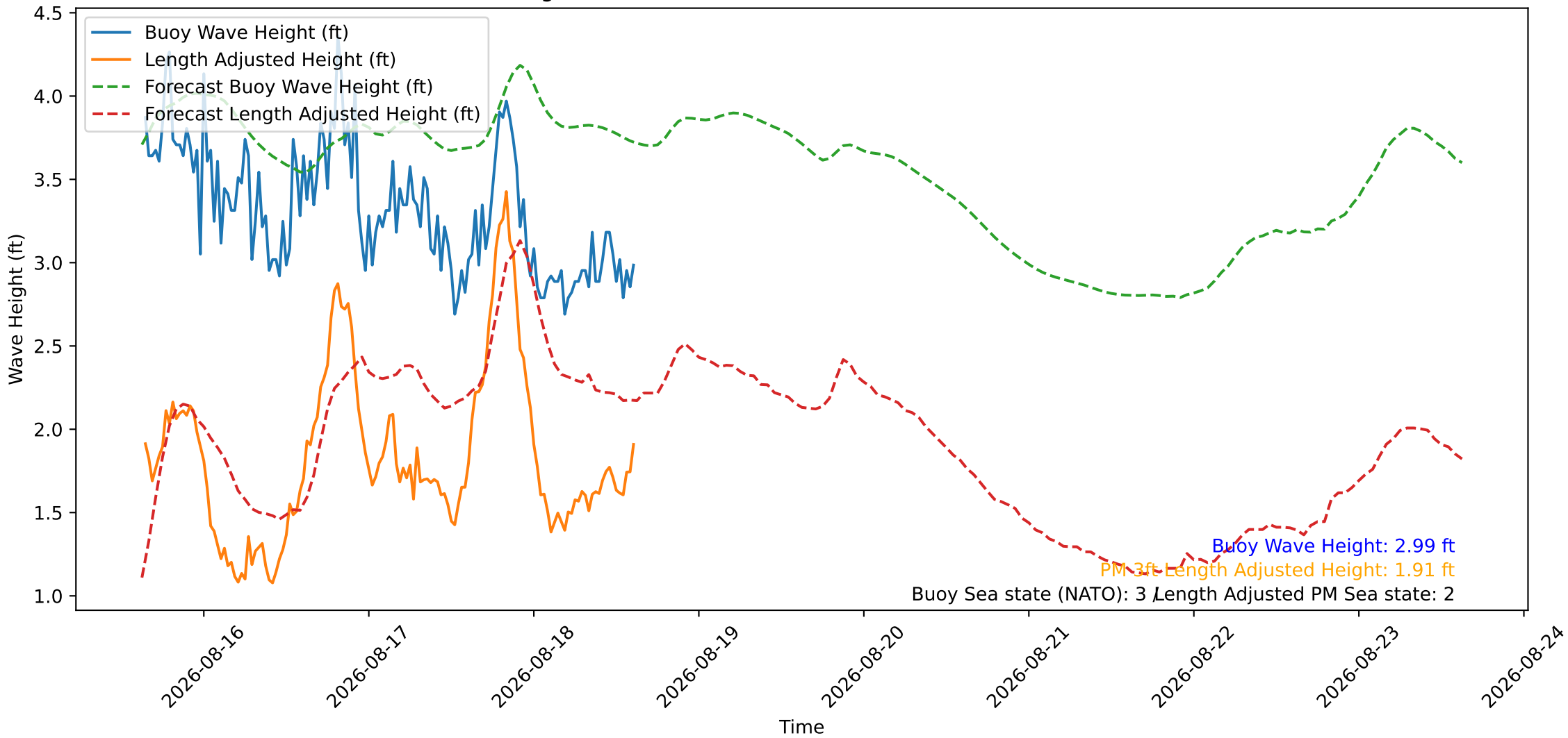
Wave Heights over Time for Green Beach at 2026-08-18 15:11:08
