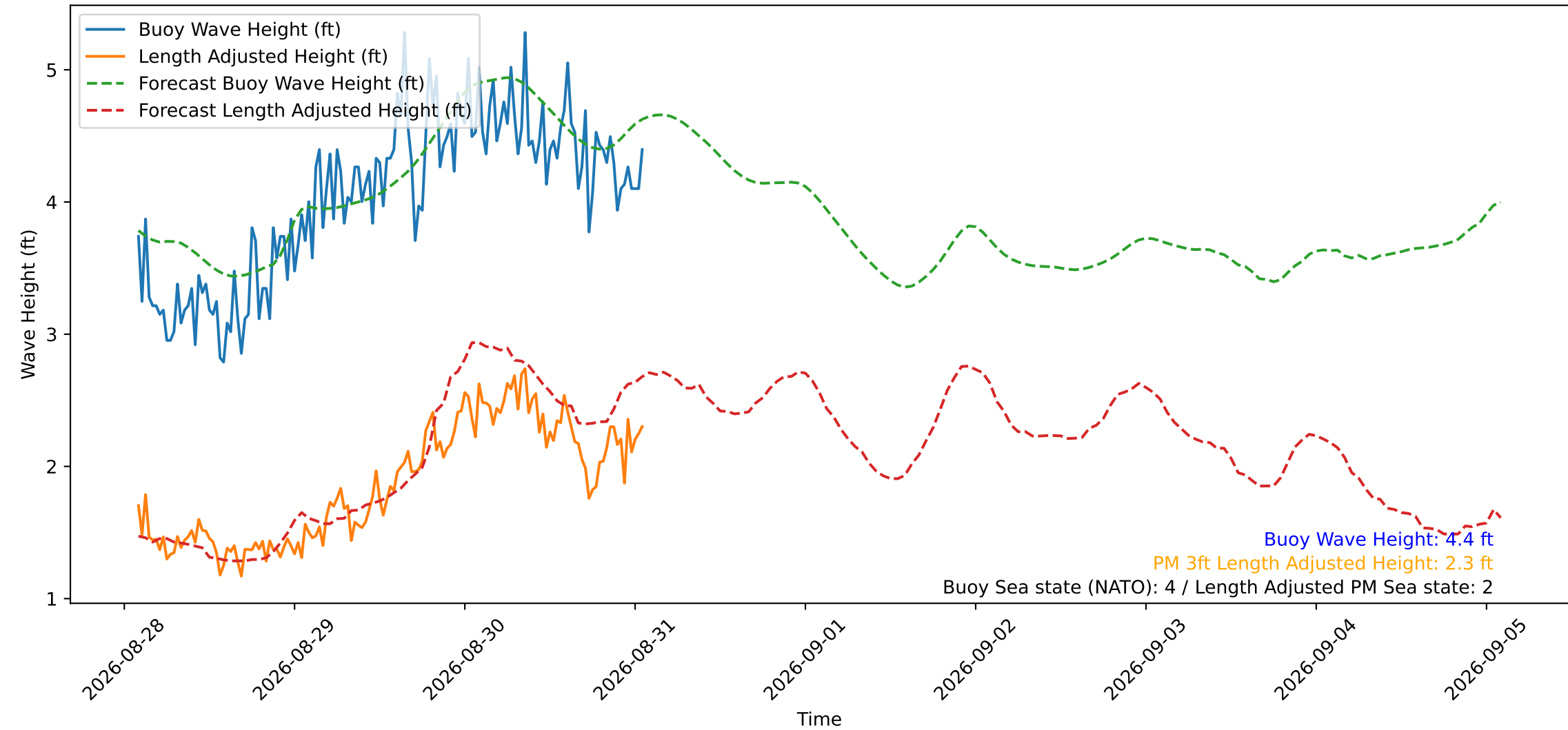
Wave Heights over Time for Oceanside Harbor at 2026-08-31 01:50:29
