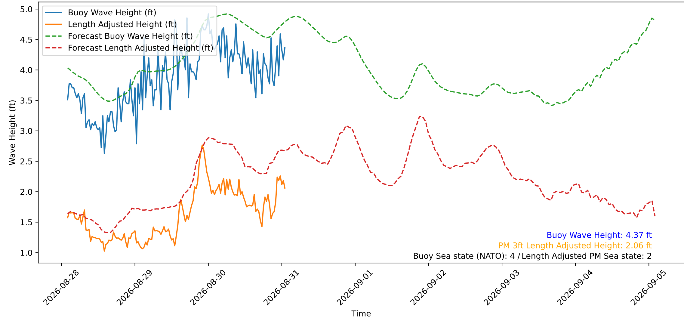
Wave Heights over Time for Green Beach at 2026-08-31 01:51:15
