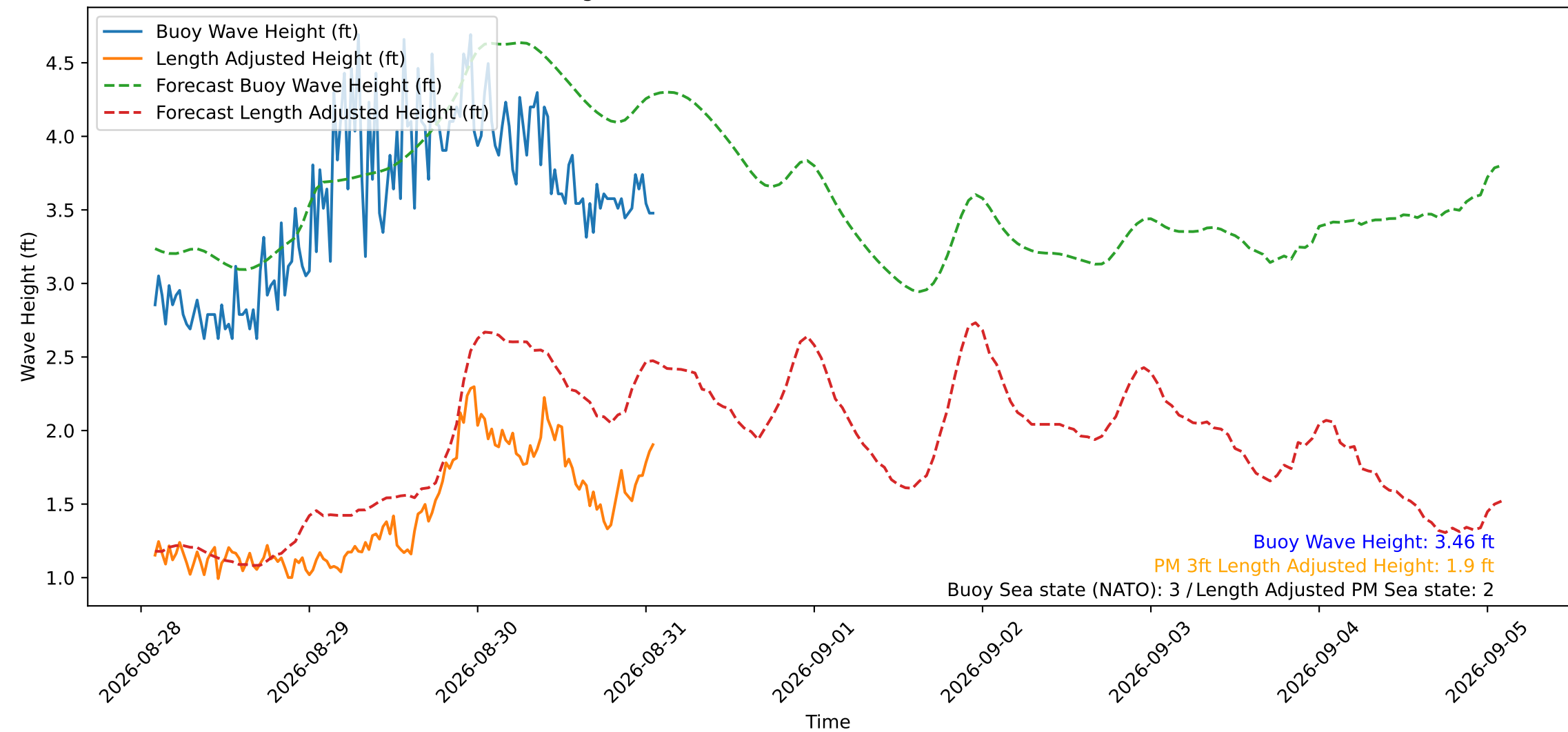
Wave Heights over Time for Red Beach at 2026-08-31 01:50:50
