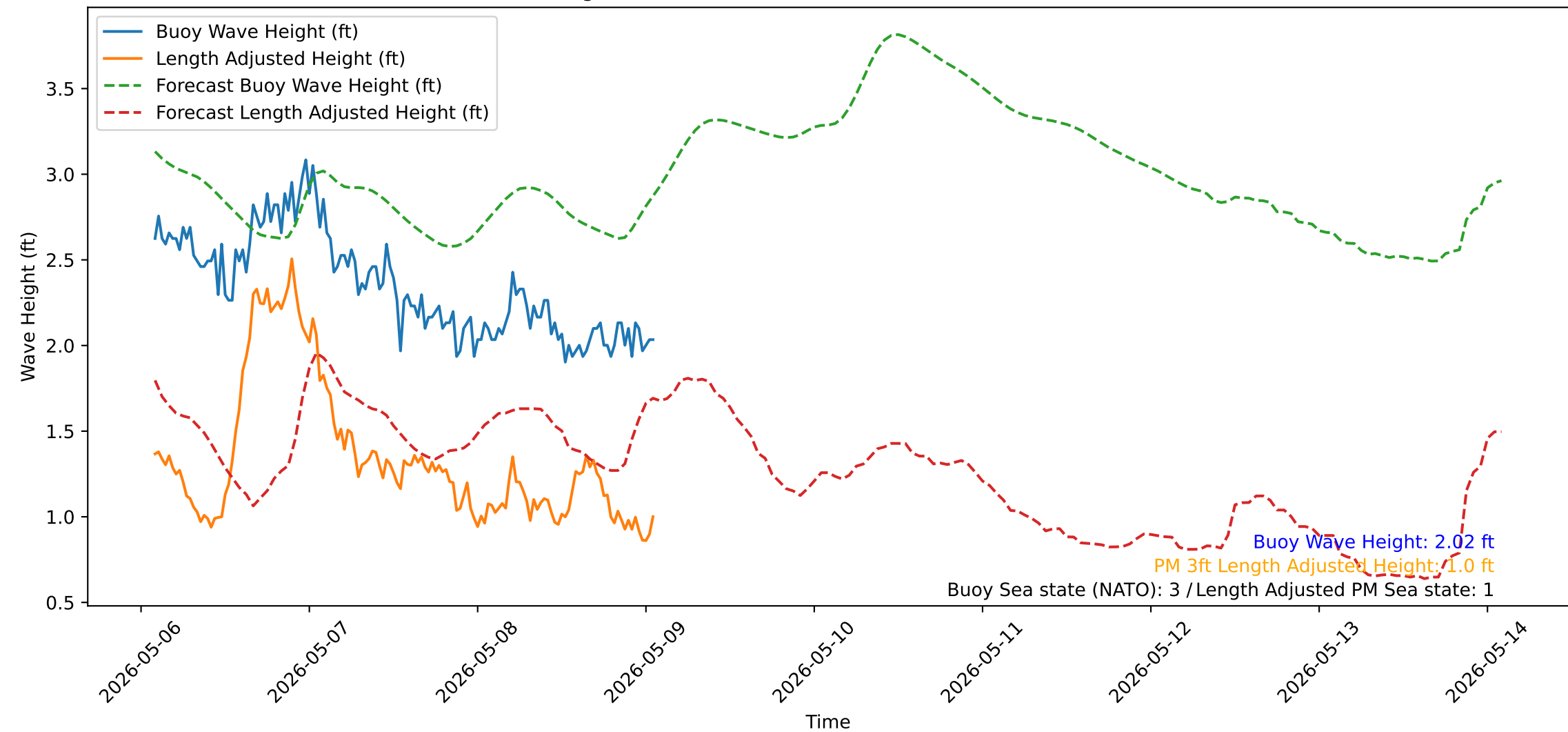
Wave Heights over Time for Red Beach at 2026-05-09 01:50:52
