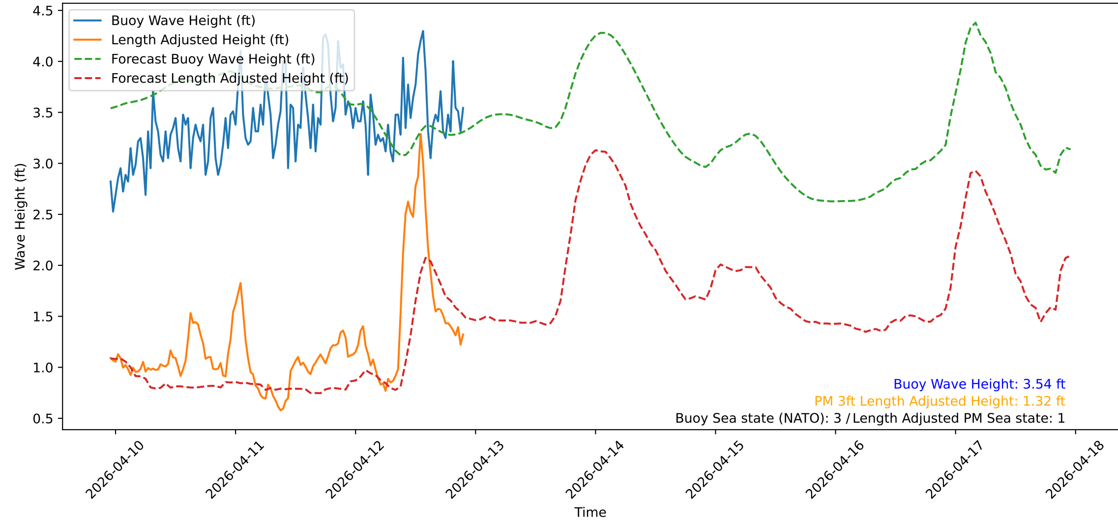
Wave Heights over Time for Red Beach at 2026-04-12 22:30:51
