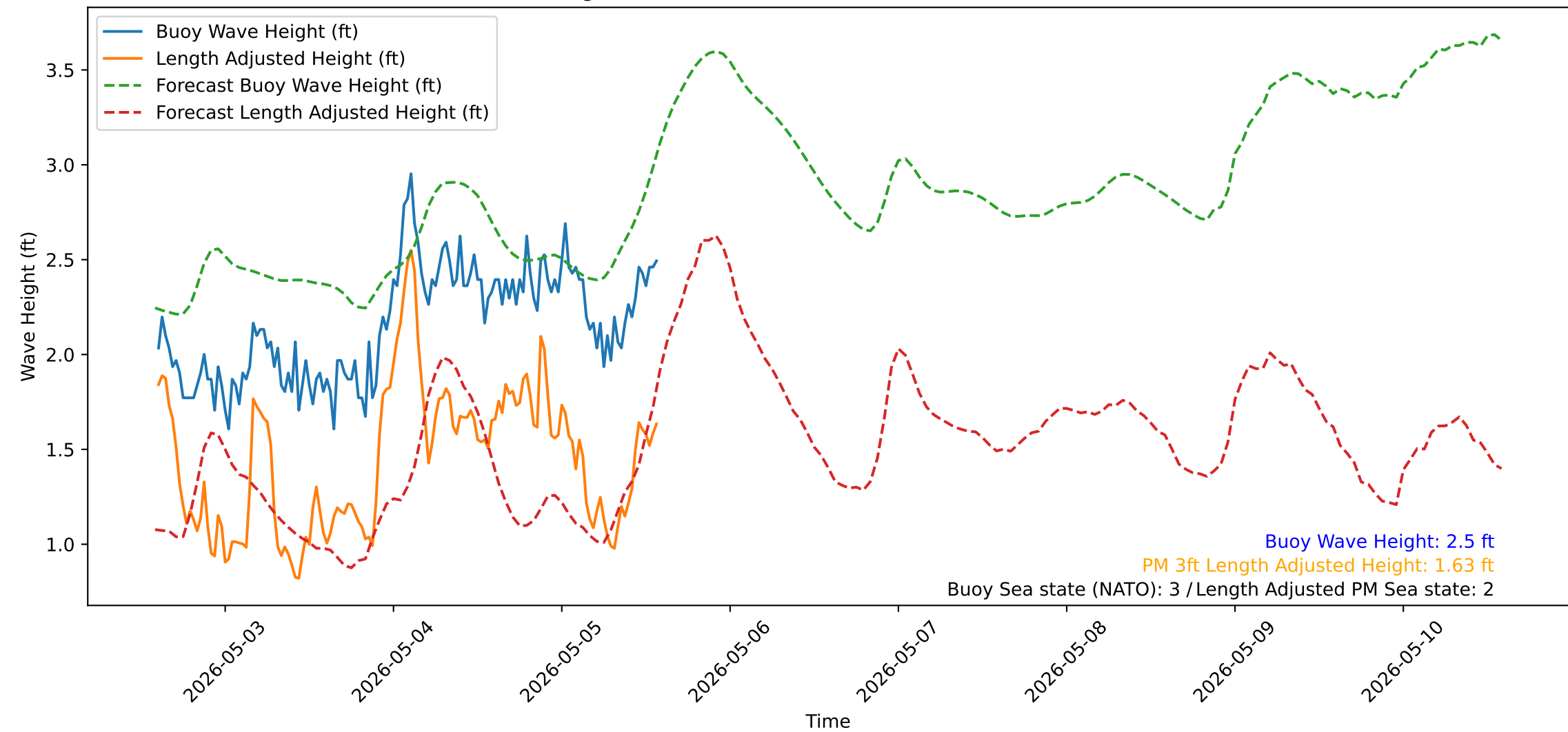
Wave Heights over Time for Red Beach at 2026-05-05 14:10:50
