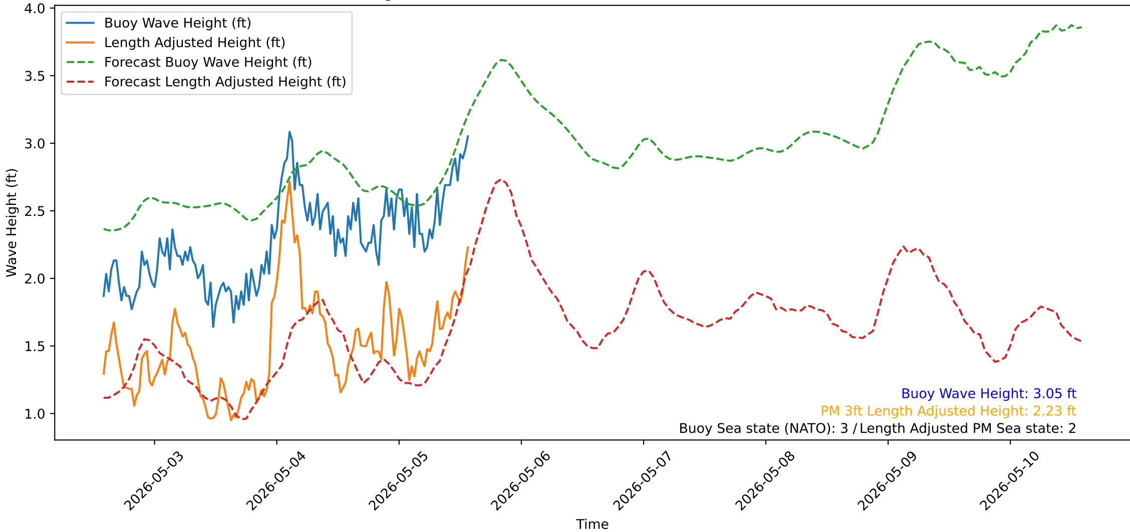
Wave Heights over Time for Oceanside Harbor at 2026-05-05 14:10:31
