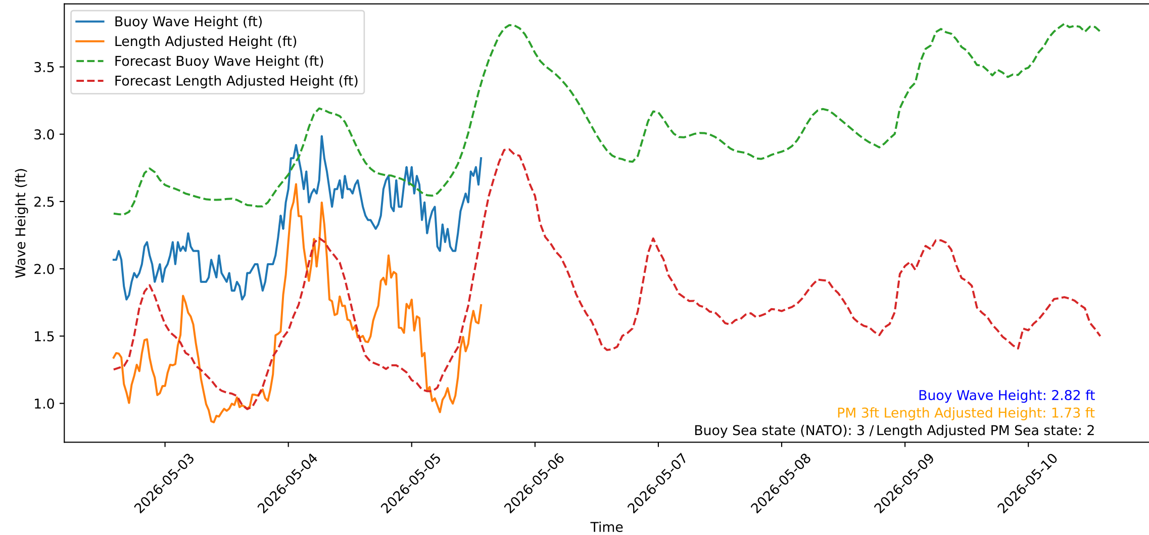
Wave Heights over Time for Green Beach at 2026-05-05 14:11:13
