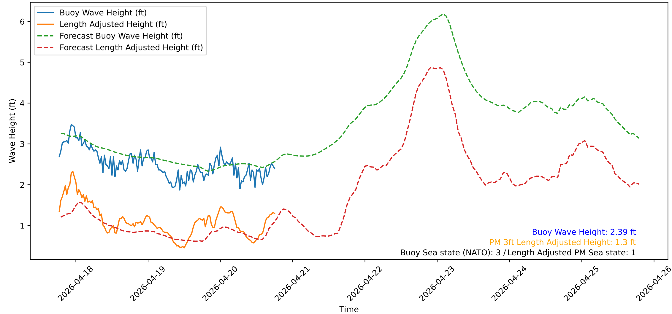
Wave Heights over Time for Green Beach at 2026-04-20 18:41:13
