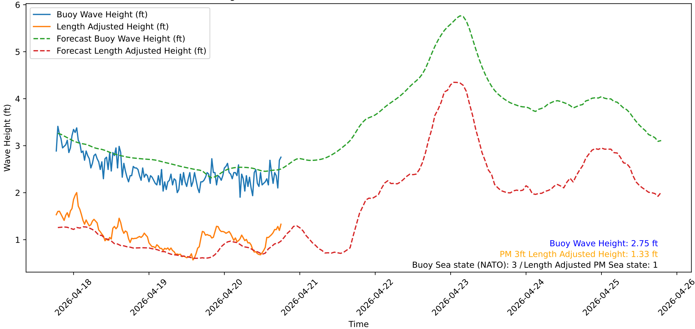
Wave Heights over Time for Oceanside Harbor at 2026-04-20 18:40:31
