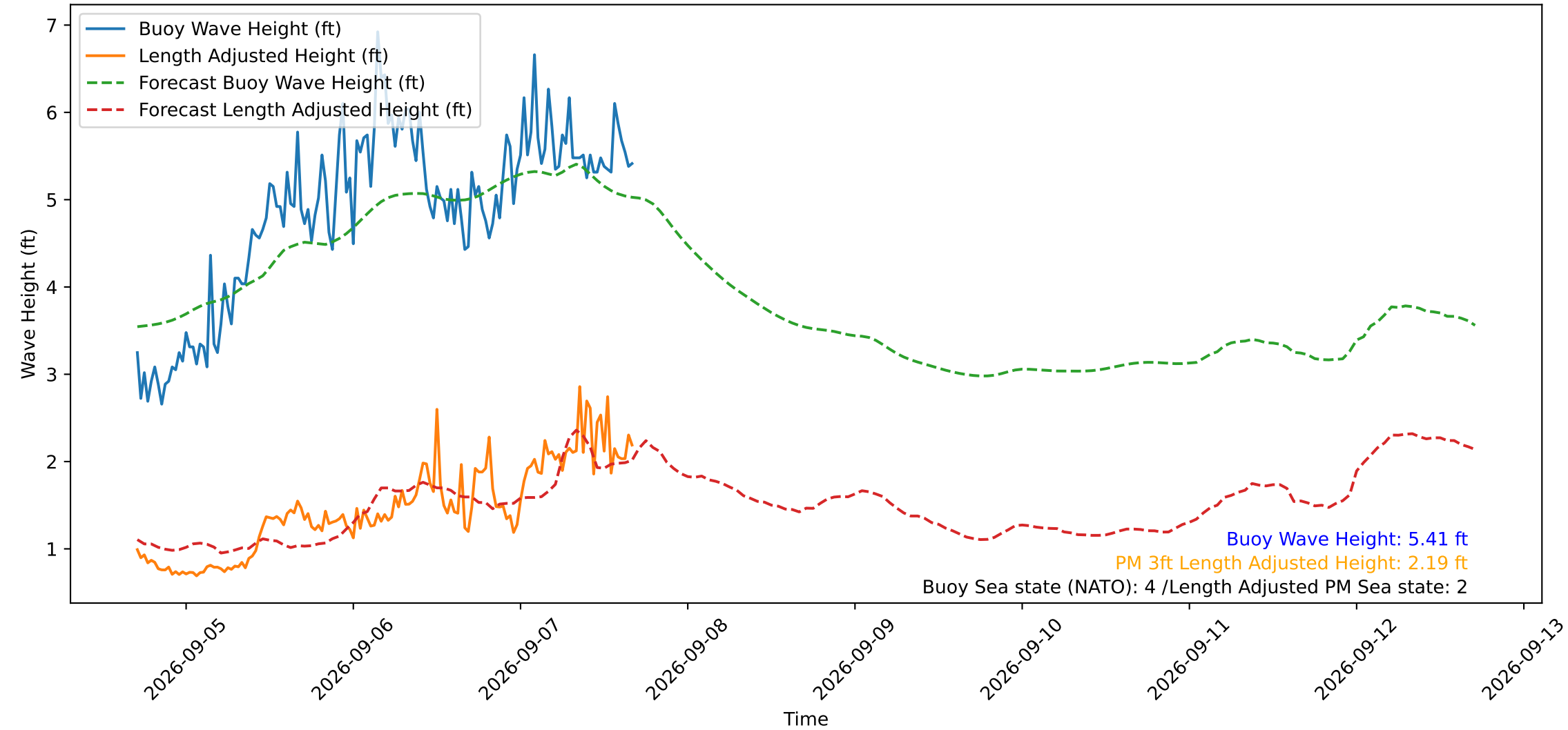
Wave Heights over Time for Red Beach at 2026-09-07 16:50:50
