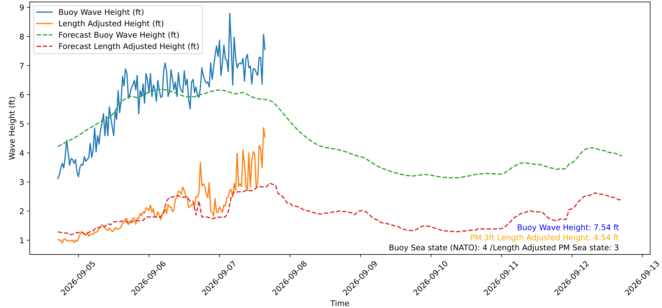
Wave Heights over Time for Green Beach at 2026-09-07 16:51:14
