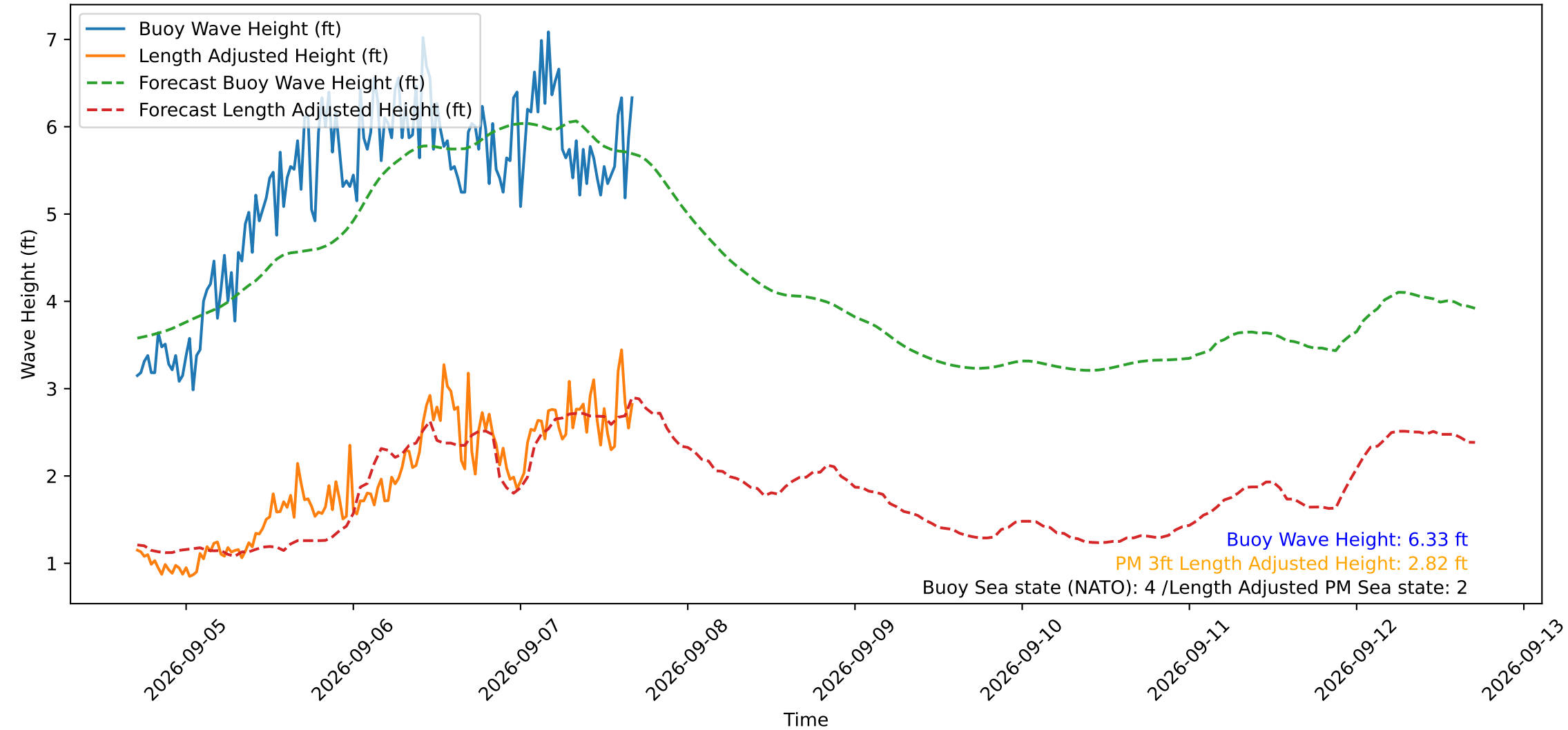
Wave Heights over Time for Oceanside Harbor at 2026-09-07 16:50:29
