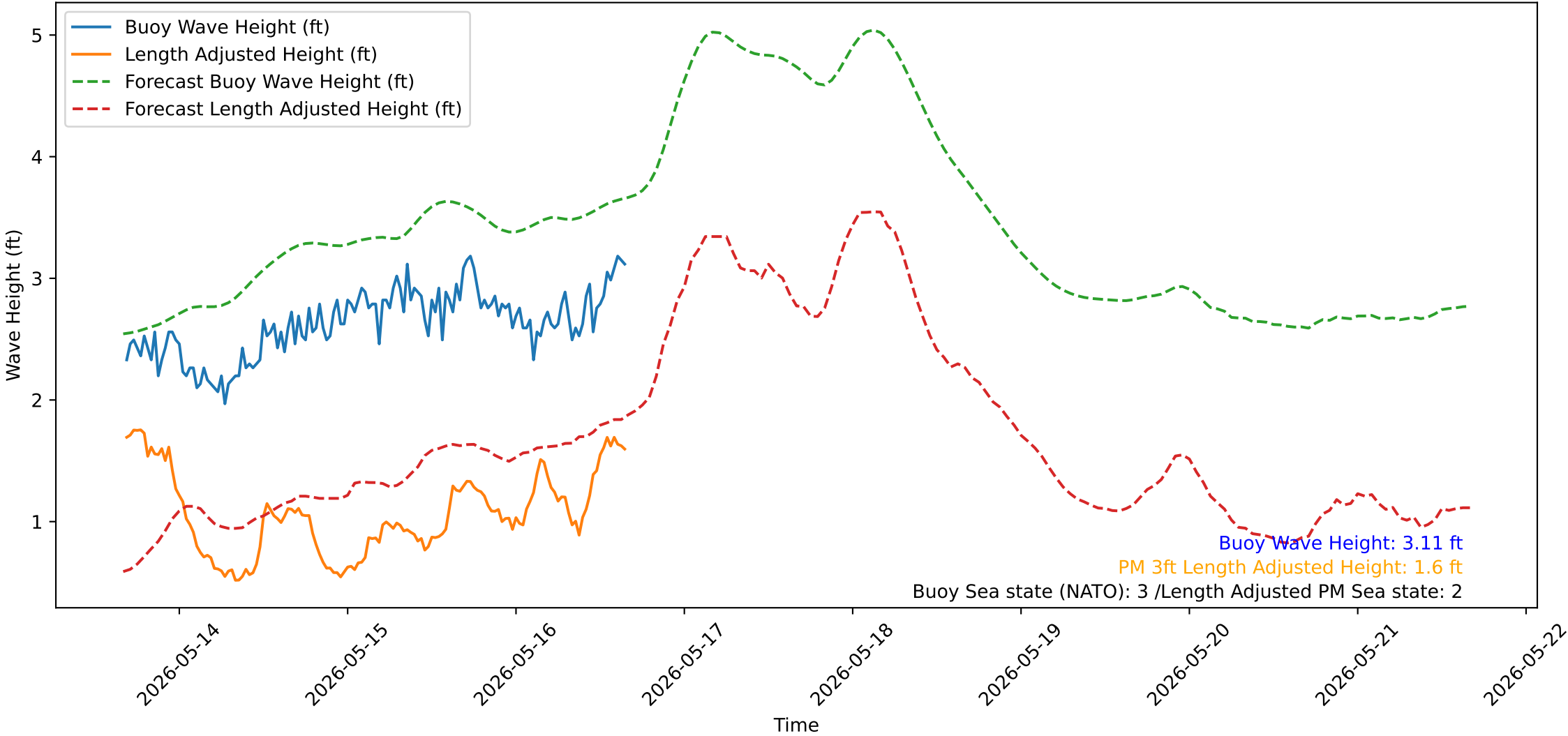
Wave Heights over Time for Red Beach at 2026-05-16 16:20:53
