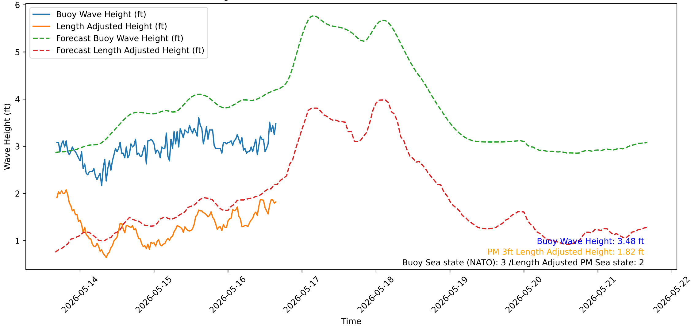
Wave Heights over Time for Oceanside Harbor at 2026-05-16 16:20:31
