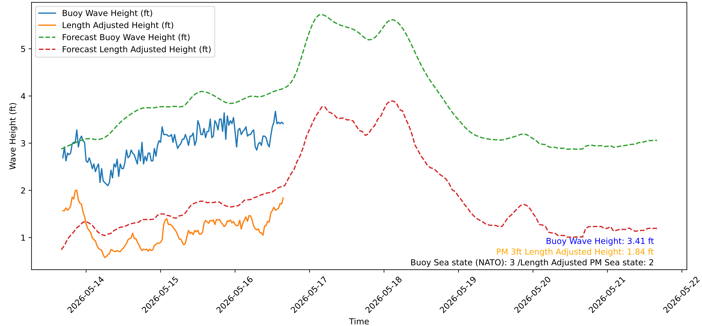
Wave Heights over Time for Green Beach at 2026-05-16 16:21:15
