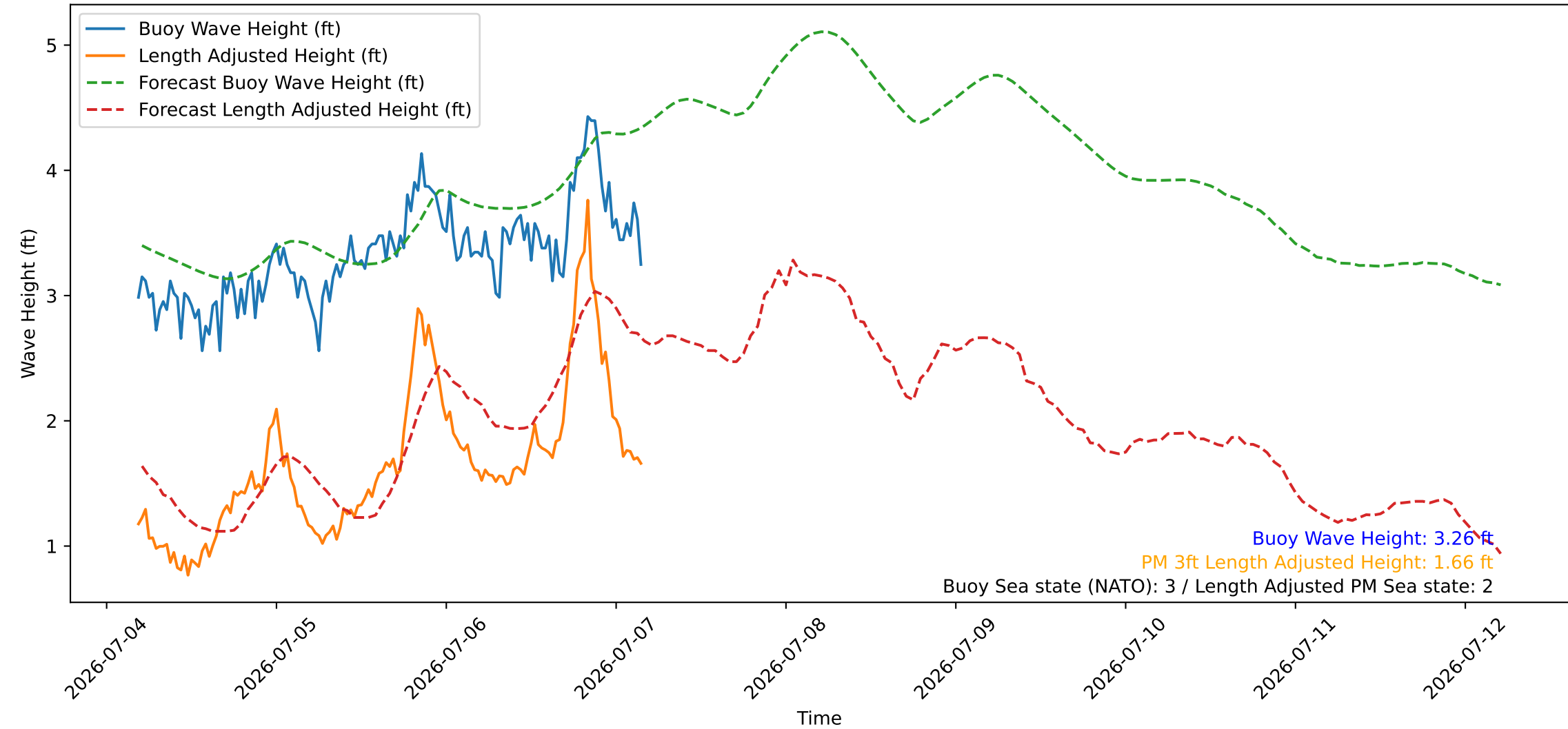
Wave Heights over Time for Green Beach at 2026-07-07 04:31:08
