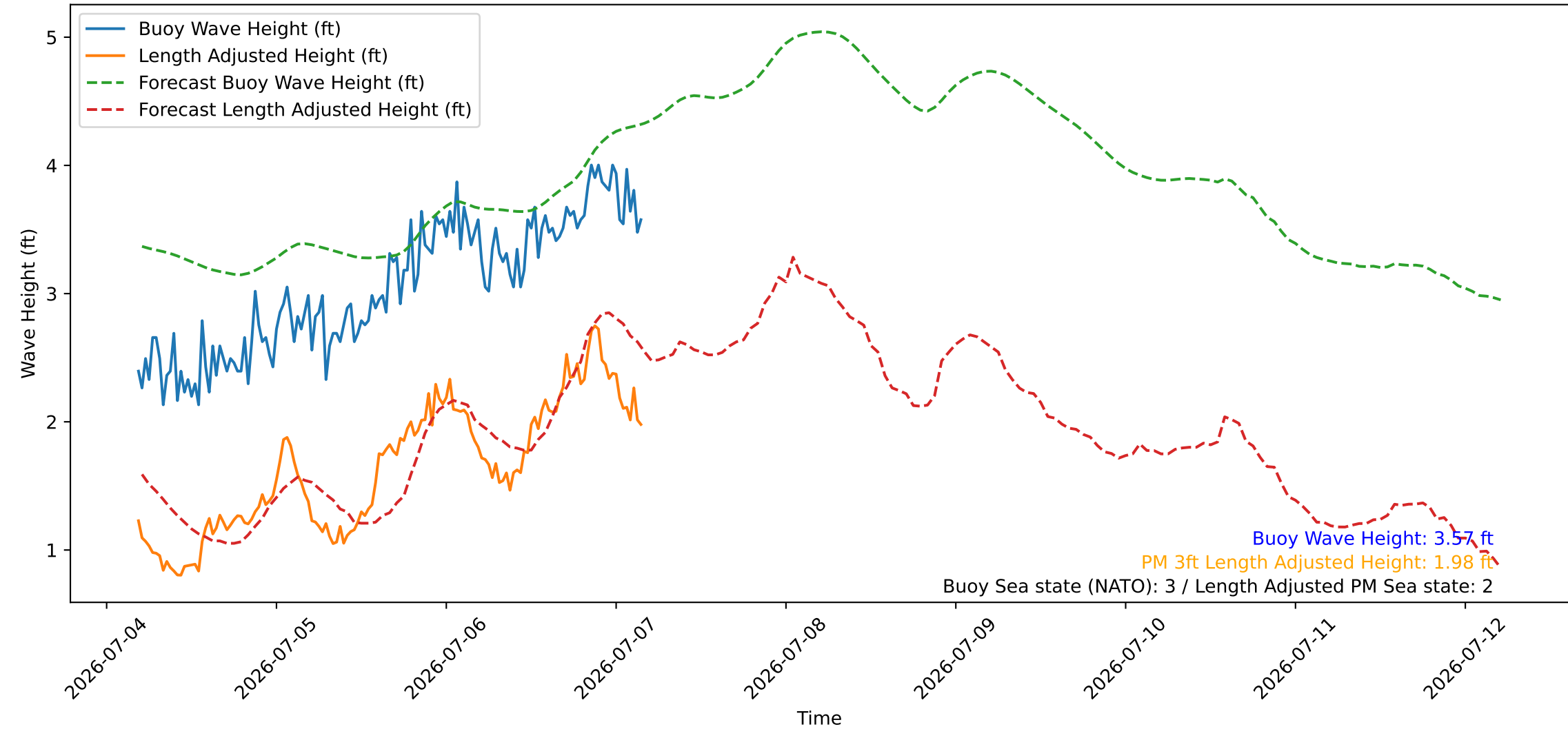
Wave Heights over Time for Oceanside Harbor at 2026-07-07 04:30:26
