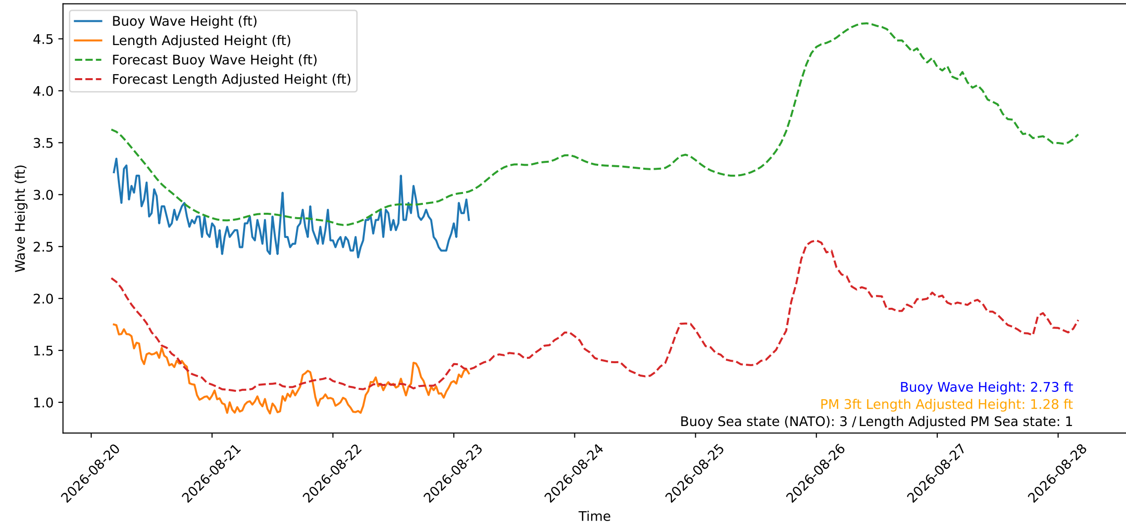
Wave Heights over Time for Green Beach at 2026-08-23 04:01:11
