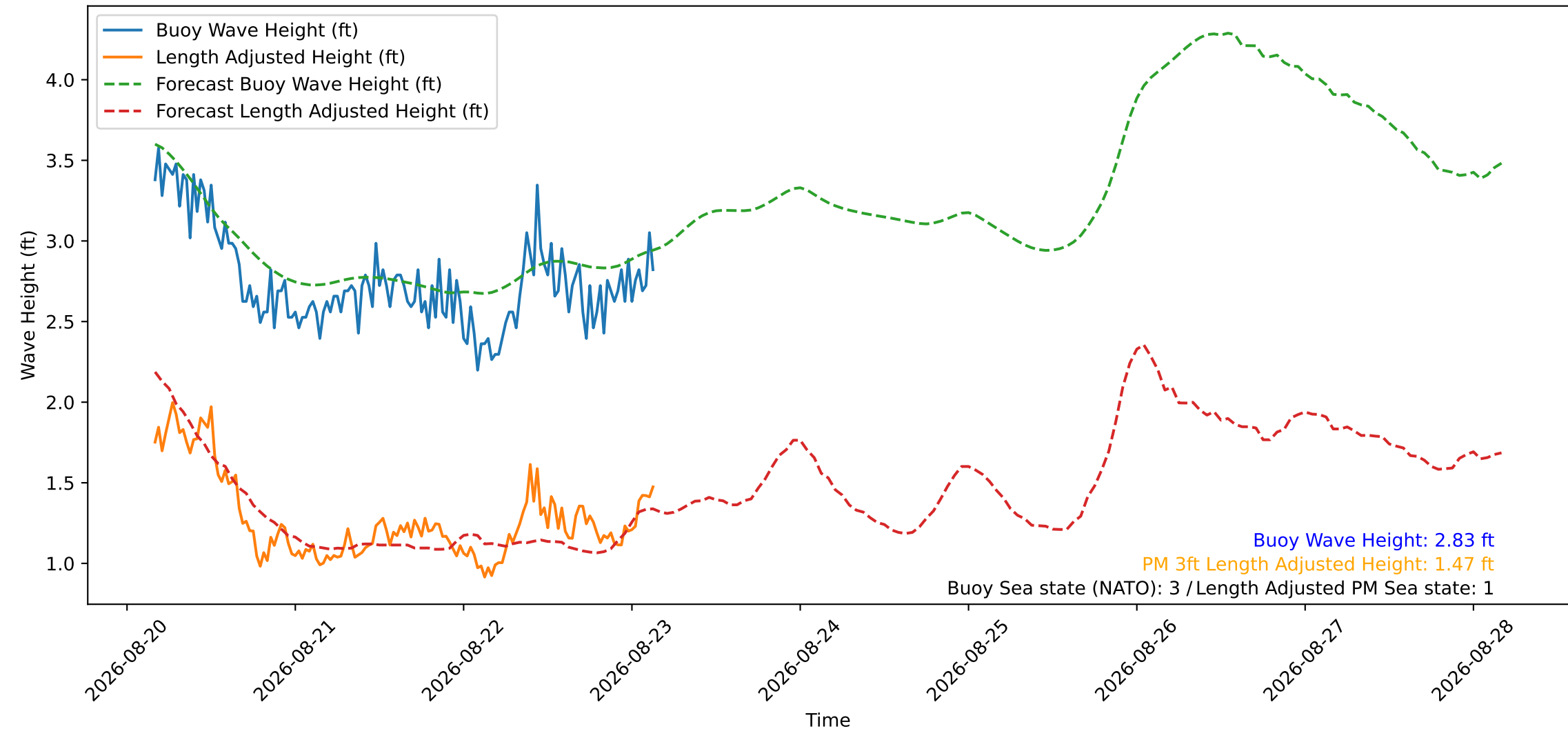
Wave Heights over Time for Oceanside Harbor at 2026-08-23 04:00:29
