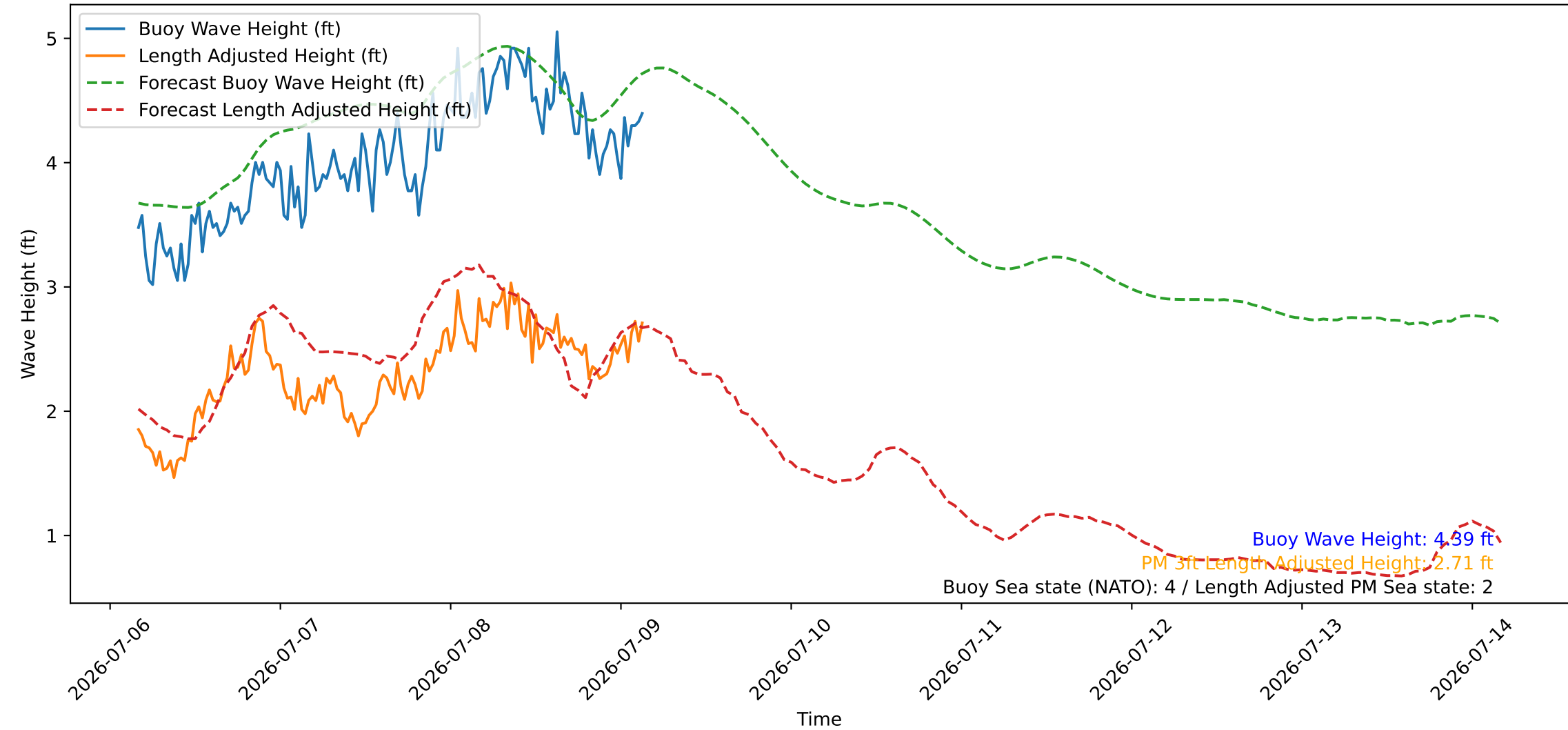
Wave Heights over Time for Oceanside Harbor at 2026-07-09 03:50:27
