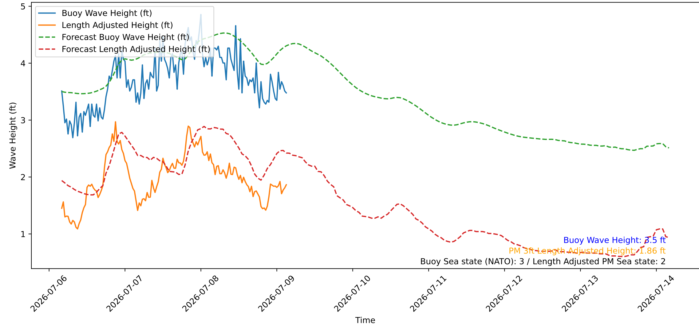
Wave Heights over Time for Red Beach at 2026-07-09 03:50:48
