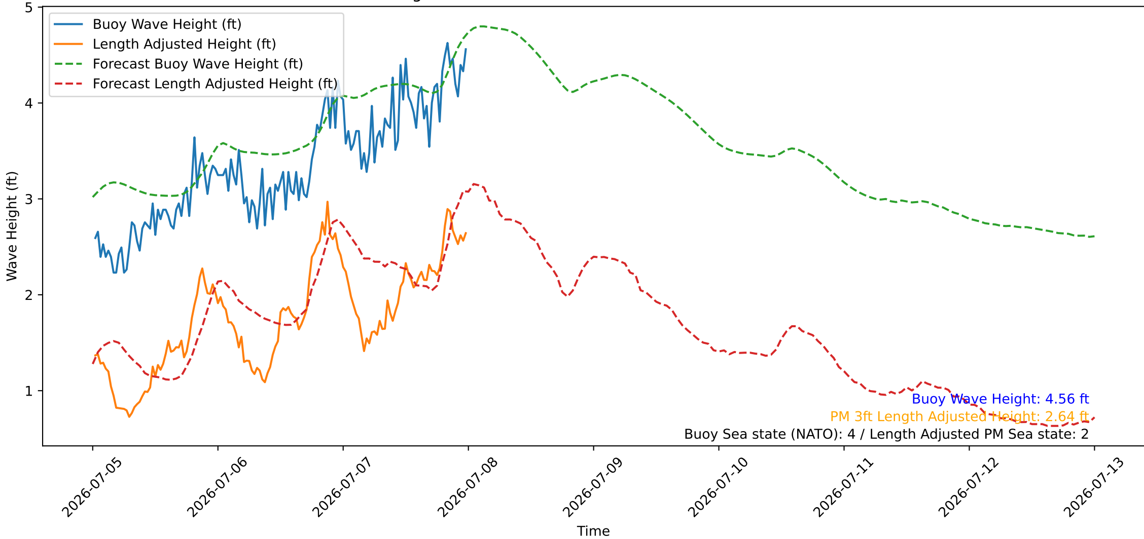
Wave Heights over Time for Red Beach at 2026-07-08 00:10:45
