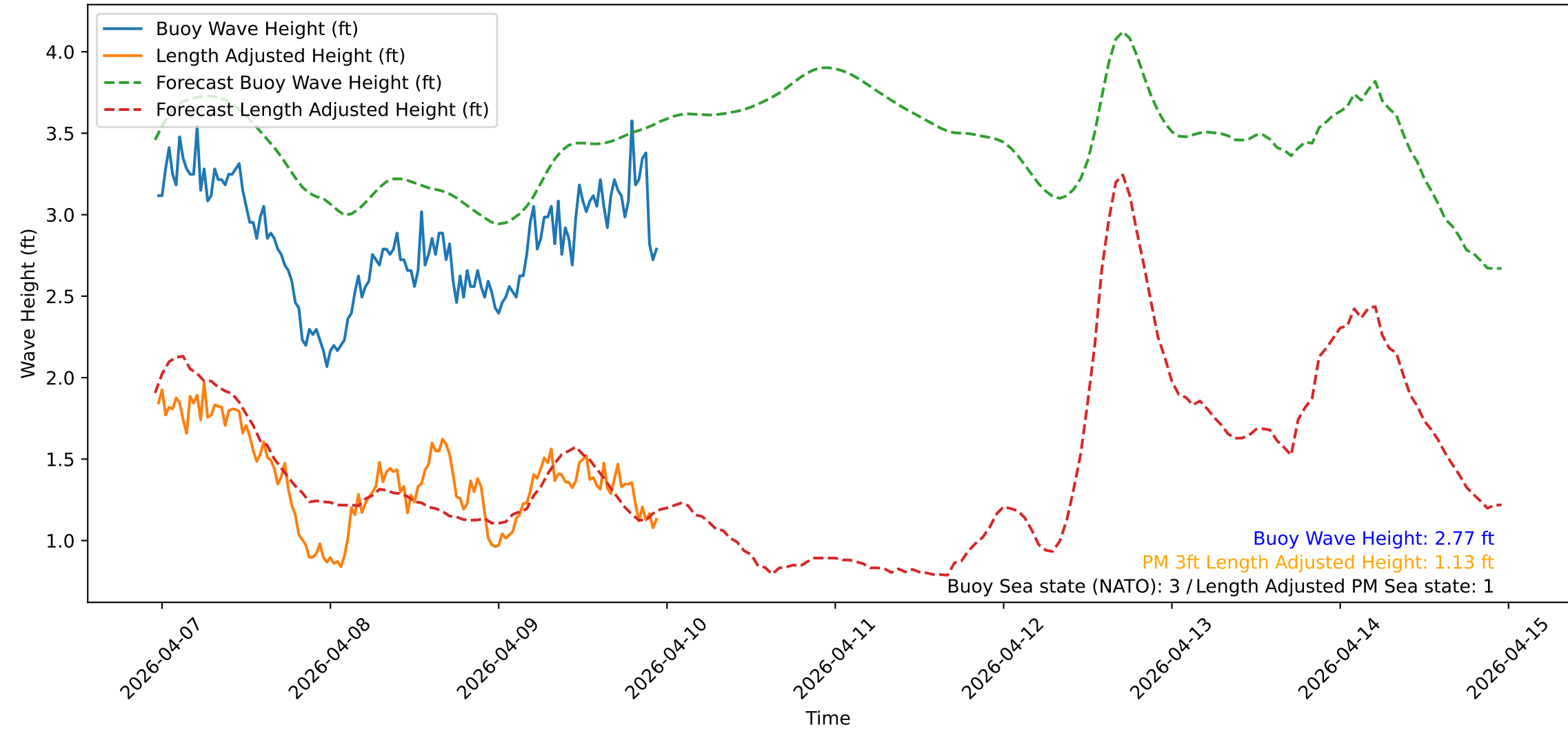
Wave Heights over Time for Red Beach at 2026-04-09 23:20:48
