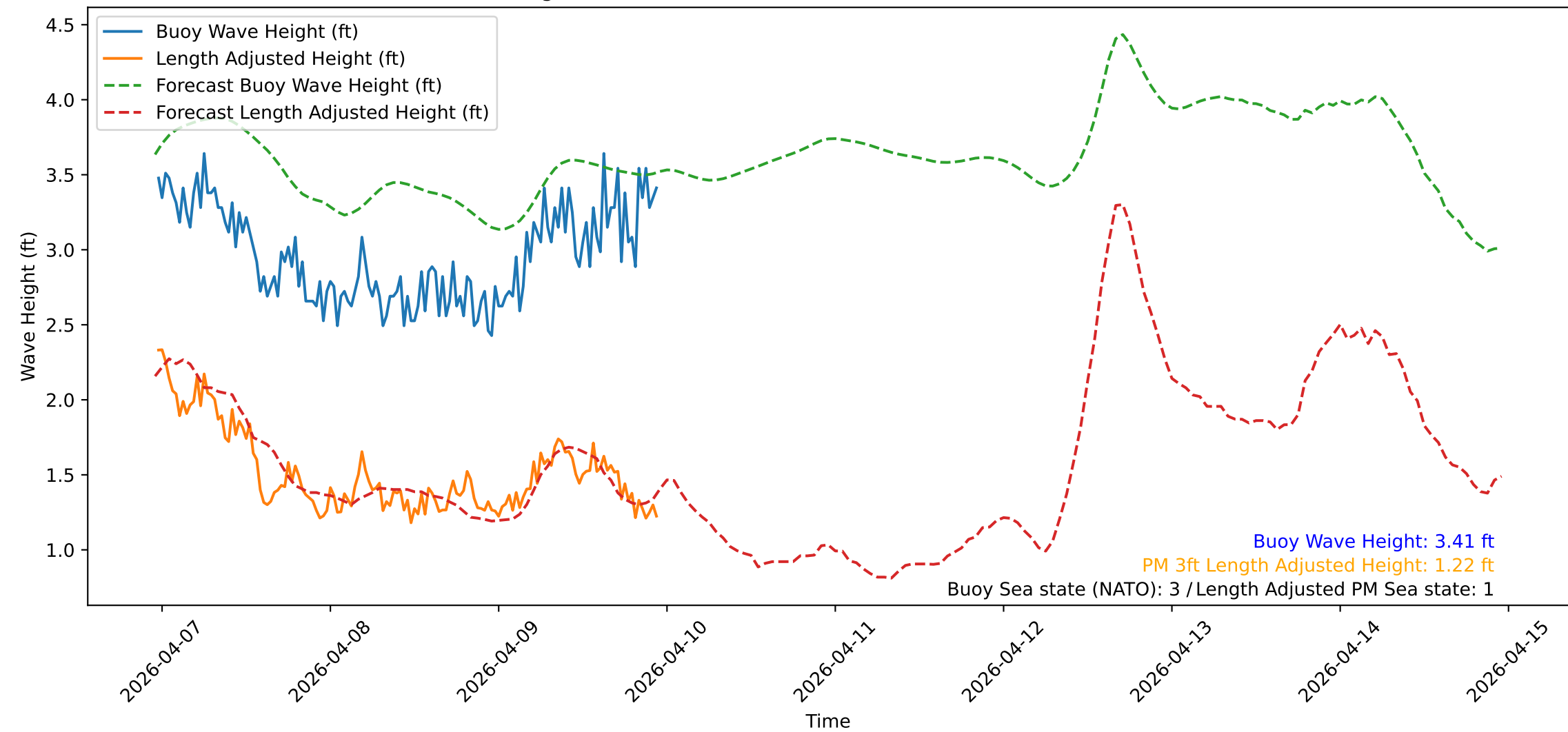
Wave Heights over Time for Oceanside Harbor at 2026-04-09 23:20:31
