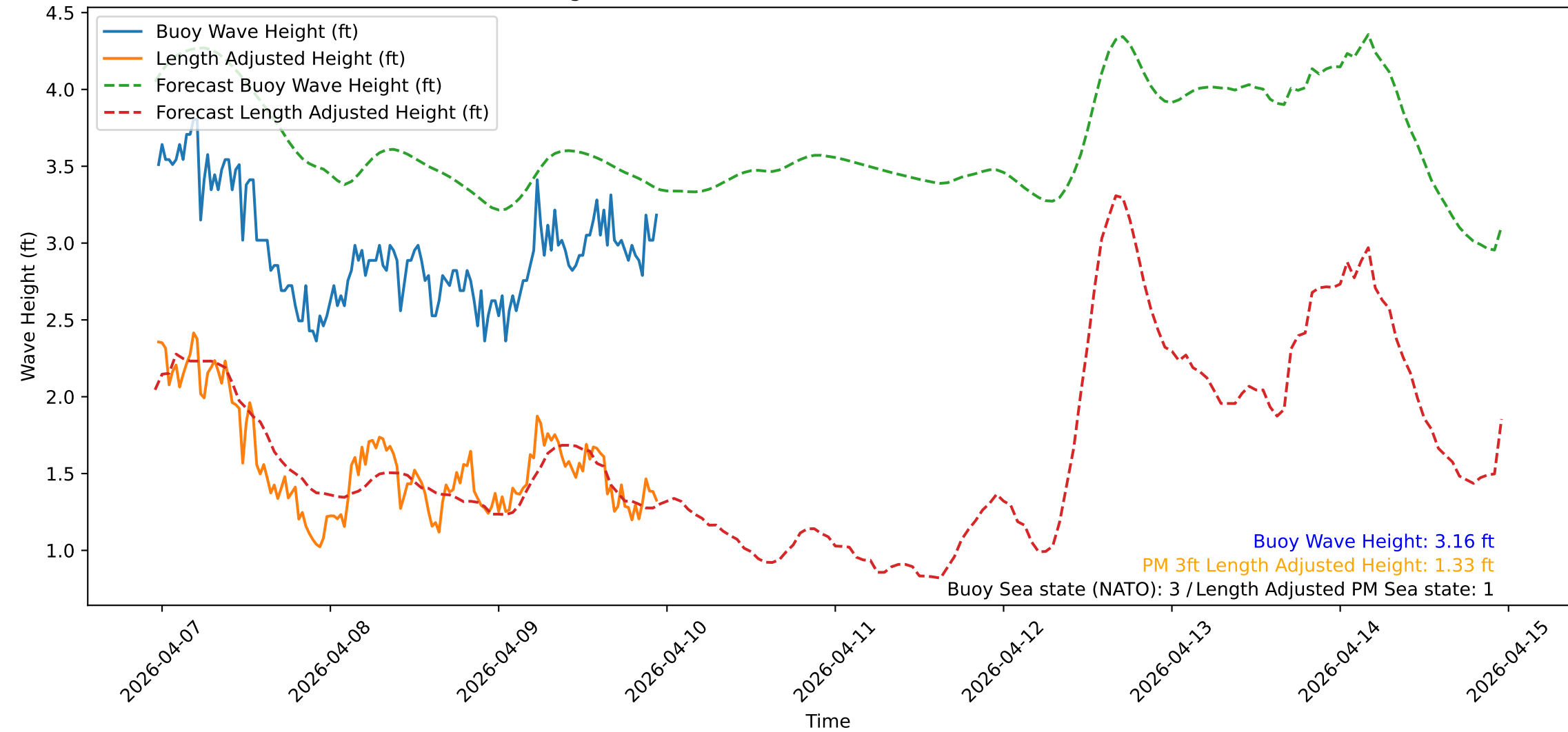
Wave Heights over Time for Green Beach at 2026-04-09 23:21:10
