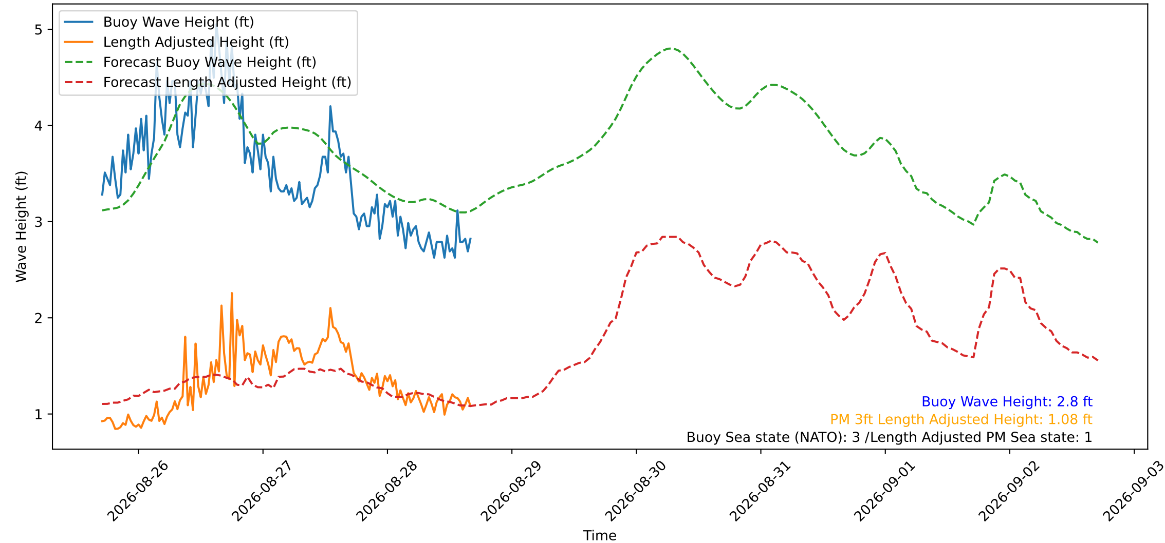
Wave Heights over Time for Red Beach at 2026-08-28 16:50:50
