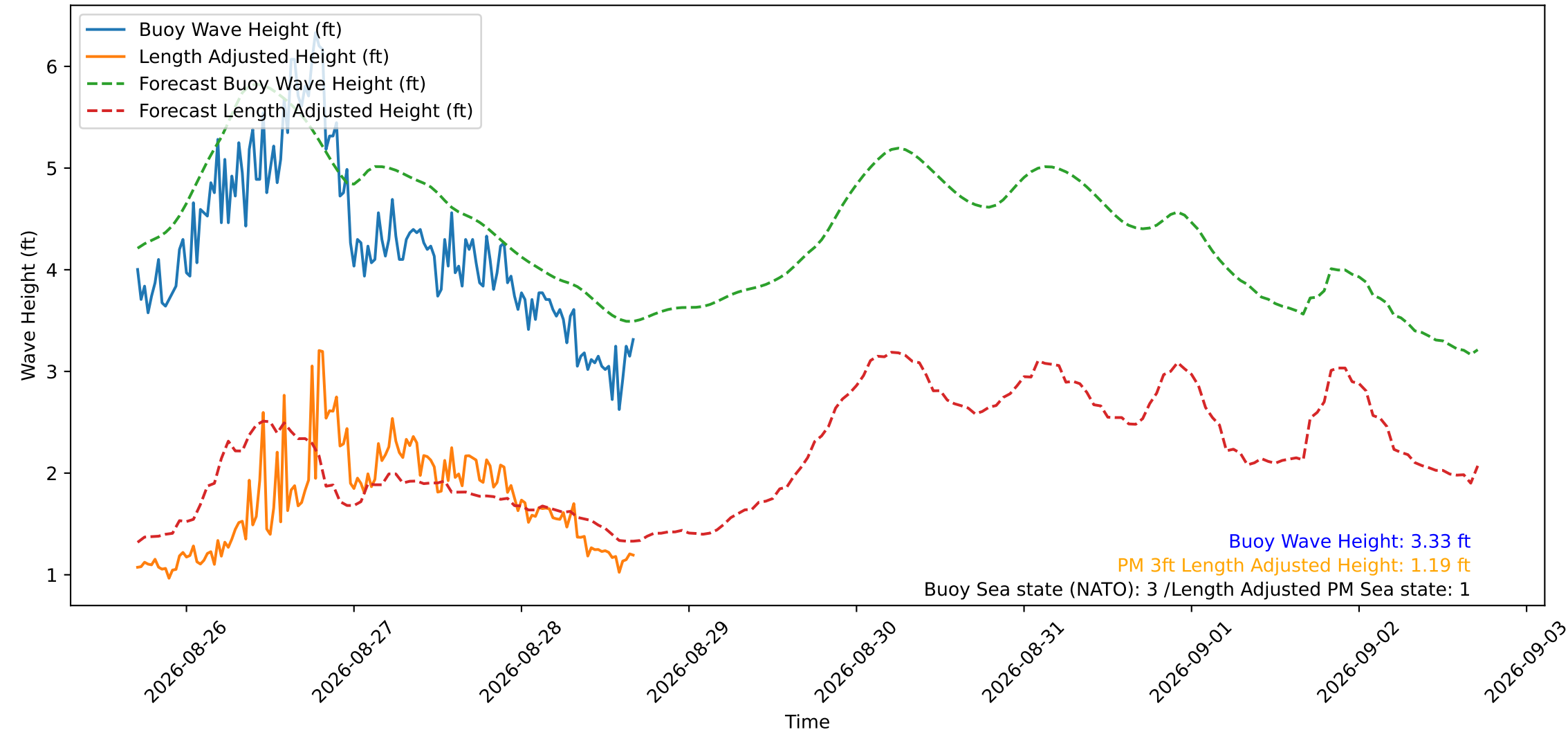
Wave Heights over Time for Green Beach at 2026-08-28 16:51:14
