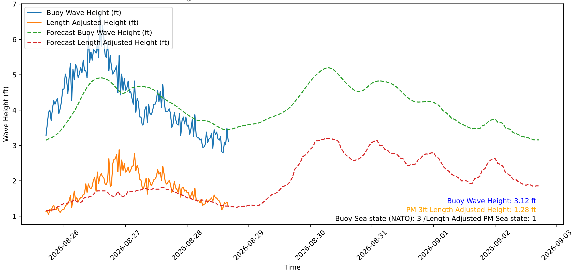
Wave Heights over Time for Oceanside Harbor at 2026-08-28 16:50:29
