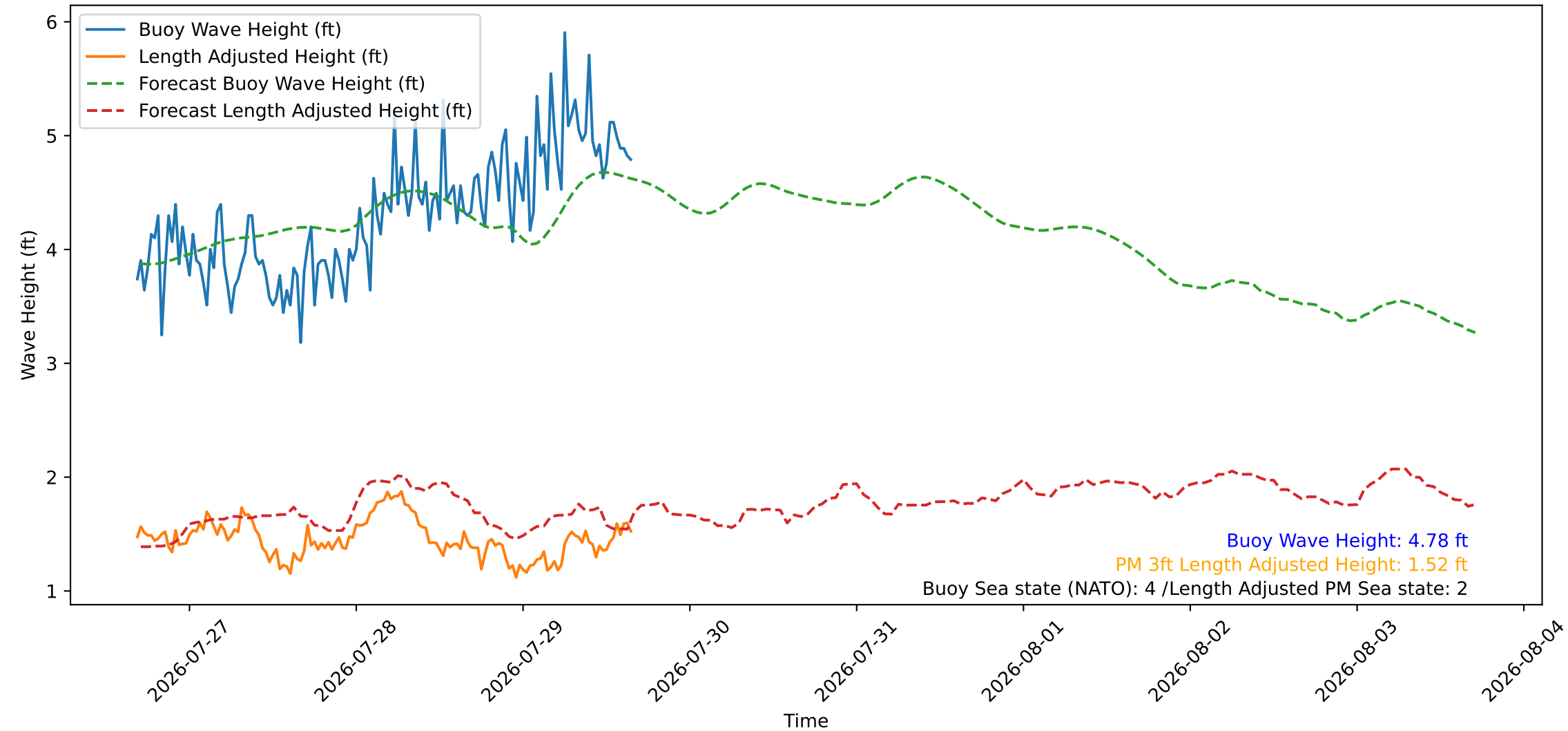
Wave Heights over Time for Oceanside Harbor at 2026-07-29 16:40:26
