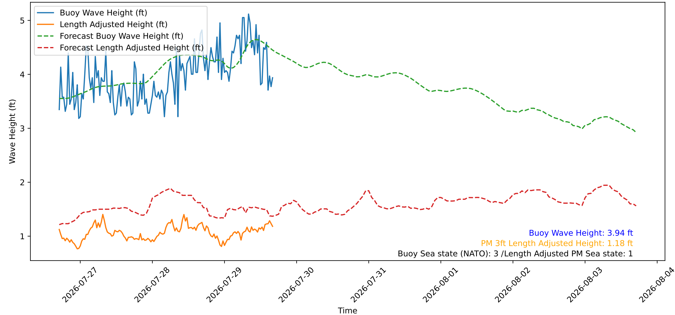
Wave Heights over Time for Red Beach at 2026-07-29 16:40:46
