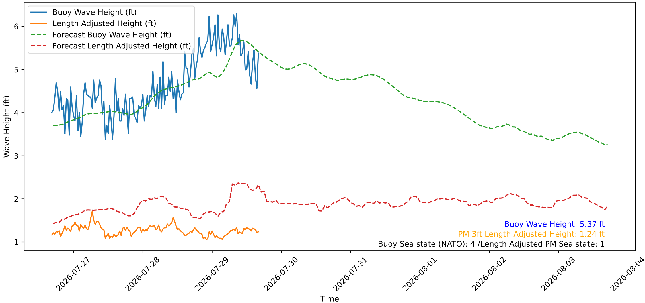
Wave Heights over Time for Green Beach at 2026-07-29 16:41:08
