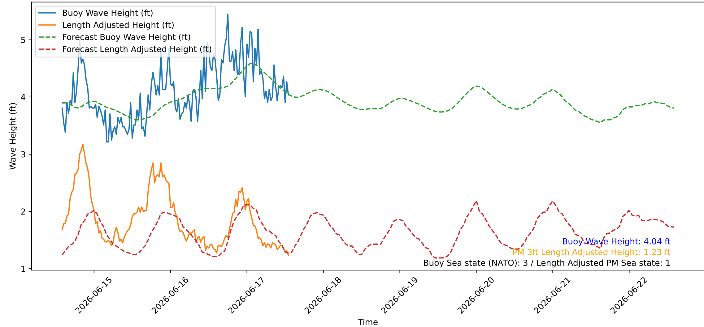
Wave Heights over Time for Oceanside Harbor at 2026-06-17 13:50:26
