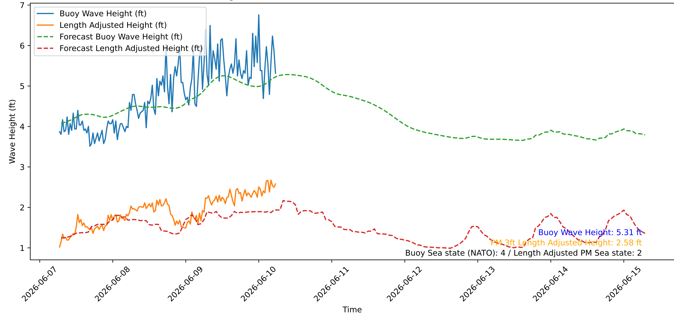
Wave Heights over Time for Oceanside Harbor at 2026-06-10 06:30:26
