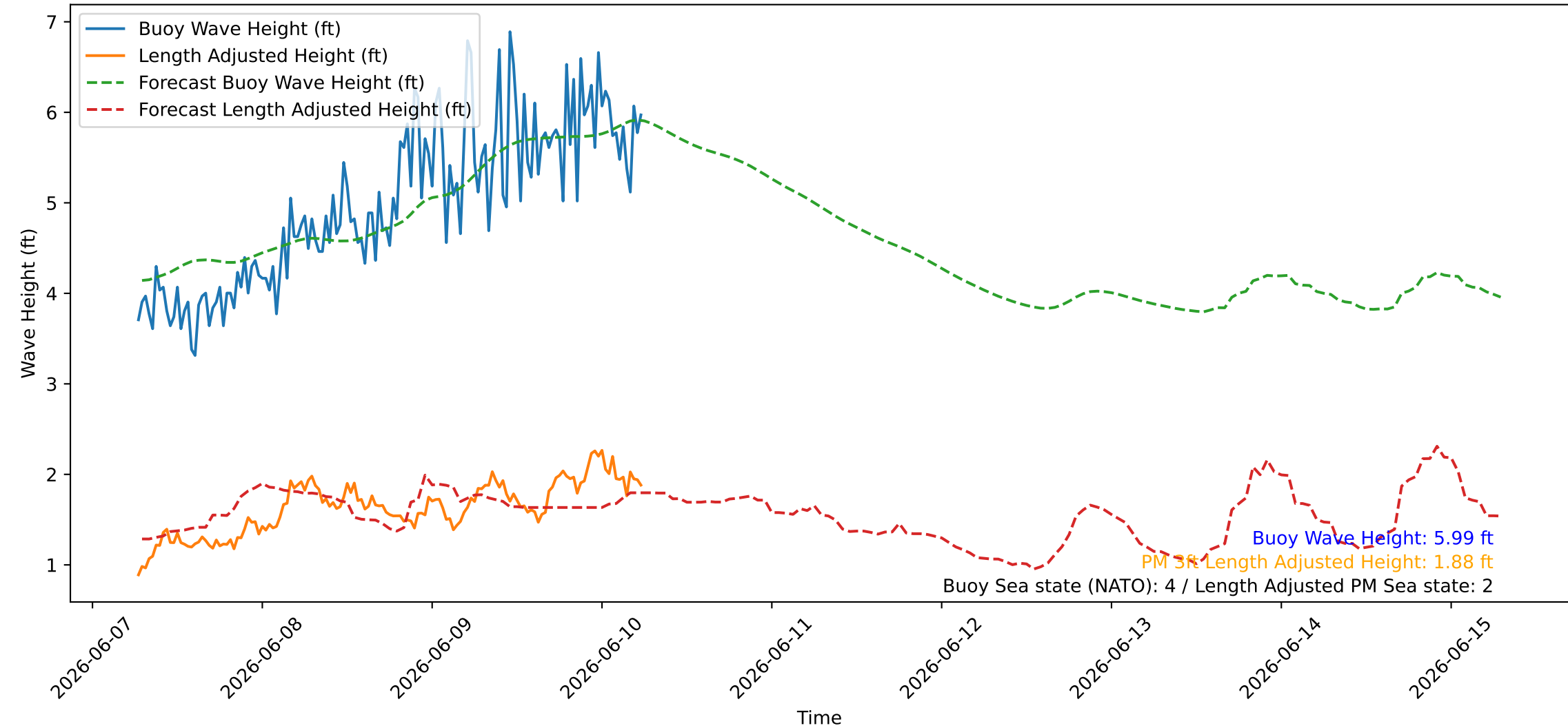
Wave Heights over Time for Green Beach at 2026-06-10 06:31:10
