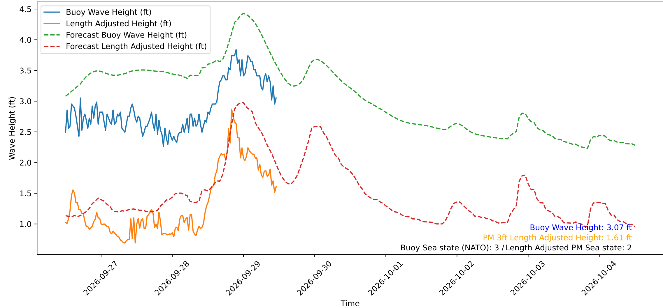
Wave Heights over Time for Red Beach at 2026-09-29 11:40:49
