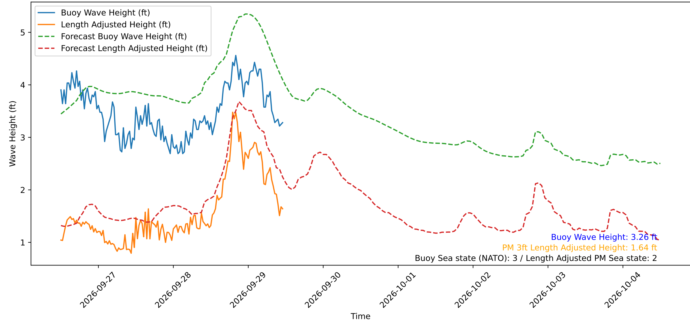
Wave Heights over Time for Green Beach at 2026-09-29 11:41:12
