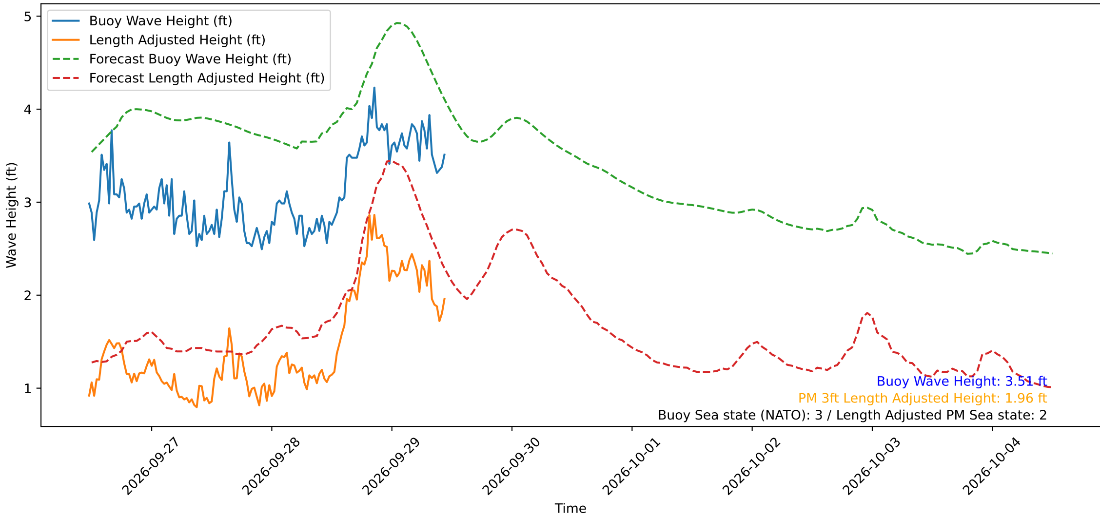
Wave Heights over Time for Oceanside Harbor at 2026-09-29 11:40:30
