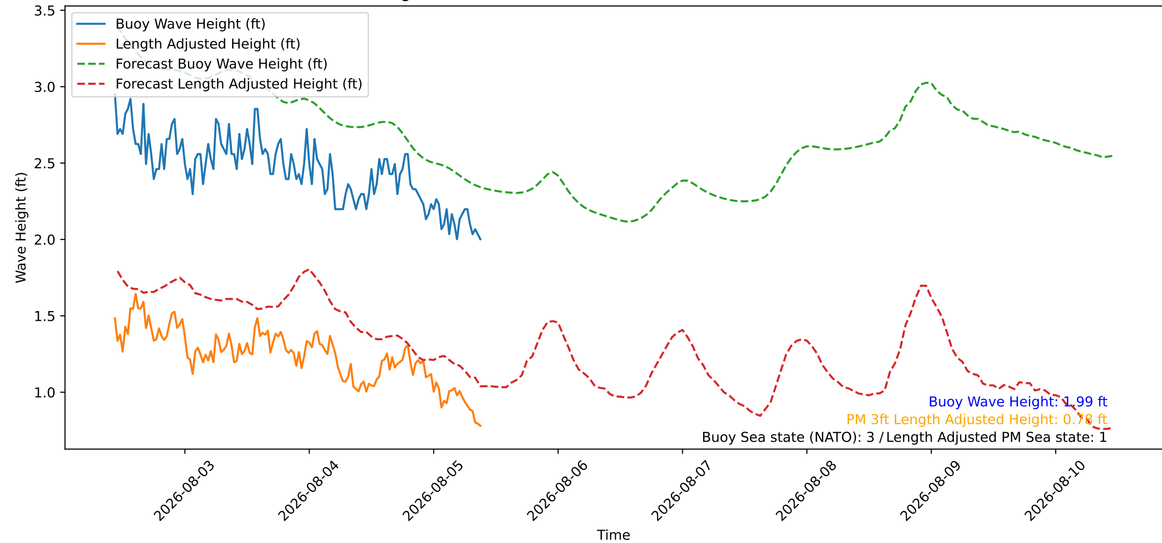
Wave Heights over Time for Oceanside Harbor at 2026-08-05 10:30:26
