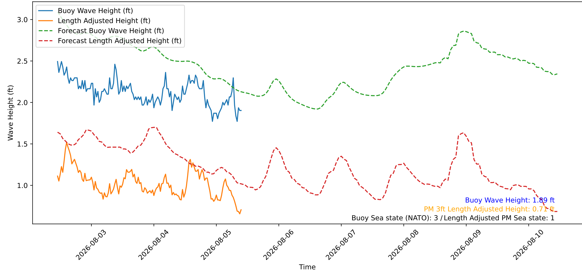
Wave Heights over Time for Red Beach at 2026-08-05 10:30:45
