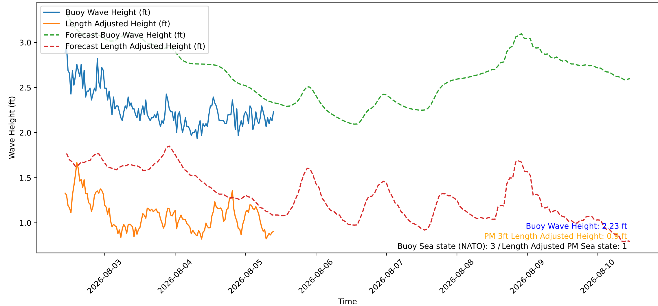
Wave Heights over Time for Green Beach at 2026-08-05 10:31:08
