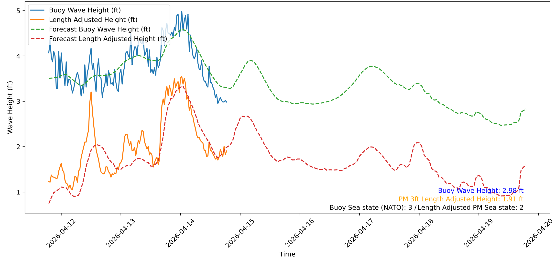
Wave Heights over Time for Green Beach at 2026-04-14 19:11:13
