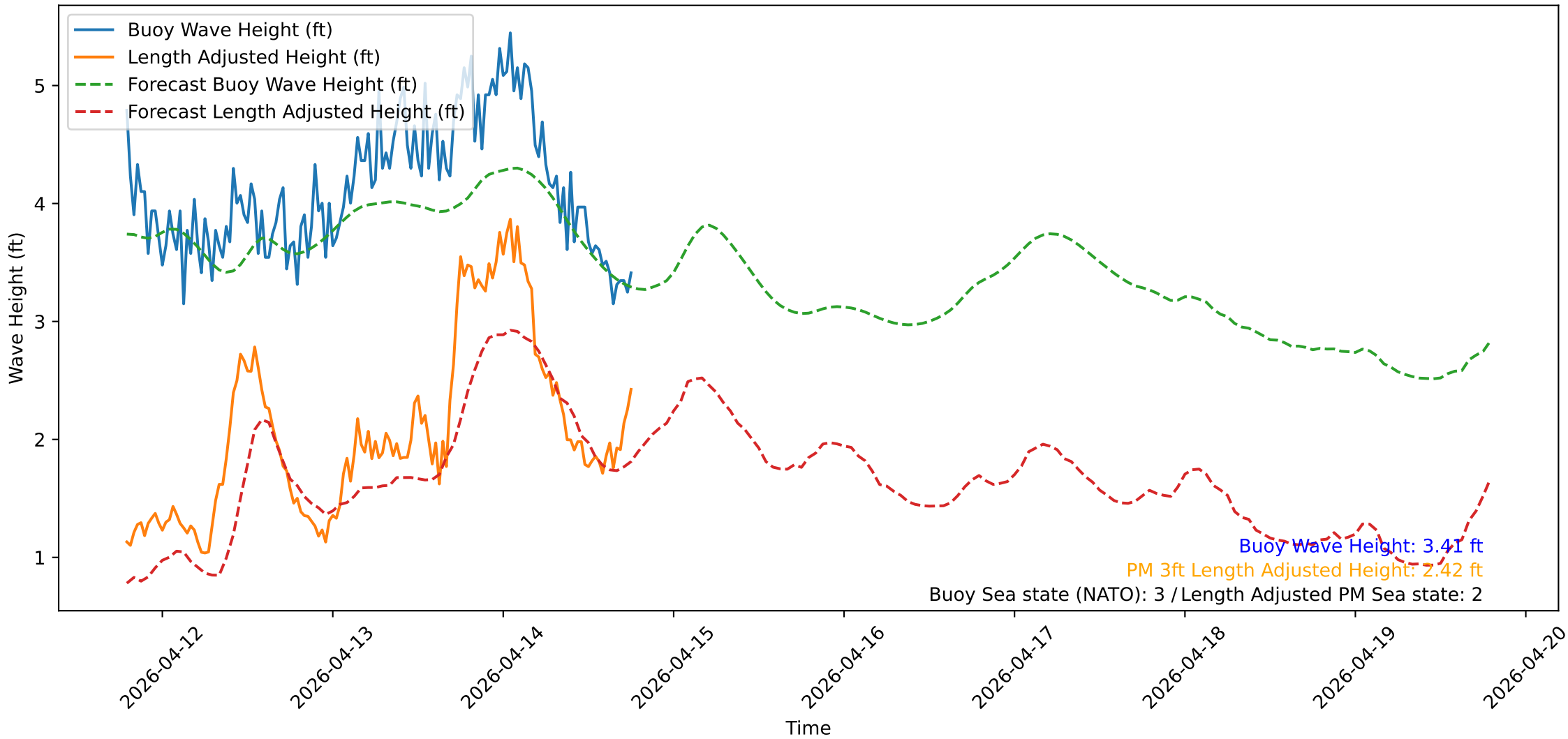
Wave Heights over Time for Oceanside Harbor at 2026-04-14 19:10:31
