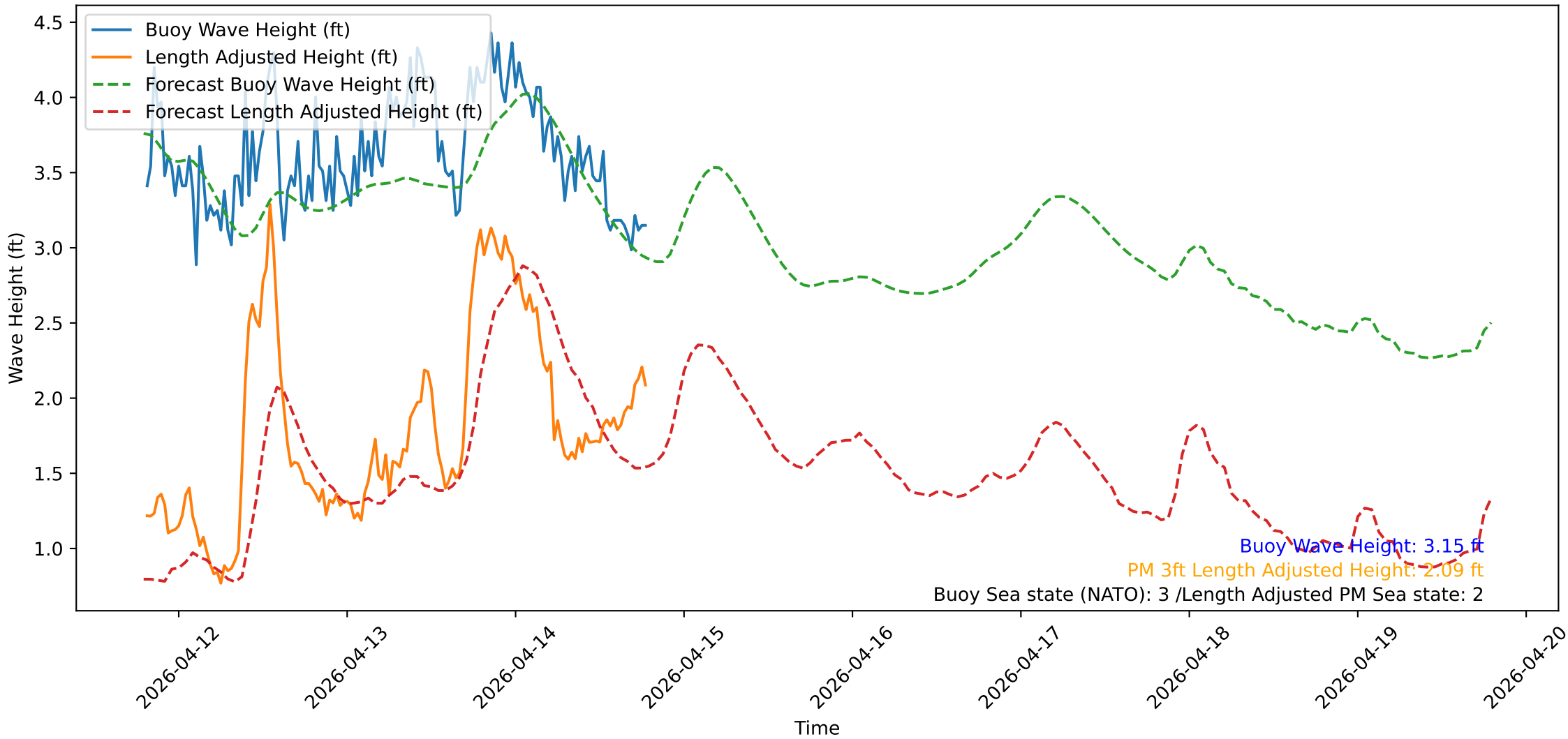
Wave Heights over Time for Red Beach at 2026-04-14 19:10:50
