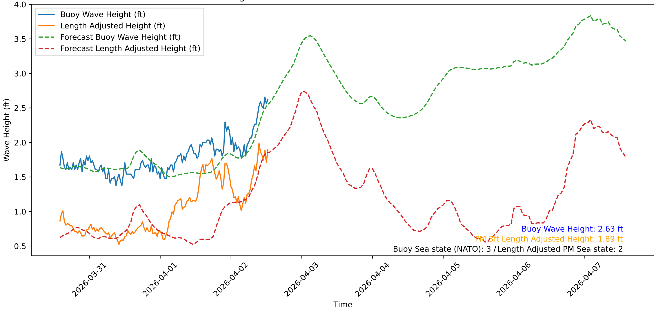
Wave Heights over Time for Red Beach at 2026-04-02 13:30:48
