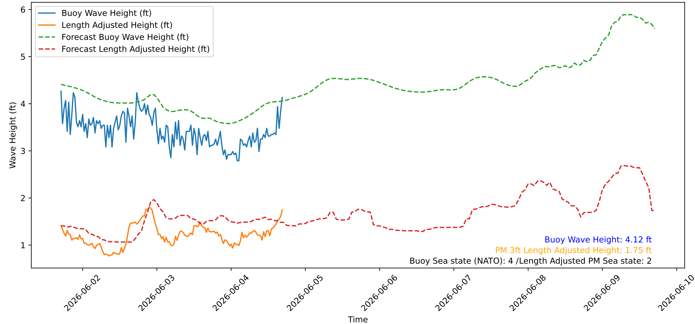
Wave Heights over Time for Green Beach at 2026-06-04 17:11:07
