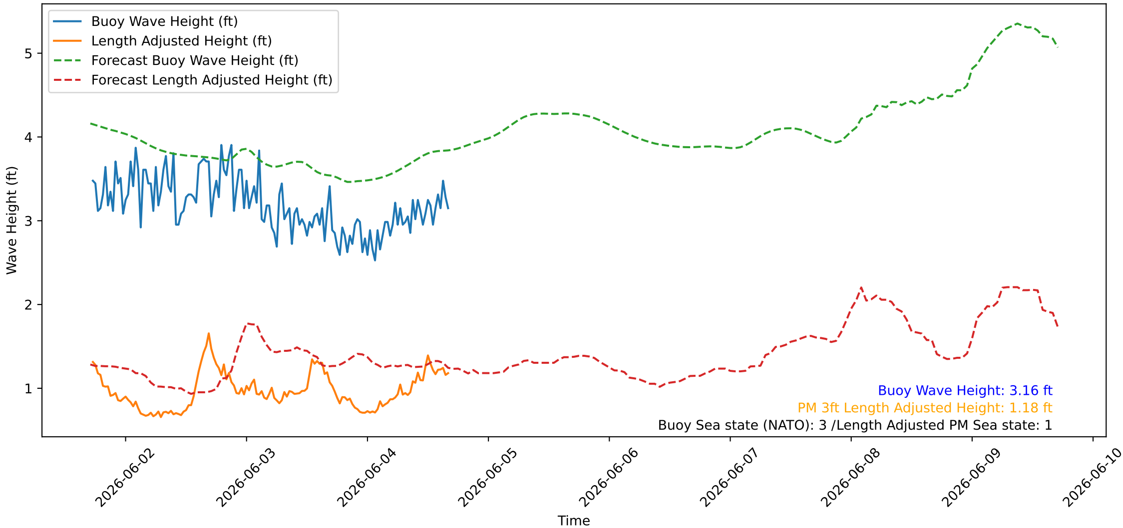
Wave Heights over Time for Red Beach at 2026-06-04 17:10:45
