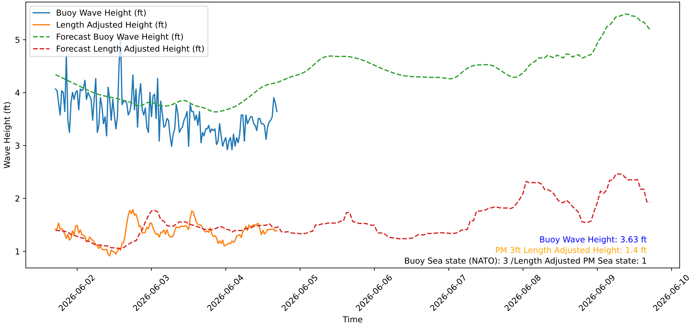
Wave Heights over Time for Oceanside Harbor at 2026-06-04 17:10:25
