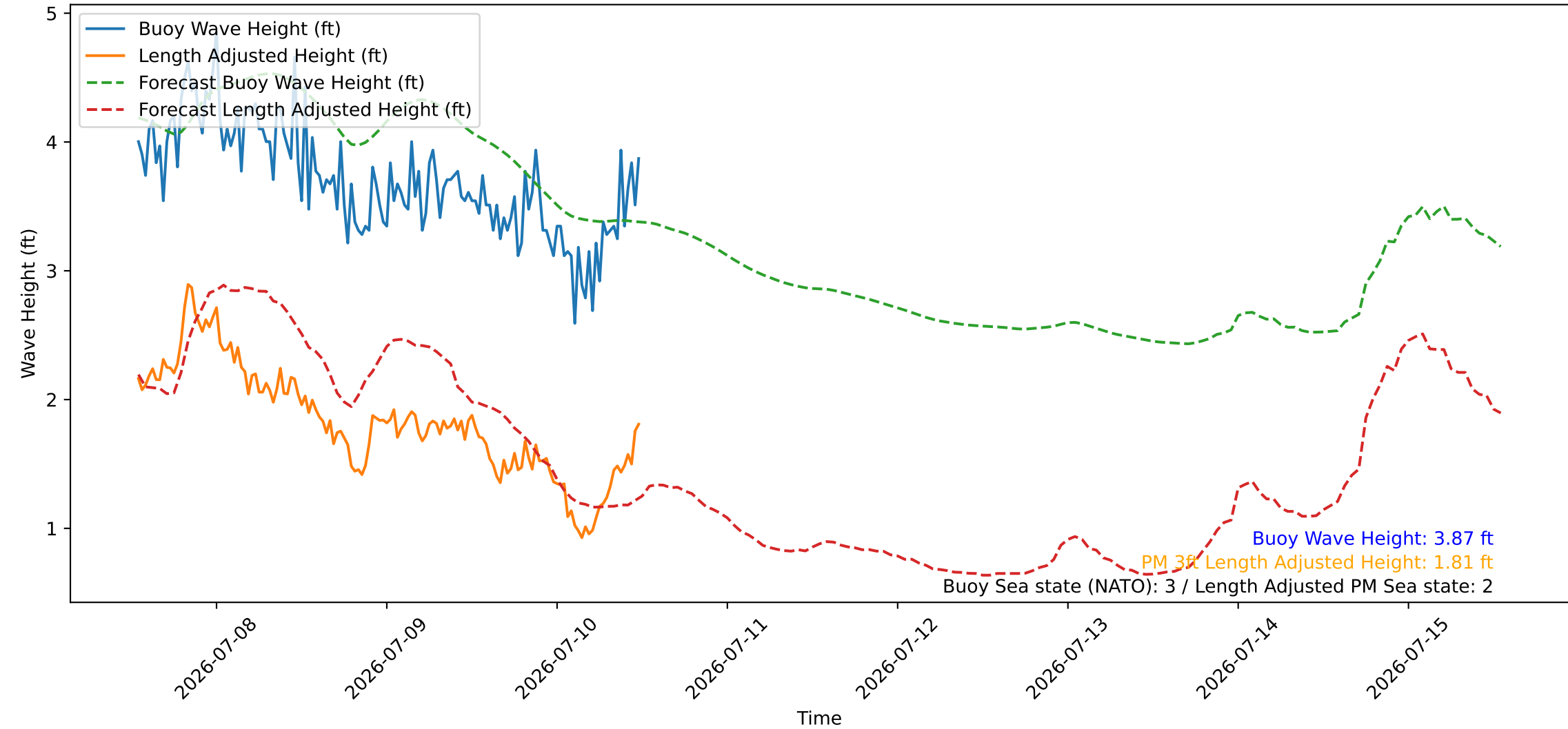
Wave Heights over Time for Red Beach at 2026-07-10 12:30:45
