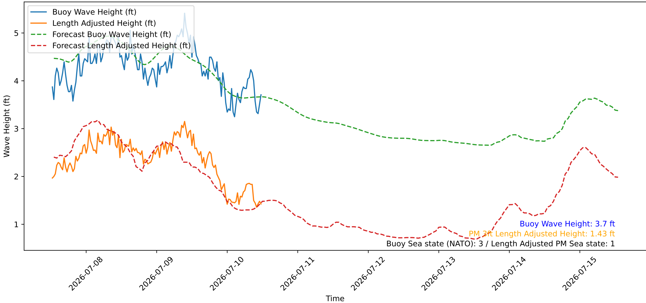
Wave Heights over Time for Oceanside Harbor at 2026-07-10 12:30:26
