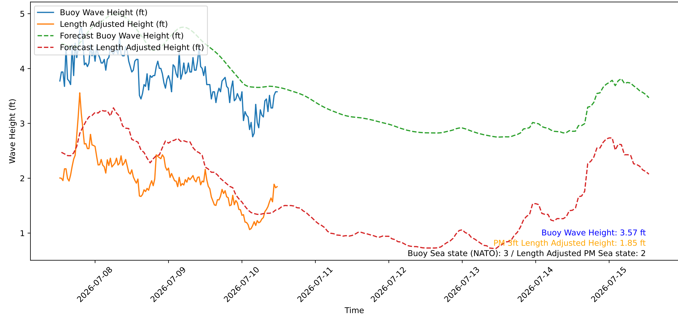
Wave Heights over Time for Green Beach at 2026-07-10 12:31:07
