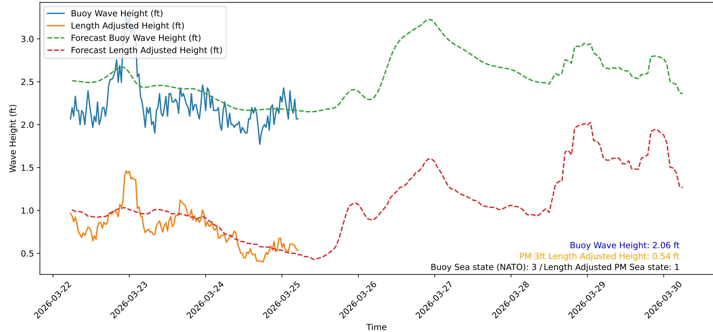
Wave Heights over Time for Green Beach at 2026-03-25 05:41:09
