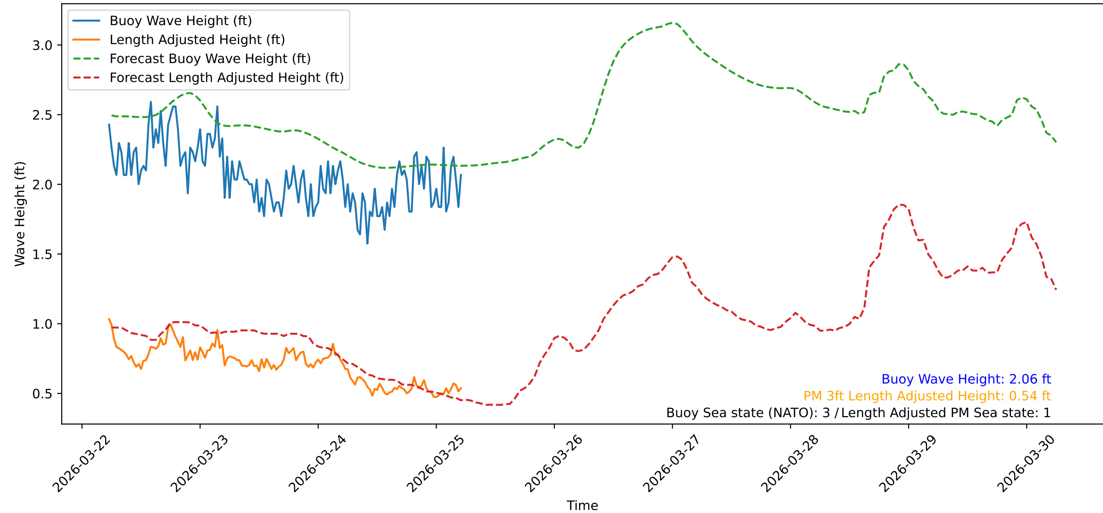
Wave Heights over Time for Oceanside Harbor at 2026-03-25 05:40:31
