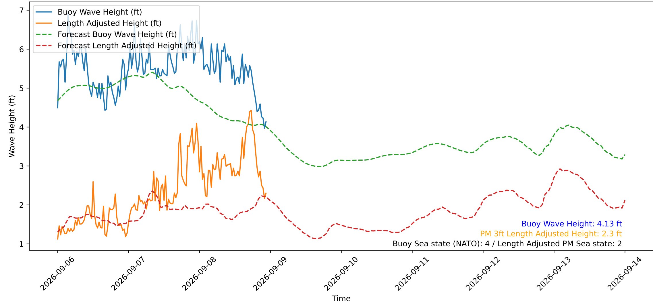
Wave Heights over Time for Red Beach at 2026-09-08 23:30:49
