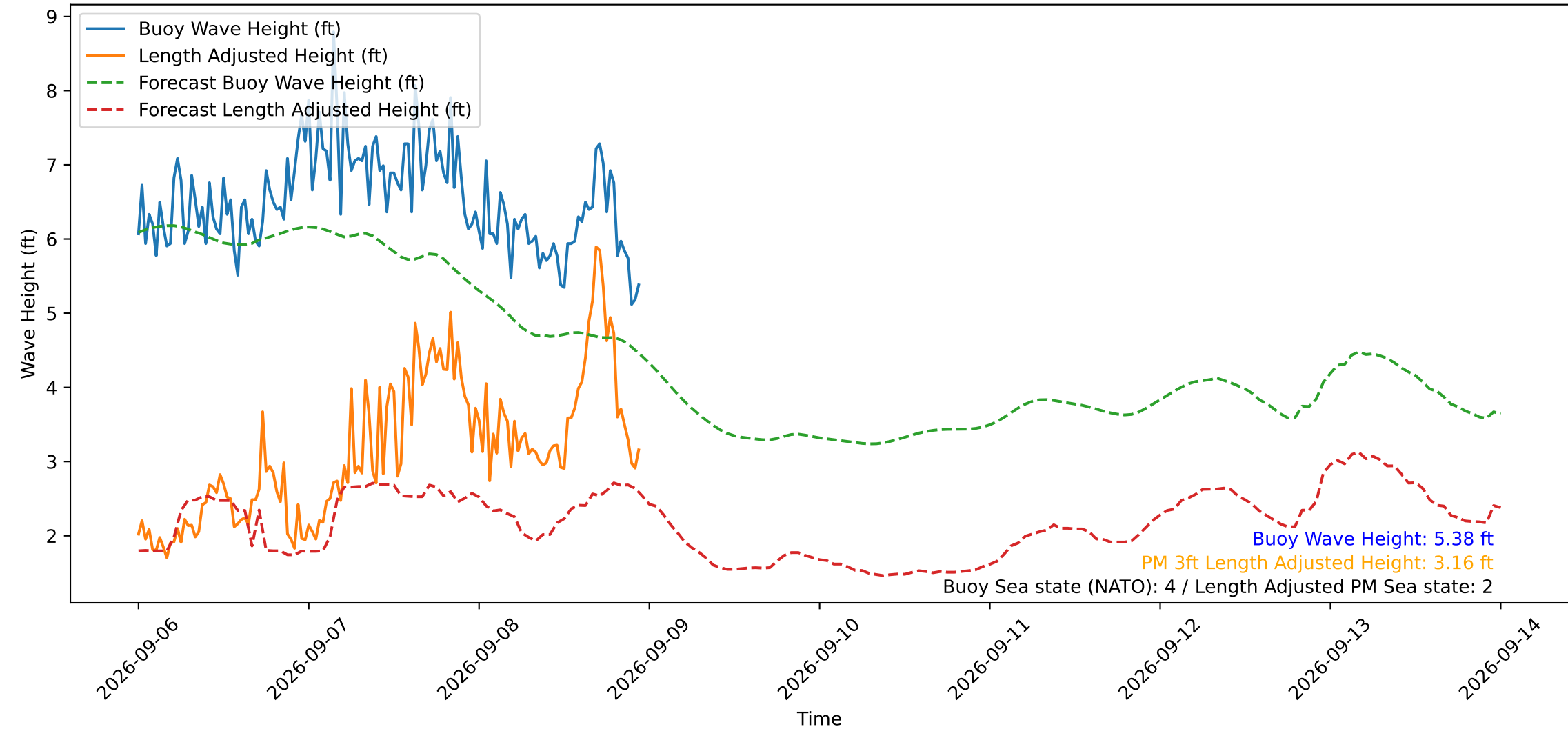
Wave Heights over Time for Green Beach at 2026-09-08 23:31:11
