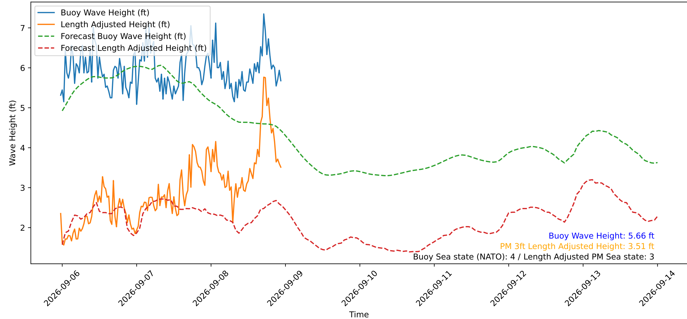
Wave Heights over Time for Oceanside Harbor at 2026-09-08 23:30:29
